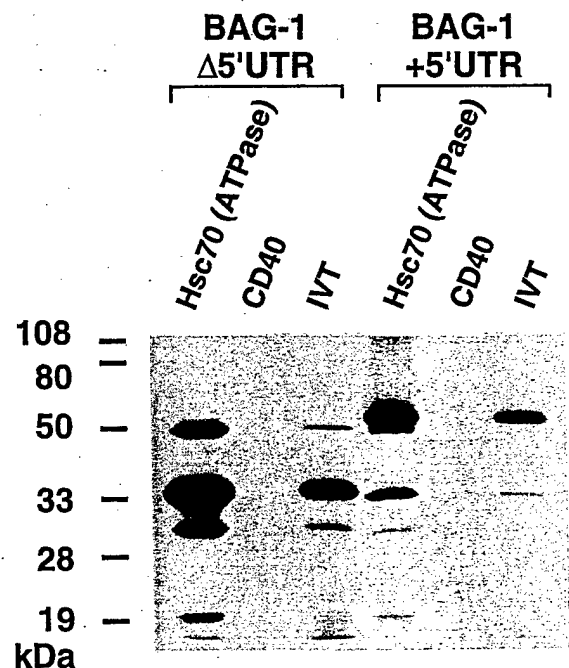
Fig. 5. Hsc70 binds to BAG-1, BAG-1L, and BAG-1M. Human BAG-1 cDNAs containing or lacking the region upstream of the originally identified ORF were in vitro translated (IVT) in the presence of [ ^{35} S]-methionine, thus producing the BAG-1, BAG-1M, and BAG-1L proteins. The BAG-1 (+5'UTR) cDNA produces primarily BAG-1L, whereas the BAG-1 ( \Delta 5'UTR) cDNA produces mostly BAG-1 along with some BAG-1M protein. IVT BAG-1 proteins were incubated with GST-Hsc70 (ATP-binding domain) or (as a negative control) GST-CD40 cytosolic domain immobilized on glutathione-Sepharose. After washing, proteins bound to beads were analyzed by SDS-PAGE/autoradiography. As a control, one-tenth the input volume of the IVT proteins was run directly in gels. Note that BAG-1, BAG-1M, and BAG-1L bind to GST-Hsc70 but not to GST-CD40. The small molecular weight proteins presumably represent partial degradation products of BAG-1 or translation initiation from internal AUG codons. These small proteins have not been detected in vivo , arising only in IVT experiments.
