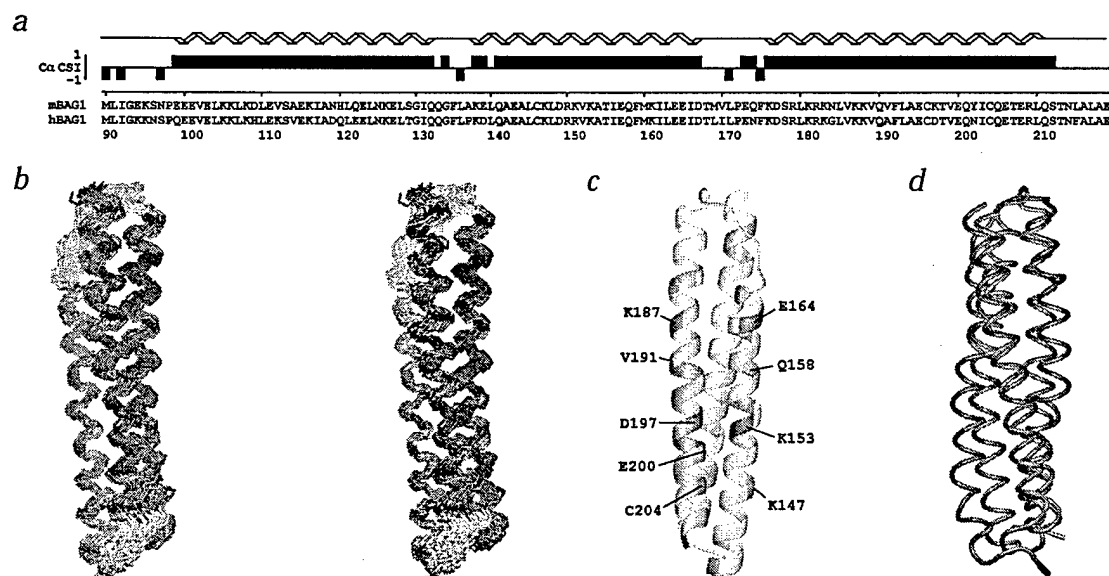
Fig. 1 C-terminal region of BAG1 is a three-helix bundle. a , \alpha chemical shift index 23 (CSI) of residues 90-219 of murine BAG1 (mBAG1). The sequence of the murine BAG1 fragment used in this study is indicated to scale below the CSI data and aligned with human BAG1L. The \alpha -helices are defined schematically at the top of the figure. b , Stereo image of superimposed backbone traces of a family of 25 final structures of BAG1 residues 99-210. The first helix ( \alpha 1 ) is colored blue, the second one ( \alpha 2 ) green and the third one ( \alpha 3 ) orange; the connecting loops are white. The images were generated with the program MOLMOL 24 . c , Ribbon representation of BAG1 residues 99-210 colored according to ^1\text{H} - and ^{15}\text{N} -chemical shift changes of the individual residues upon binding of Hsc70 peptide (Asn 256-Cys 267). The color intensity is proportional to the change. Gray indicates residues for which no data are available. Some of the residues with the most pronounced changes are labeled. The model depicted here is rotated 180° relative to the orientation in (b). d , Comparison of BAG1 with syntaxin (view as in (a)). Tube models of the \alpha atoms of residues 101-212 of BAG1 (orange) and residues 27-146 of syntaxin (blue; PDB code 1BR0) 25 are superimposed. Note the similar configuration of helices in these two antiparallel three-helix bundles.
