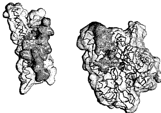
Fig. 3 Contact regions of the BAG1–Hsc70 ATPase complex. The proteins are represented by red C \alpha traces and transparent surfaces of BAG1 on the left and Hsc70 ATPase domain 15 on the right. An ADP molecule that binds in the cleft between the two lobes of the ATPase domain is shown in red as van der Waals spheres. The complex has been 'opened up' by a 180° rotation of BAG1 to reveal the contact surfaces predicted from mutagenesis and molecular docking. The sites of mutation that abolish binding are colored yellow and adjacent contact sites suggested from molecular docking are colored cyan. This image was produced with the program SPOCK 35 .
