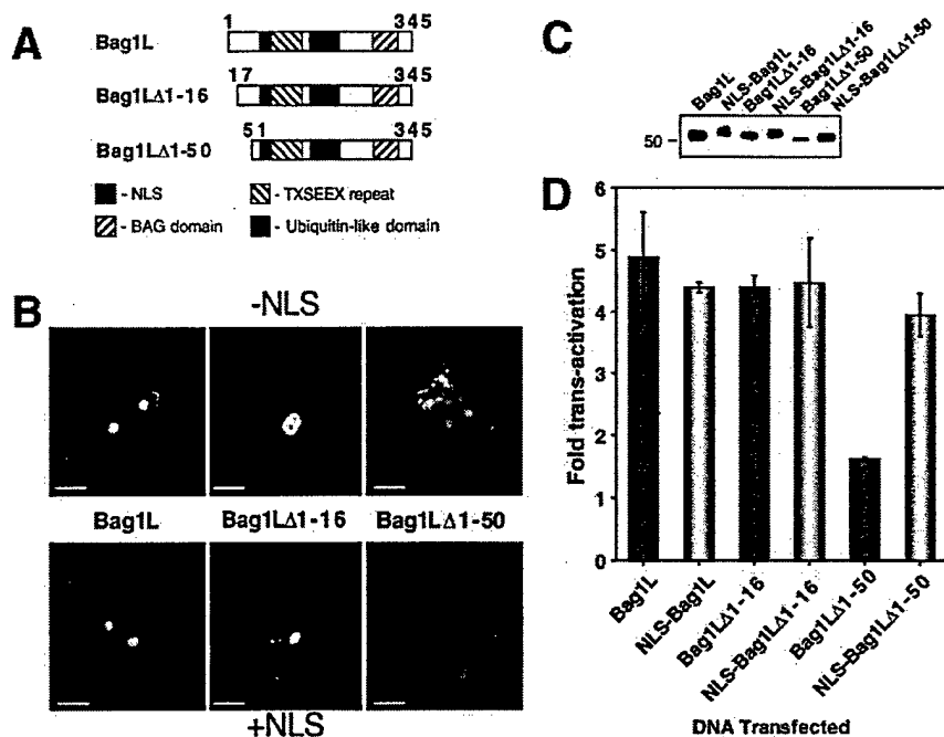
FIG. 4. The NH 2 terminus of Bag1L is required for its targeting/retention in the nucleus. A, a schematic is presented showing deletion mutants of Bag1L, which are lacking the NH 2 -terminal 16 (Bag1LΔ1-16) or 50 amino acids (Bag1LΔ1-50). B, COS-7 cells were transfected with the following Bag1 expression plasmids: pcDNA3-Bag1L, pcDNA3-Bag1LΔ1-16, pcDNA3-Bag1LΔ1-50, pcDNA3-NLS-Bag1L, pcDNA3-NLS-Bag1LΔ1-16, or pcDNA3-NLS-Bag1LΔ1-50. At 30 h post-transfection, cells were fixed, stained, and examined by laser confocal microscopy. C, COS-7 cells were transfected as in A, and after 30 h the cells were lysed in radioimmune precipitation buffer. Cell extracts (25 μg of total protein) were subjected to SDS-PAGE/immunoblot assay and probed with an antibody to Bag1. D, COS-7 cells were transfected with 0.06 μg of pSG5-AR, 0.5 μg of pLCI, 0.04 μg of pCMV-β-galactosidase, and various amounts of the Bag1 expression plasmids used in B. Total DNA was maintained at 1.1 μg by the addition of pcDNA3 control plasmid. At 30 h after transfection, cells were stimulated with 1 nM R1881. Cell extracts were prepared and assayed for CAT and β-galactosidase activity at 40 h after transfection (mean ± S.E., n = 2).
