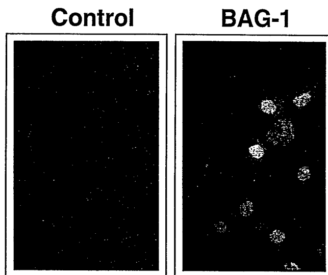
Fig. 7. Confocal immunofluorescence analysis of intracellular distribution of BAG-1 proteins demonstrates nuclear location. Rat-1a cells, which had been stably transfected with a huBAG-1 cDNA (encompassing nucleotides –390 to 880 bp relative to the AUG), were analyzed for huBAG-1 protein expression by immunofluorescence assay. After fixation, cells were incubated with either a mlgG1 control (left) or the anti-huBAG-1 monoclonal antibody KS-6C8, followed by a FITC-conjugated secondary antibody.
