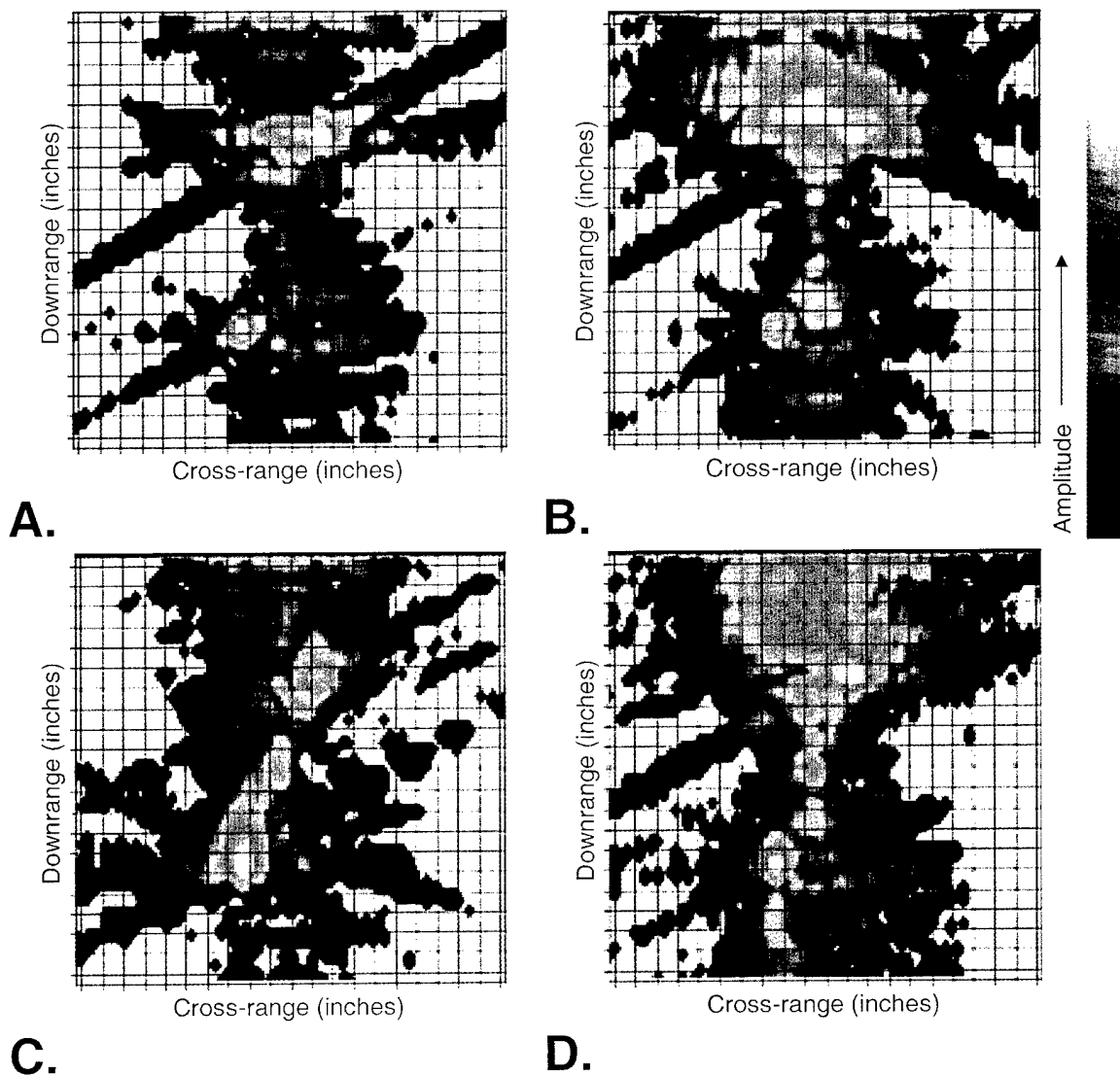
Figure 17. Inverse synthetic aperture radar (ISAR) images for targets at 70^\circ off broadside. (a) PEC plate. (b) Dielectric plate. (c) HIGP with vias. (d) HIGP with no vias.
