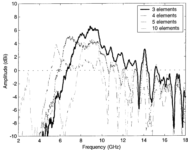
Figure 38. Copper tape monopoles coupling elements of narrowband HIGP with no vias. Broadside frequency responses.
