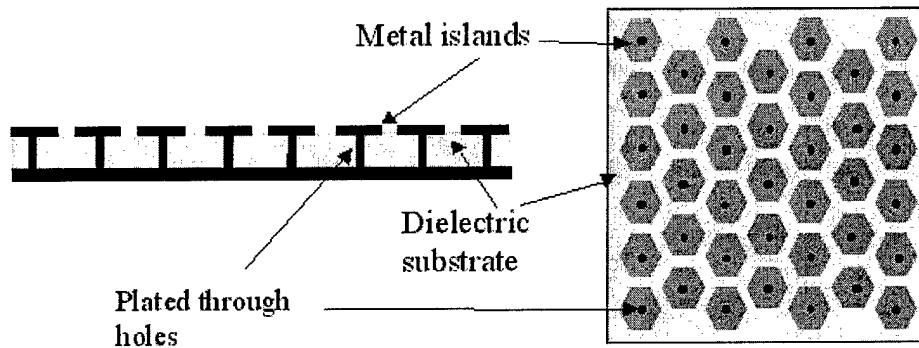
Figure 5. "Thumbtack" high-impedance ground plane [9].
