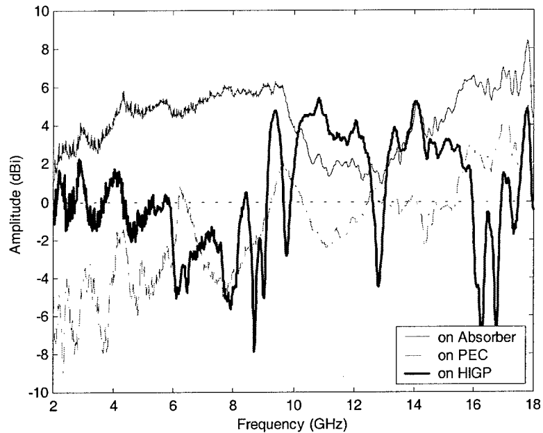
Figure 27. Thin foil log-periodic zigzag antenna mounted on absorber filled cavity, on PEC plate, and on narrowband HIGP. Broadside frequency sweeps.
