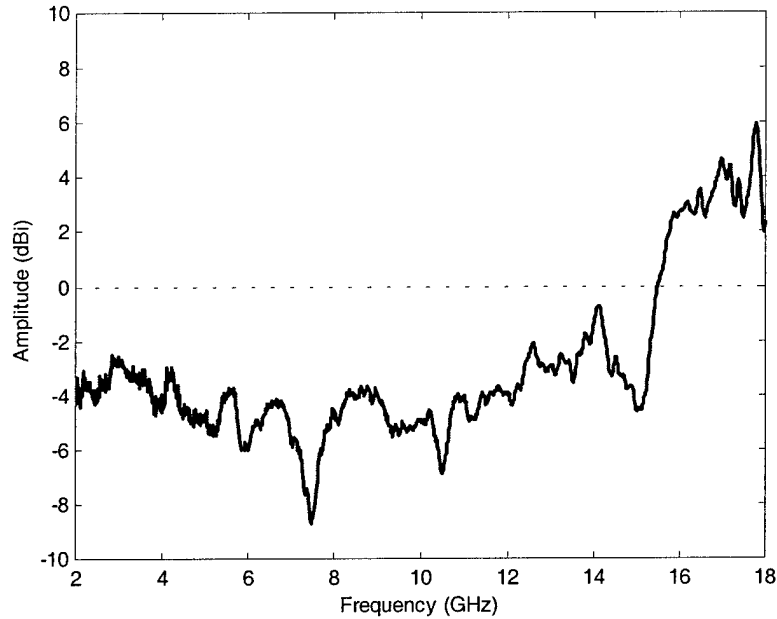
Figure 35. Thin foil log-periodic zigzag antenna mounted on spatially varying broadband HIGP. Broadside frequency sweep.
