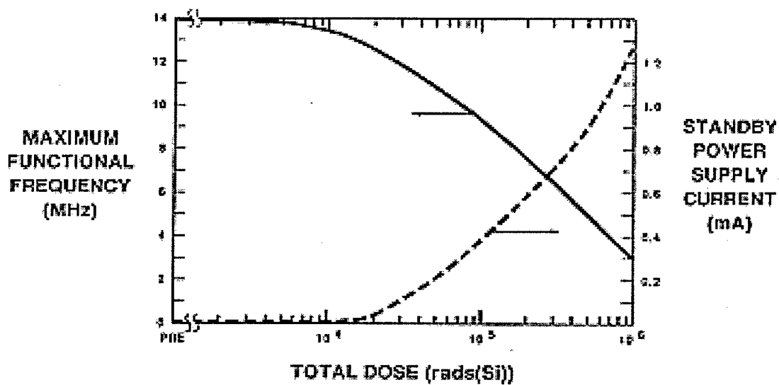
Figure 2-7. Microprocessor Trend for Operating Frequency and Standby Current versus Total Ionizing Dose [18]
