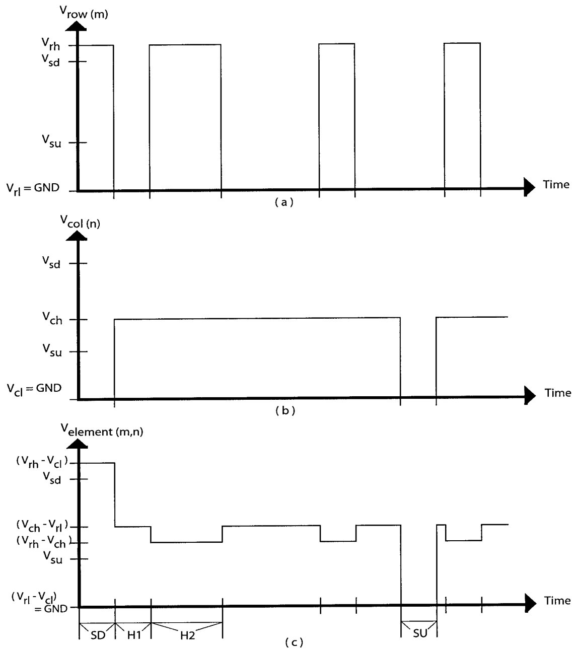
Figure 4-2. Example PWM signals for enhanced bi-stable operation.
