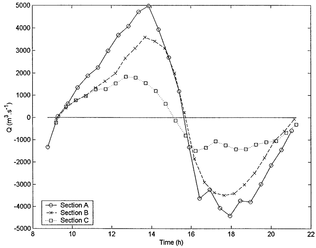
Figure 4-13. Cross-sectional discharge through Main Inlet.
