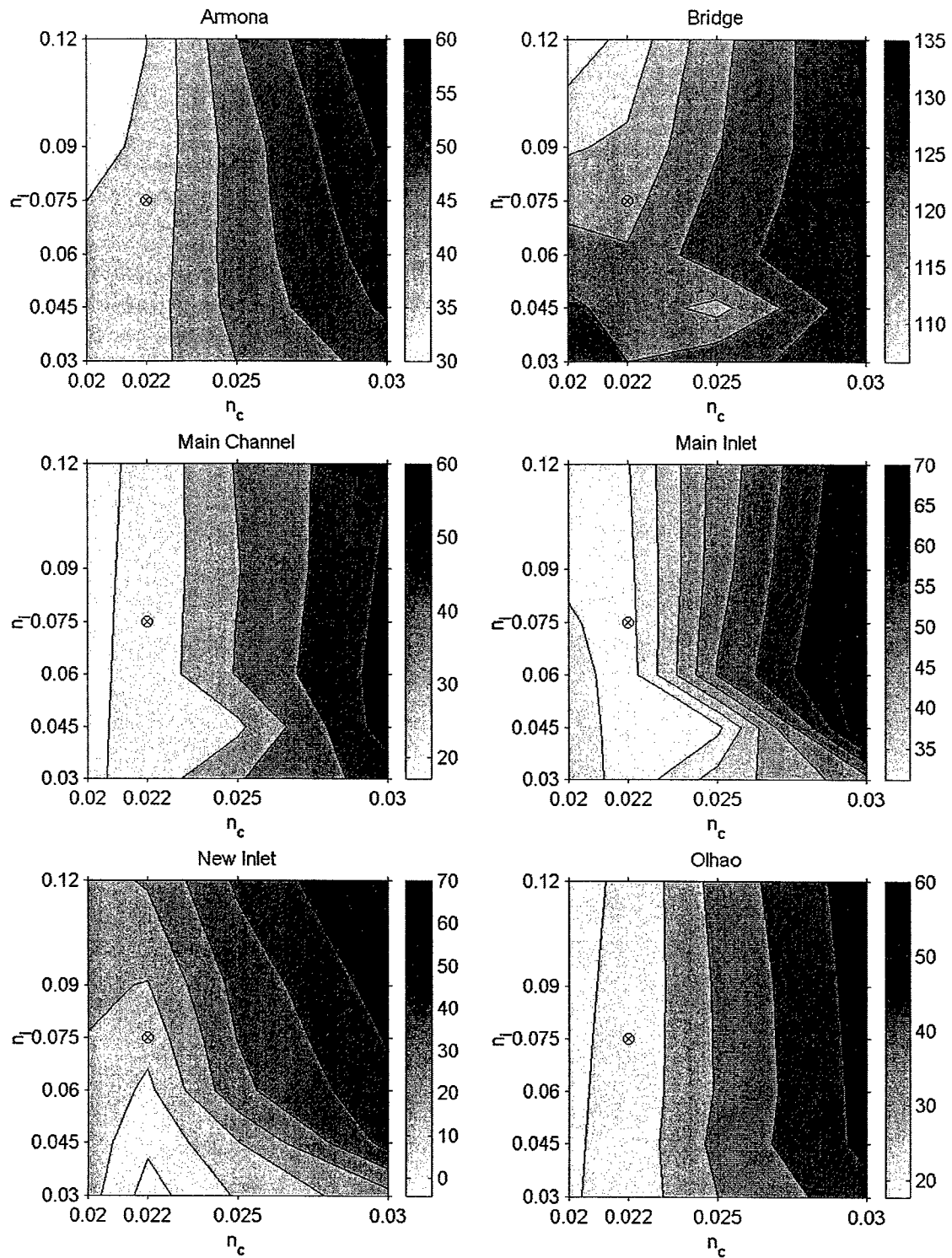
Figure 5-32. Friction Coefficient Calibration: M_4 phase difference (degrees) between model results and measurements (the circled cross corresponds to the friction coefficients chosen for the simulations).
