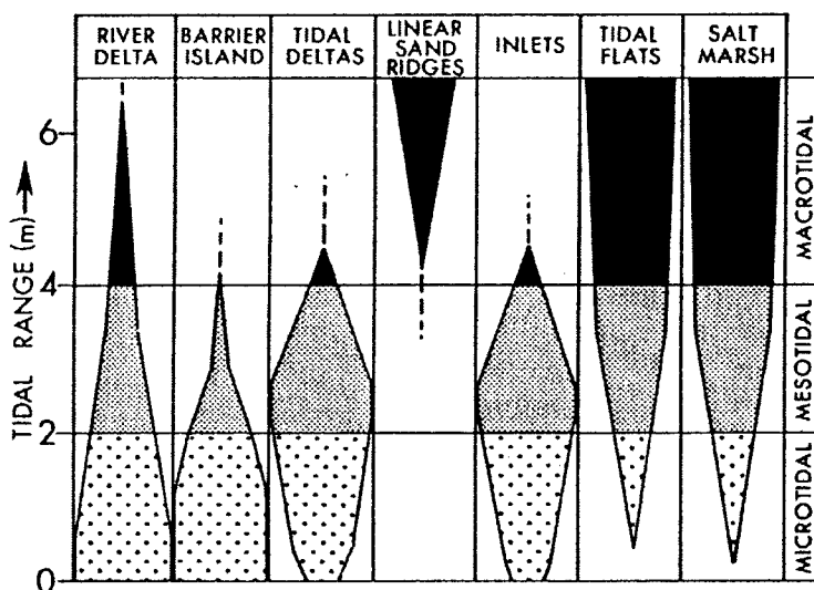
Figure 3-3. Variation of morphology of coastal plain shorelines with respect to mean tidal range (from Hayes, 1979).
