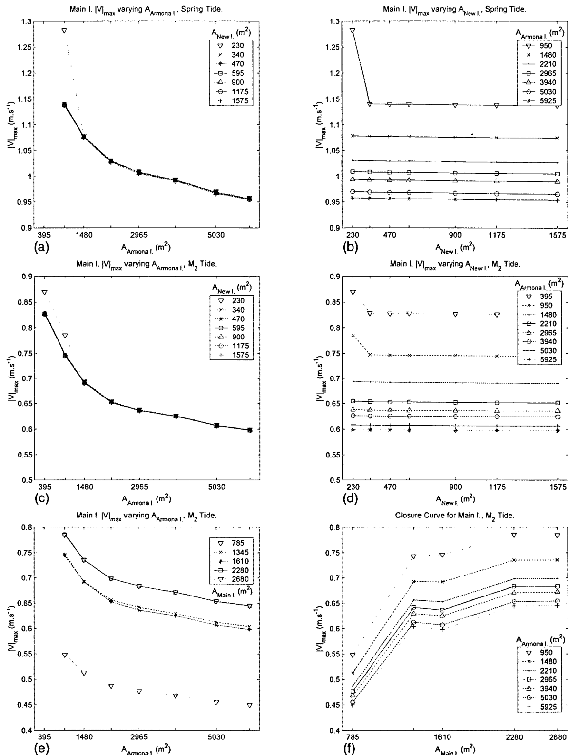
Figure 5-25. Maximum Velocities through Main Inlet. Spring tidal forcing, varying A_{\text{Armona}} and A_{\text{New}} (a and b); M_2 forcing varying A_{\text{Armona}} and A_{\text{New}} (c and d), and varying A_{\text{Armona}} and A_{\text{Main}} (e and f). For a, b, c, and d: A_{\text{Main I}}=1,610 m 2 . For e and f, A_{\text{New I}}=595 m 2 . All the plots are at the same scale.
