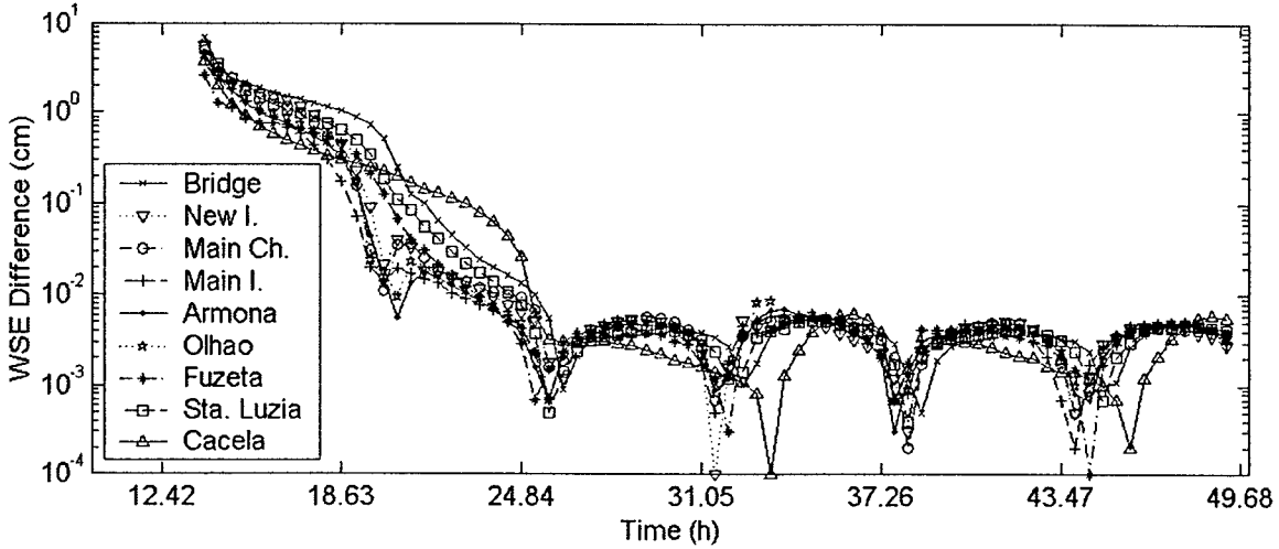
Figure 5-5. Water surface elevation difference between modeled and measured values at the 9 stations shown in Figure 5-4.
