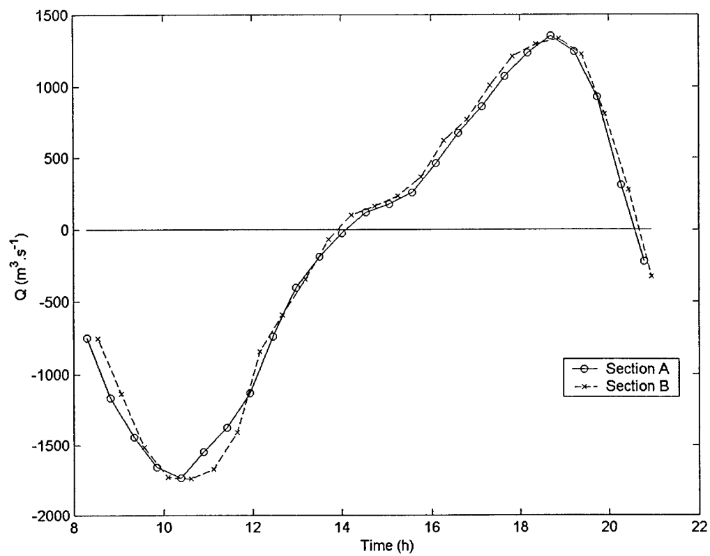
Figure 4-16. Cross-sectional discharge through Armona Inlet.
