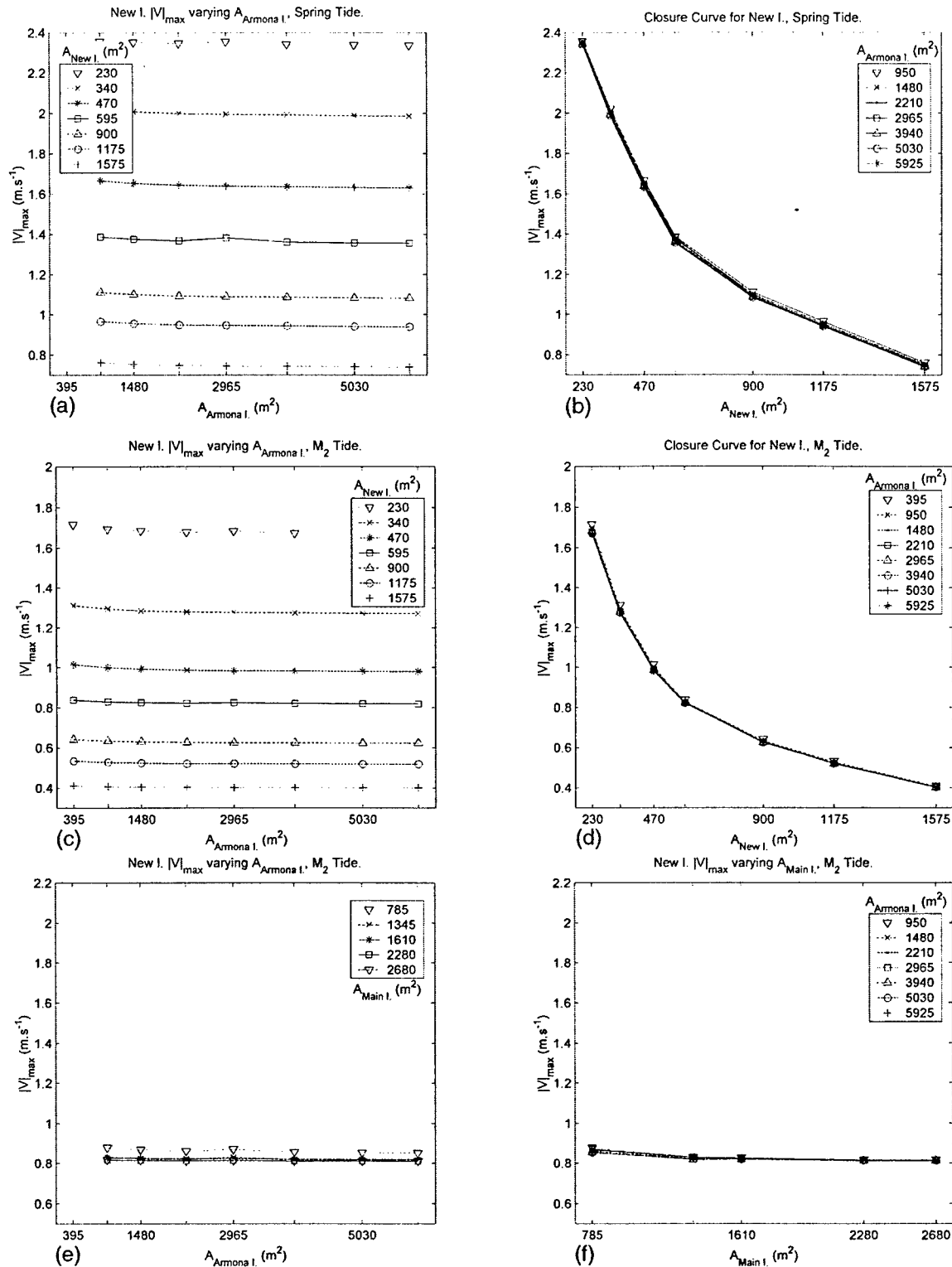
Figure 5-22. Maximum Velocities through New Inlet. Spring tidal forcing, varying A_{\text{Armona}} and A_{\text{New}} (a and b); M_2 forcing varying A_{\text{Armona}} and A_{\text{New}} (c and d), and varying A_{\text{Armona}} and A_{\text{Main}} (e and f). For a, b, c, and d: A_{\text{Main}}=1,610 \text{ m}^2 . For e and f, A_{\text{New}}=595 \text{ m}^2 . All the plots are at the same scale.
