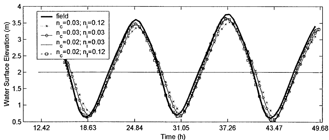
Figure 5-10. Field and modeled (selected runs) water surface elevation at “Main Channel” station (the offshore MSL is +2.00m).
