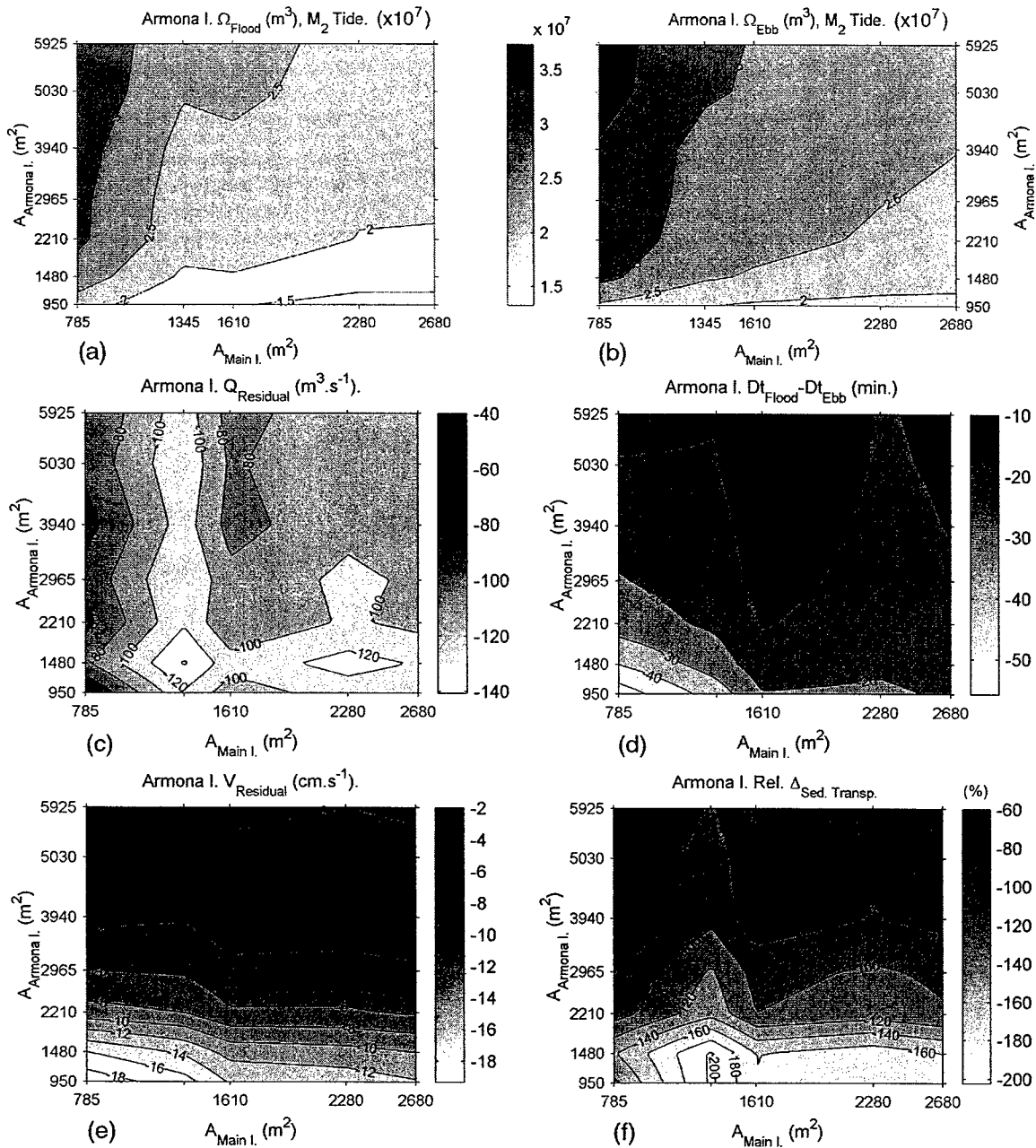
Figure 5-18. Results at Armona Inlet from simulations with M_2 forcing, varying A_{\text{Armona}} and A_{\text{Main}} ( A_{\text{New}}=595 \text{ m}^2 ). Flood and ebb tidal prisms (a and b); Residual discharge (c); Difference between flood and ebb durations (d); Residual current (e); and flood – ebb near-bed sediment transport difference, relative to the flood sediment transport (f).
