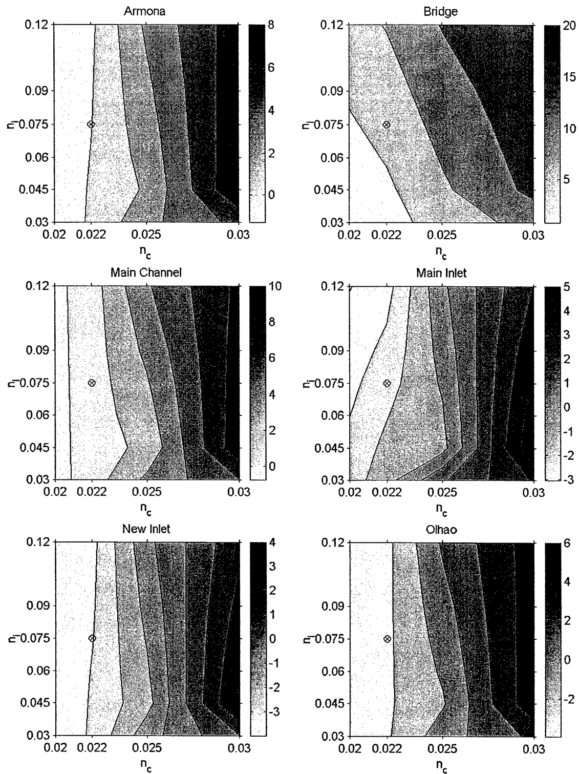
Figure 5-30. Friction Coefficient Calibration: M_2 phase difference (degrees) between model results and measurements (the circled cross corresponds to the friction coefficients chosen for the simulations).
