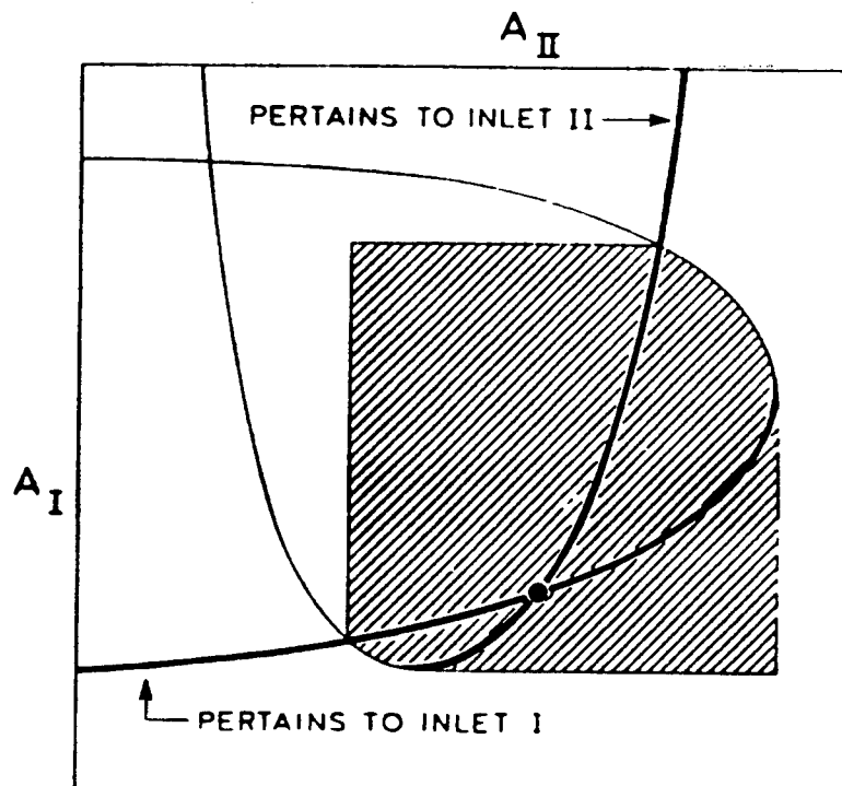
Figure 2-4. Equilibrium Flow Curves for Inlets I and II (adapted from van de Kreeke, 1985)
