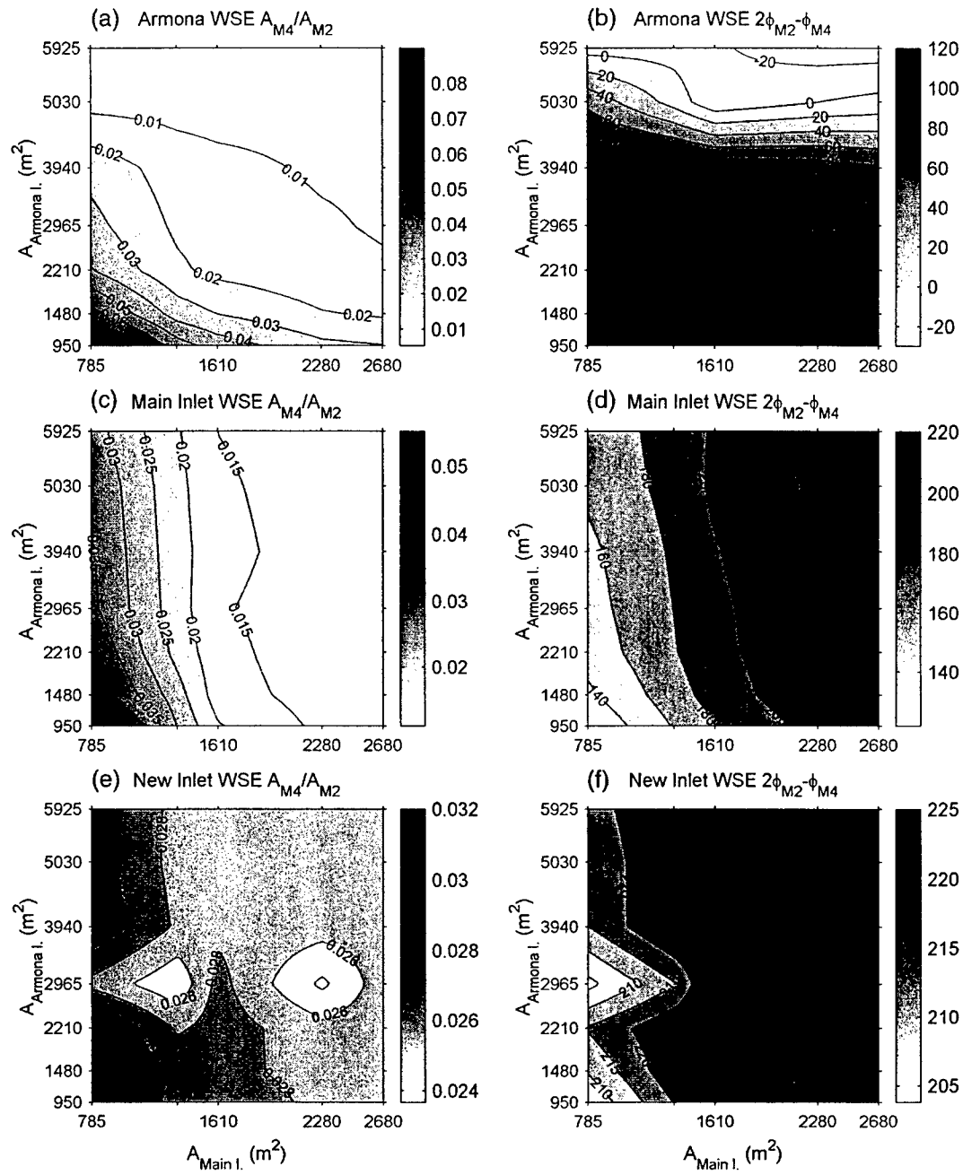
Figure 5-47. M_4 to M_2 water surface amplitude ratio and phase of M_4 relative to M_2 at Armona Inlet, Main Inlet, and New Inlet. Simulations using M_2 forcing, varying A_{\text{Armona}} and A_{\text{Main}} ( A_{\text{New}}=595 \text{ m}^2 ).
