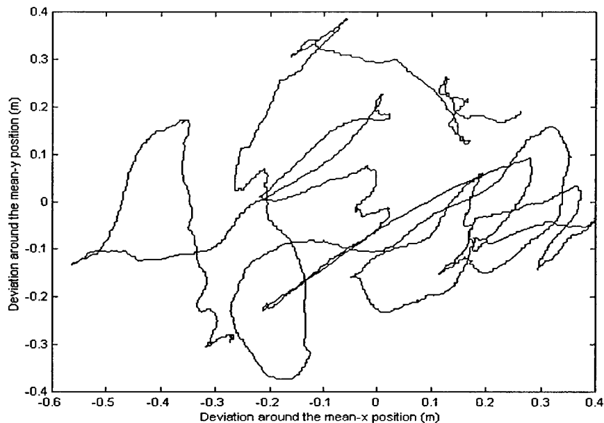
Figure 4-1. DGPS Test results.
