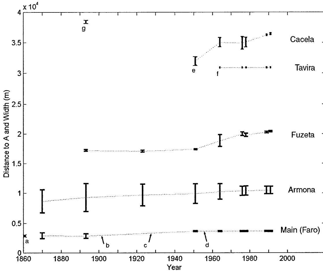
Figure 3-26 Eastern inlet evolution. Width (represented by the bars, and with the scale shown in the y-axis), and position with respect to baseline origin, point A (see Figure 3-20). Notes: a, opening of Bispo Inlet; b, virtual closure of Bispo Inlet; c, artificial opening of Main (Faro) Inlet; d, conclusion of Main Inlet stabilization; e, natural Cochicho Inlet; f, stabilized Tavira Inlet; g, Cacela Inlet at the end of the lagoon (no shore-attached barrier present).
