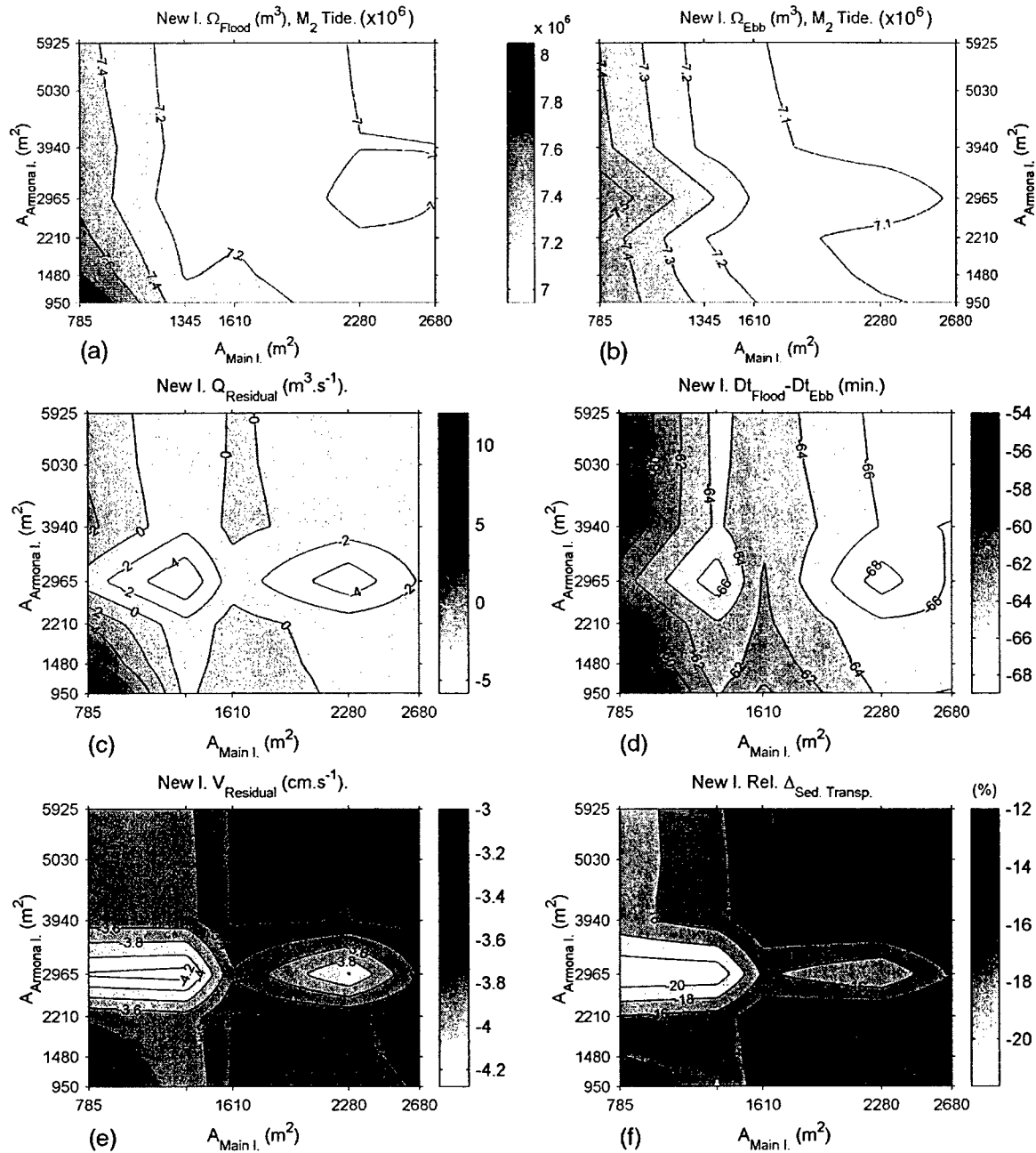
Figure 5-13. Results at New Inlet from simulations with M_2 forcing, varying A_{Armona} and A_{Main} ( A_{New}=595 m^2 ). Flood and ebb tidal prisms (a and b); Residual discharge (c); Difference between flood and ebb durations (d); Residual current (e); and flood – ebb near-bed sediment transport difference, relative to the flood sediment transport (f).
