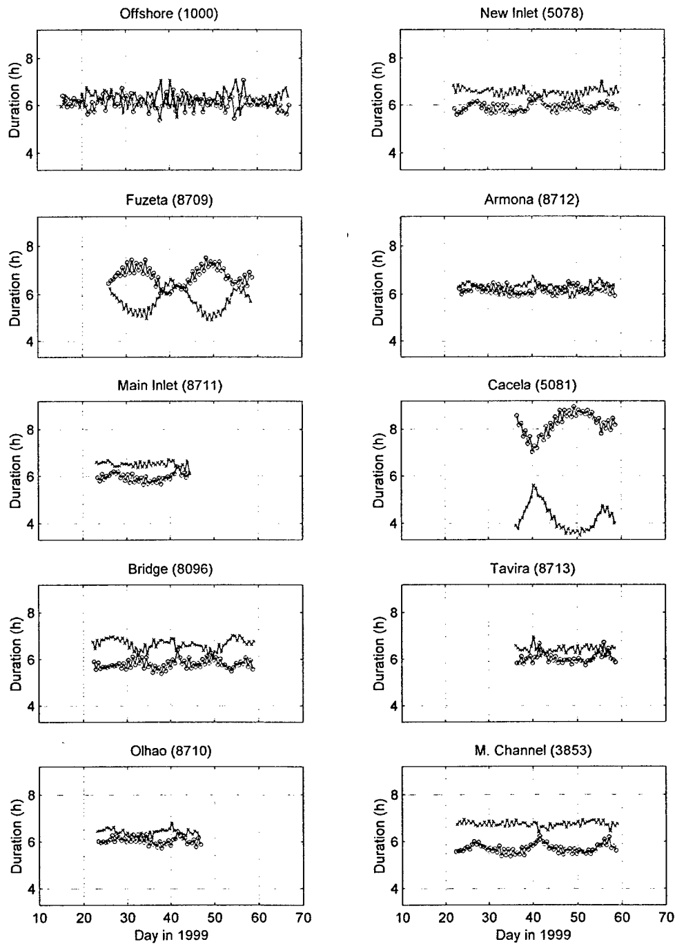
Figure 4-7. Flood ( crosses ) and Ebb ( circles ) durations for each station (determined from the water surface elevation fluctuations).
