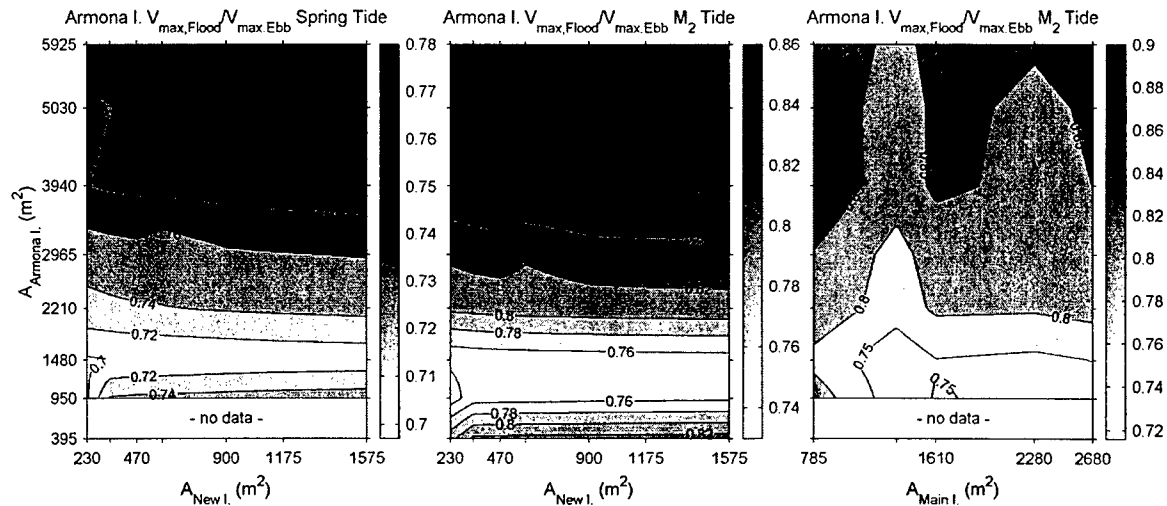
Figure 5-28. Flood / Ebb Armona Inlet maximum velocity ratio. Spring forcing varying A_{Armona} and A_{NewI} (a); M_2 forcing varying A_{Armona} and A_{NewI} (b), and A_{Armona} and A_{MainI} (c).
