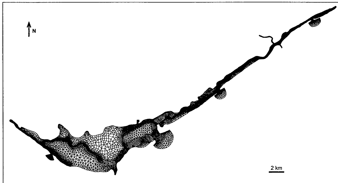
Figure 5-2 Computational mesh of Ría Formosa (12,800 elements).
