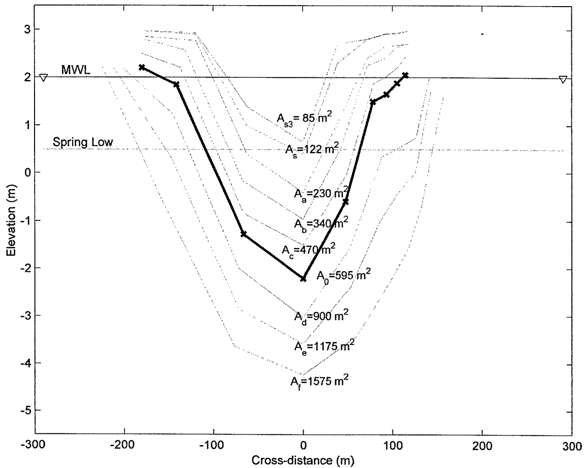
Figure 5-40. New Inlet cross-sectional areas used in the simulations.
