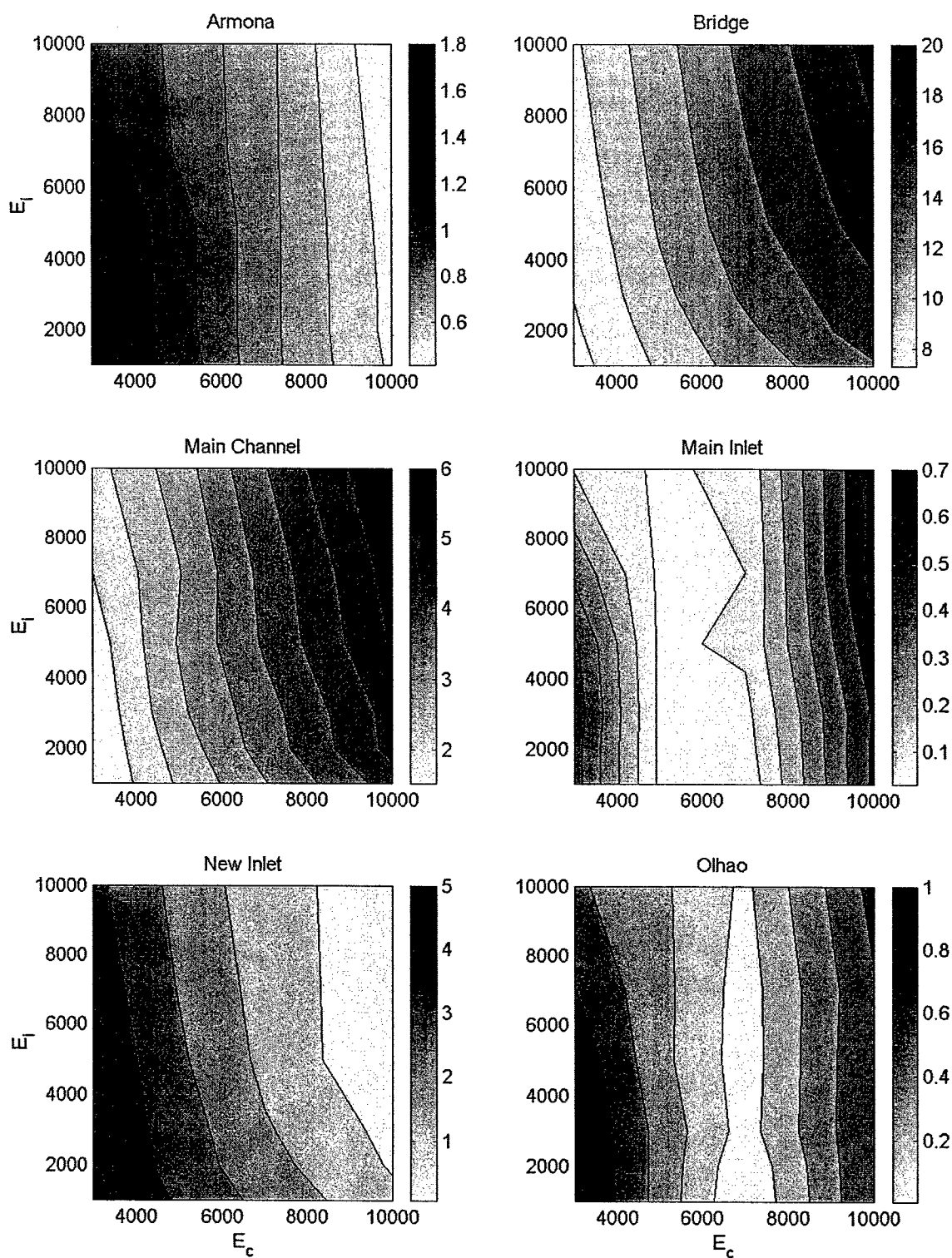
Figure 5-34. Eddy Viscosity Calibration: M_2 amplitude absolute difference (cm) between model results and measurements.
