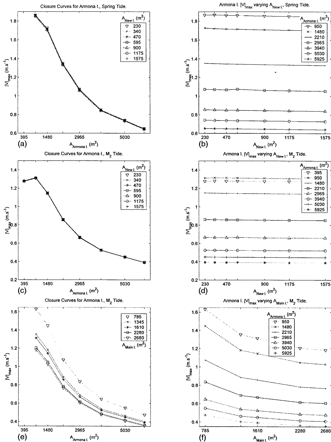
Figure 5-27. Maximum Velocities through Armona Inlet. Spring tidal forcing, varying A_{\text{Armona}} and A_{\text{New}} (a and b); M_2 forcing varying A_{\text{Armona}} and A_{\text{New}} (c and d), and varying A_{\text{Armona}} and A_{\text{Main}} (e and f). For a, b, c, and d: A_{\text{Main I.}} = 1,610 \text{ m}^2 . For e and f, A_{\text{New I.}} = 595 \text{ m}^2 . All the plots are on the same scale.
