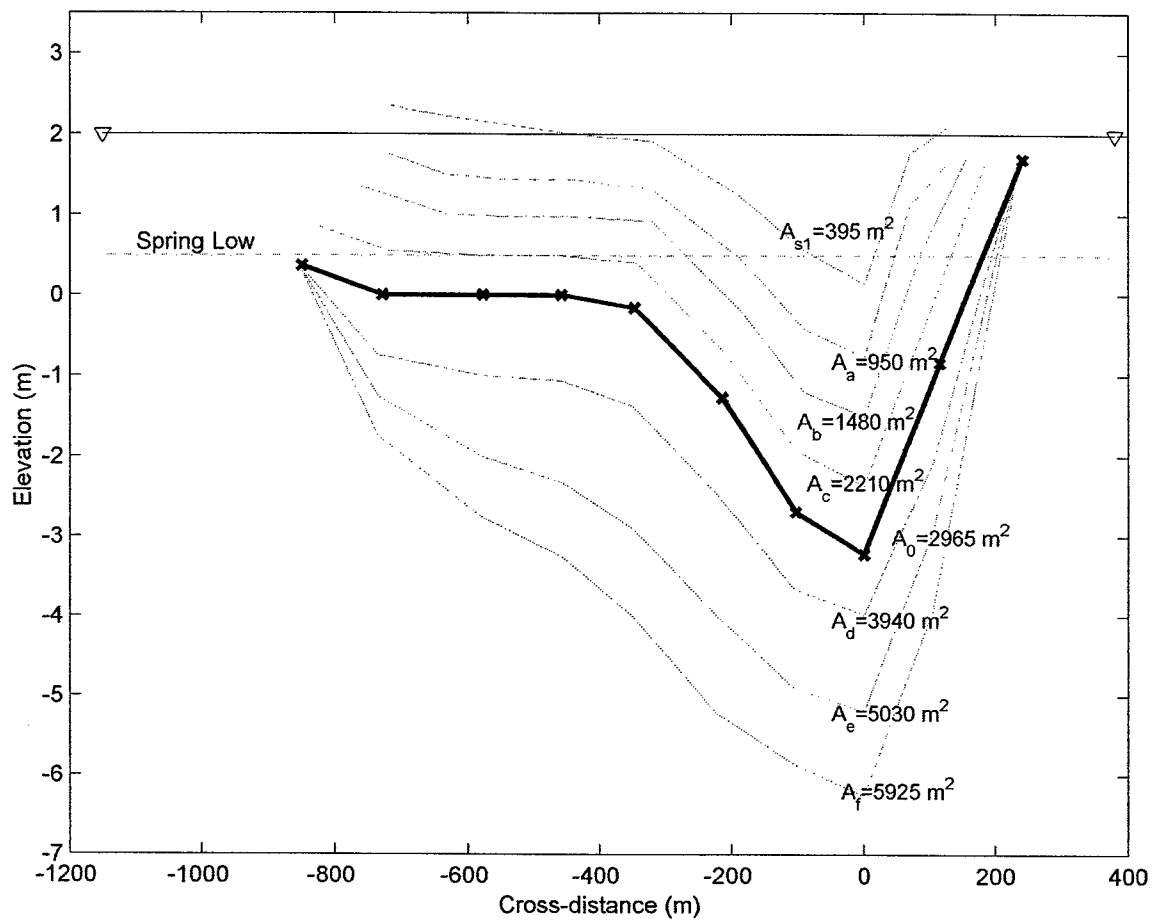
Figure 5-42. Armona Inlet cross-sectional areas used in the simulations.
