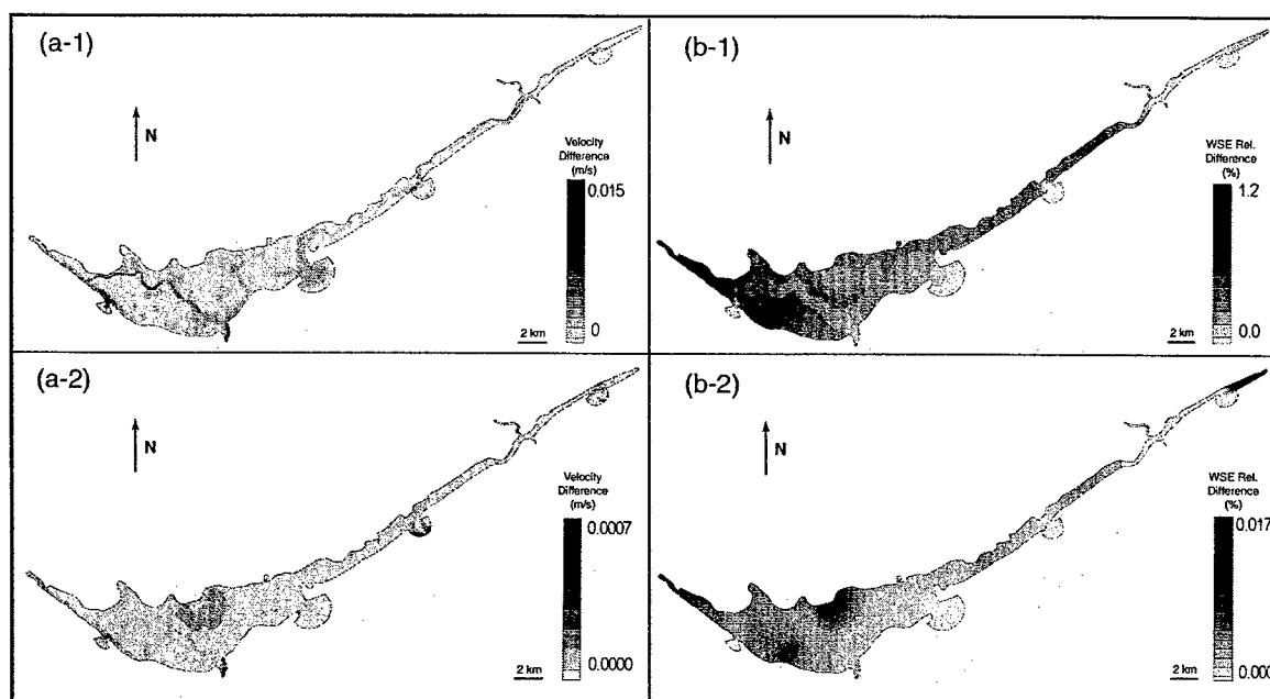
Figure 5-6. Velocity and water surface elevation (WSE) errors between consecutive tidal cycles throughout the lagoon. For velocity, the error is simply the difference between velocity magnitude at different times, and for WSE the error is the difference between the elevation at t_0 and at t_1 , relative to the elevation at t_0 . Velocity (a-1) and WSE (b-1) errors between t_0=1.91 and t_1=14.33 h; Velocity (a-2) and WSE (b-2) differences between t_0=12.42 and t_1=24.84 h (a-2).
