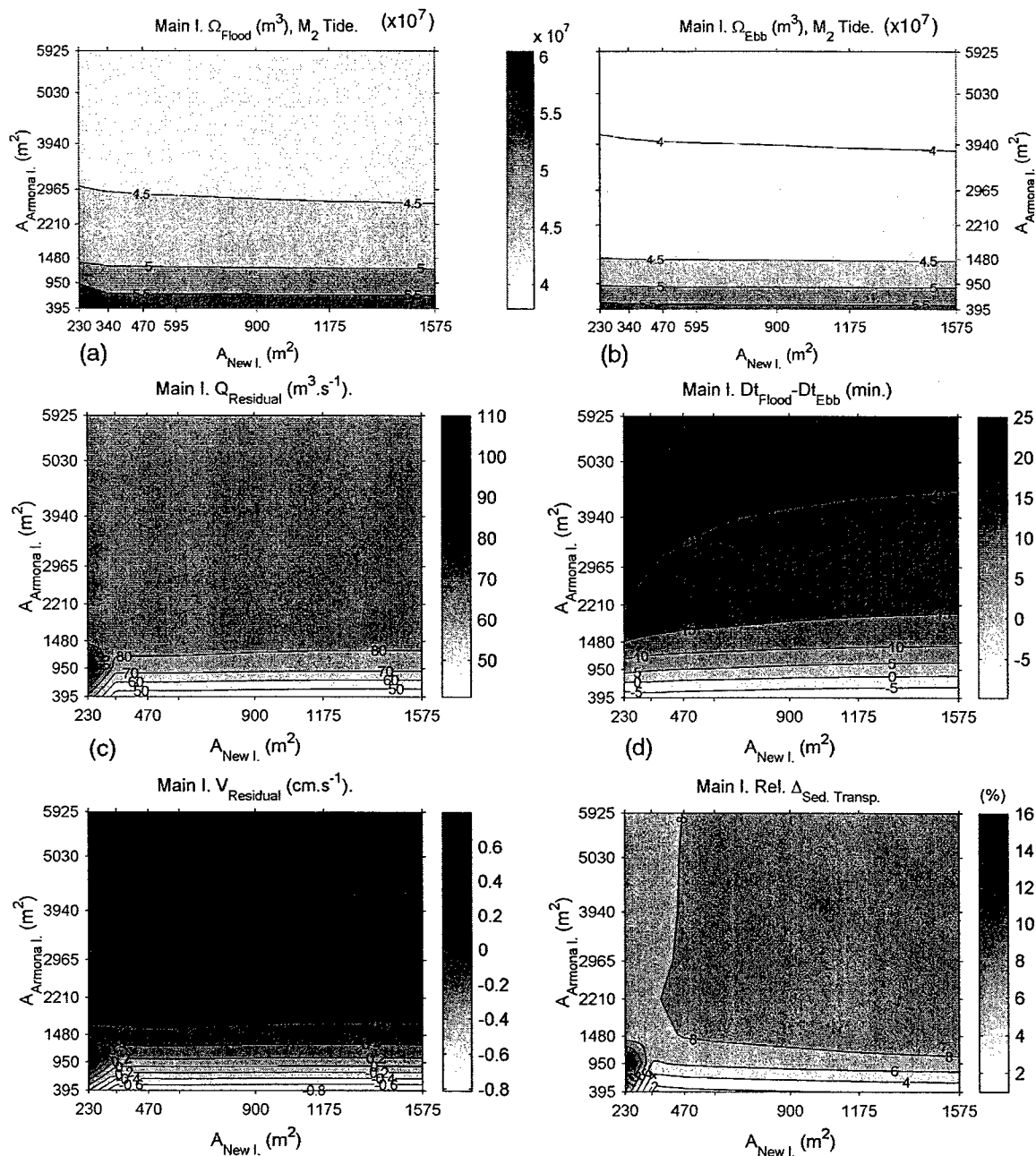
Figure 5-15. Results at Main Inlet from simulations with M_2 forcing, varying A_{Armona} and A_{New} ( A_{Main}=1,610 m^2 ). Flood and ebb tidal prisms (a and b); Residual discharge (c); Difference between flood and ebb durations (d); Residual current (e); and flood – ebb near-bed sediment transport difference, relative to the ebb sediment transport (f).
