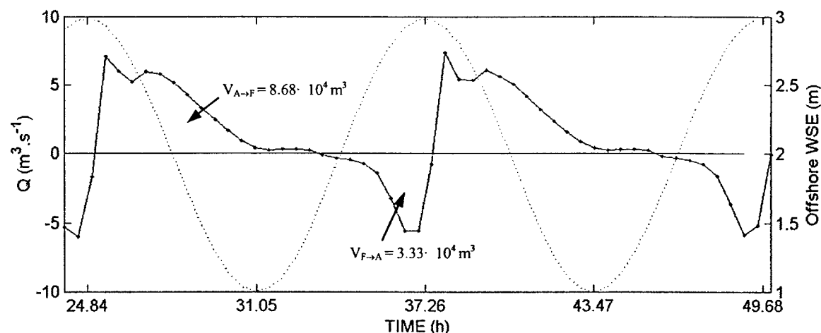
Figure 5-9. Discharge time series through the “hydrodynamic divide” between Armona and Fuzeta inlets ( V_{A \rightarrow F} : volume of flow in Armona-Fuzeta direction; V_{F \rightarrow A} : volume of flow in Fuzeta-Armona direction). The dotted line is the Offshore water surface elevation.
