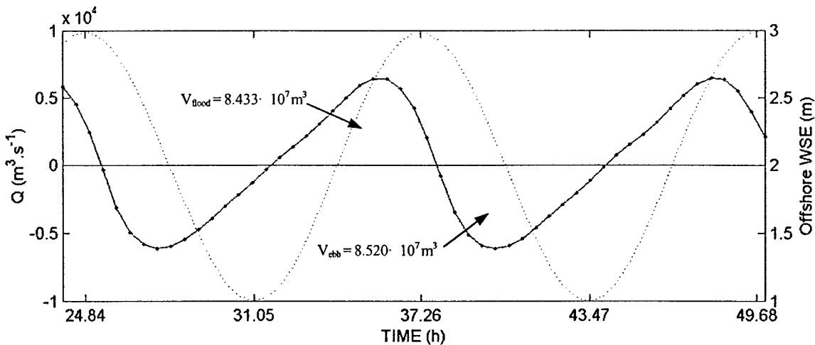
Figure 5-7. Total discharge through the inlets. Discharge (solid line); offshore WSE (dotted line).
