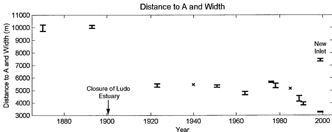
Figure 3-22. West Side inlet evolution. Width (represented by the error bars, and with the scale shown in the y-axis), and position with respect to baseline origin, point A (see Figure 3-20). The stars are data points from Vila et al. (1999).
