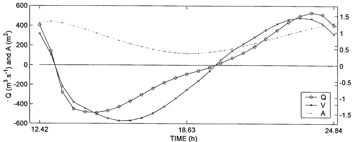
Figure 5-14. Discharge, velocity and cross-sectional area time series at New Inlet for simulation XAA, showing maximum discharge occurring during flood (positive) and maximum velocity occurring during ebb.
