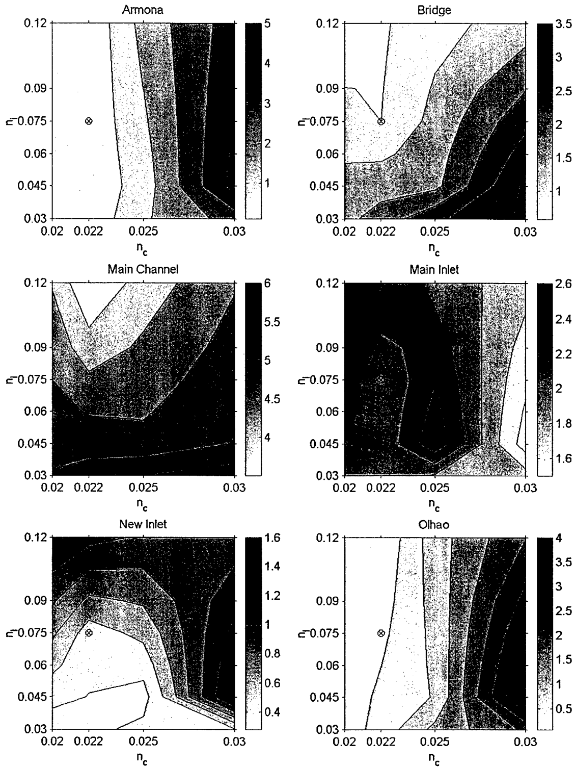
Figure 5-31. Friction Coefficient Calibration: M_4 amplitude absolute difference (cm) between model results and measurements (the circled cross corresponds to the friction coefficients chosen for the simulations).
