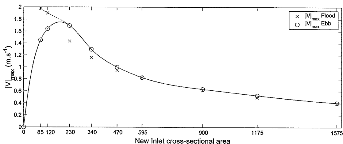
Figure 5-23. Maximum Flood and Ebb cross-sectionally averaged velocity magnitudes through New Inlet for runs [S 2 XA, S 1 XA, AXA, BXA, CXA, XXA, DXA, EXA, FXA].
