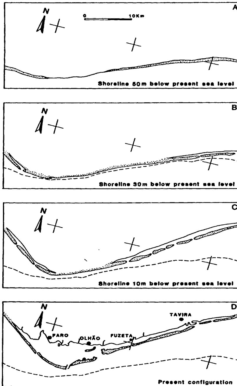
Figure 3-4. Hypothesized sequence of the Ría Formosa formation (from Pilkey et al. , 1989). The dashed reference line represents the isobath at 50m below present sea level.
