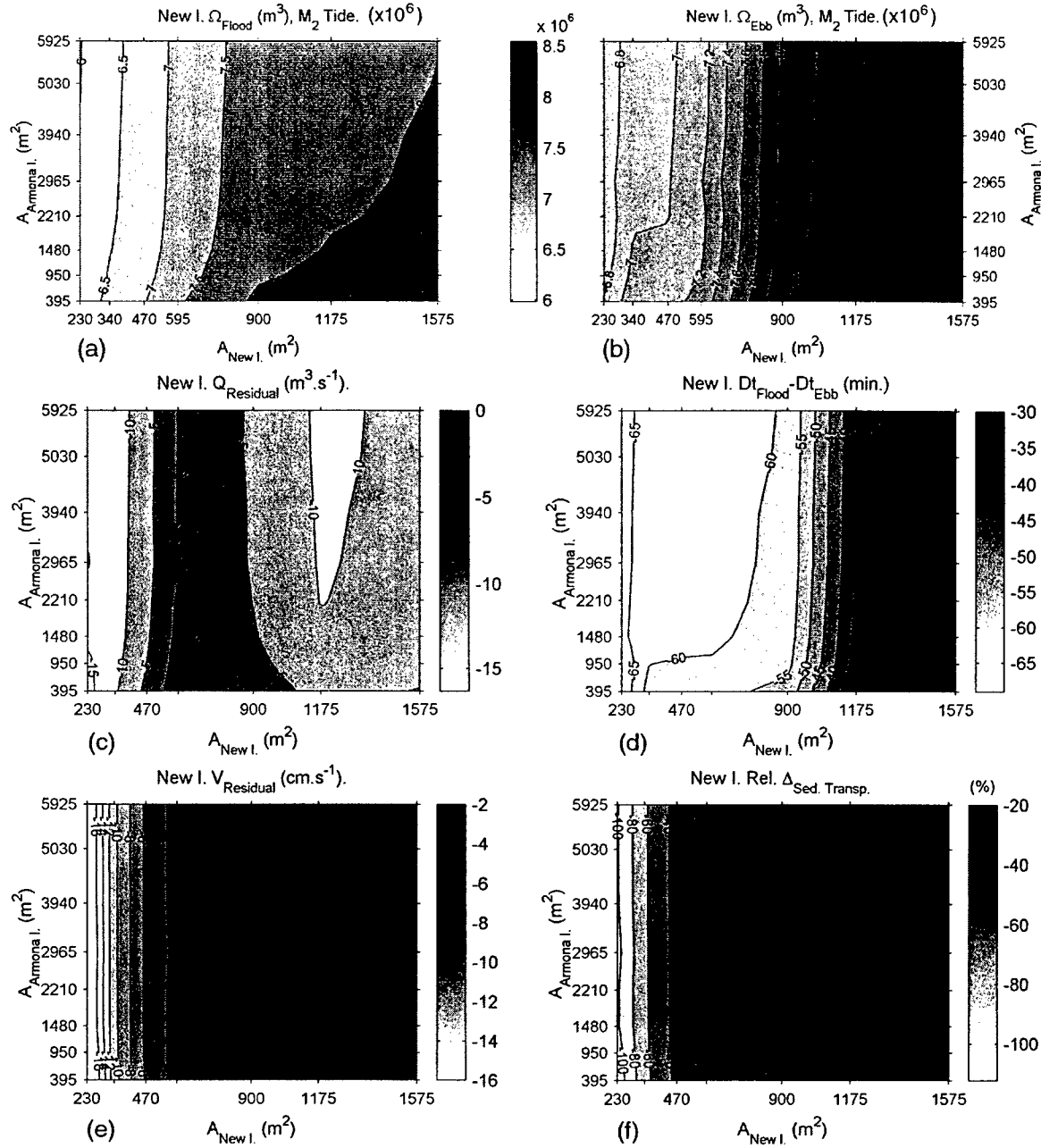
Figure 5-12. Results at New Inlet from simulations with M_2 forcing, varying A_{Armona} and A_{New} ( A_{Main}=1,610 \text{ m}^2 ). Flood and ebb tidal prisms (a and b); Residual discharge (c); Difference between flood and ebb durations (d); Residual current (e); and flood – ebb near-bed sediment transport difference, relative to the flood sediment transport (f).
