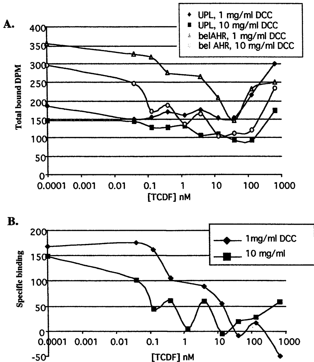
Figure 1. Competitive binding assay with dextran-coated charcoal (DCC).
