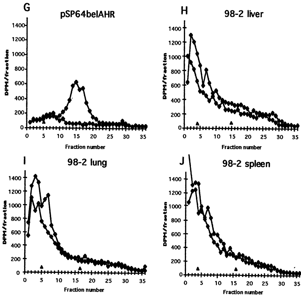
Figure 5. Specific 3 H-TCDD binding in 98-1 and 98-2 belugas. Cytosols were incubated with 3 H-TCDD, plus DMSO or 200-fold excess TCDF, applied to a sucrose gradient and sedimented. Solid diamonds represent total binding disintegrations per minute (DPM) per fraction, hollow diamonds are non-specific binding DPM/fraction. Small triangles indicate peak of 14 C-labeled 3.6 S and 11.3 S protein size standards. Specific binding (fmol/mg) and sedimentation coefficients are indicated. Panels (A) through (F) show 98-1 tissue cytosols. Panels (H) through (J) show binding in tissue cytosols from beluga 98-2. Panel (G) shows binding of TNT expressed beluga AHR, used as a positive control run for samples in panels (D) through (J).
