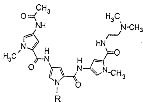
MGT-6a R =
