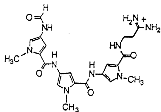
Distamycin
