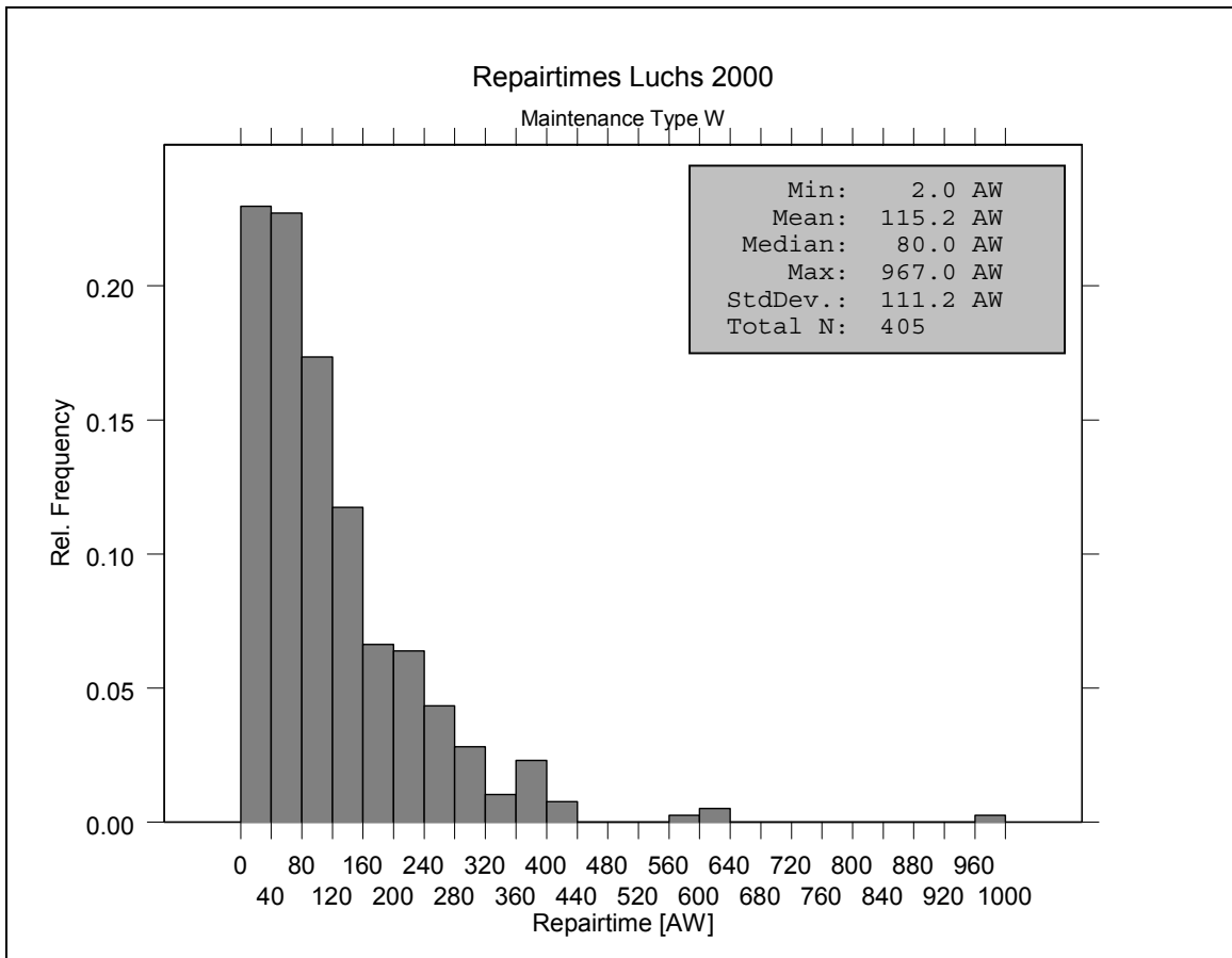
Figure 4.5 Histogram of Luchs Repairtimes (Weapon).
