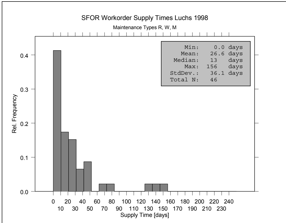
Figure 5.7 Workorder Supply Times SFOR.
