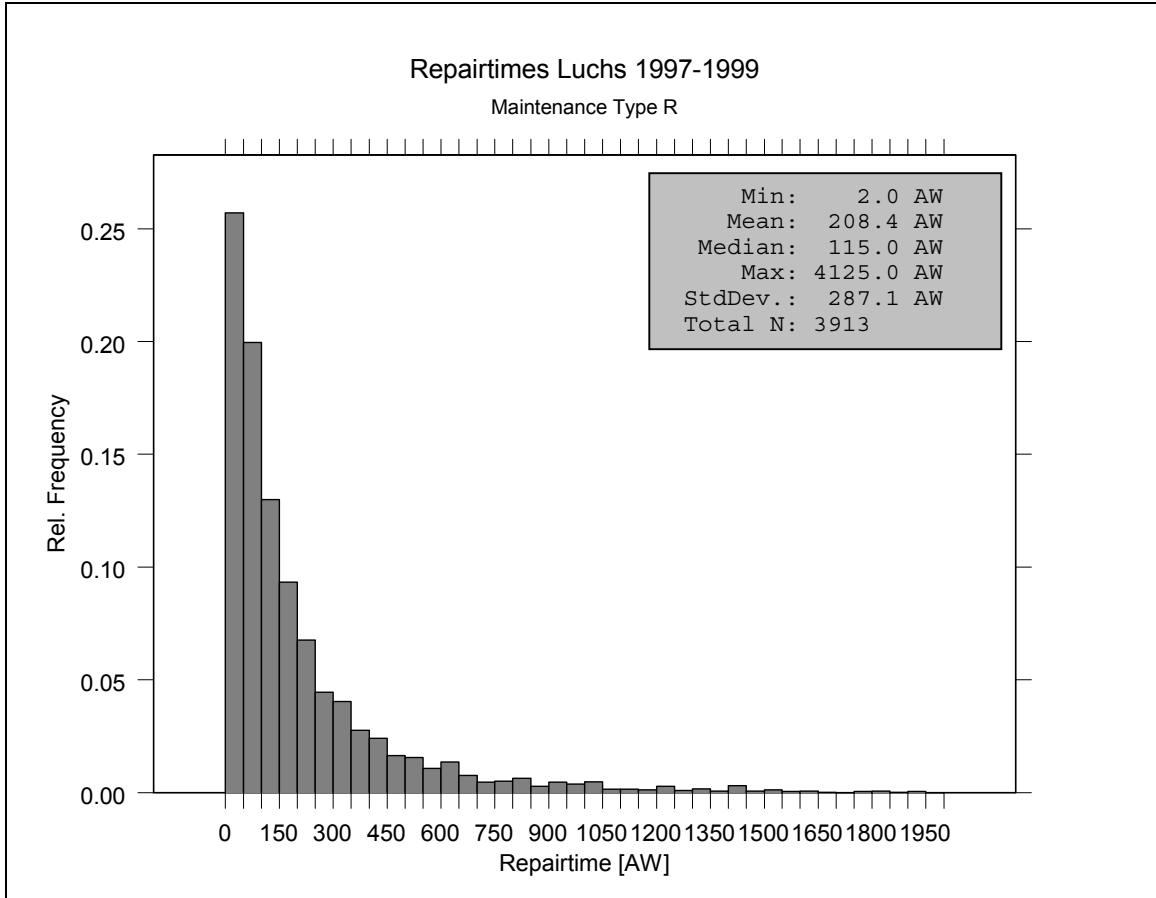
Figure 4.1 Histogram of Luchs Repairtimes (Vehicle). There are 10 workorders with repairtimes > 2000 AW and 84 workorders with repairtimes > 1069 AW (which represents mean + 3*SD) within this data set. These repairtimes are extraordinarily long, which could indicate that the workorders are incorrect and should be excluded from the analysis. However, a careful examination of each of these workorders showed that extensive and complex work resulted in these outliers. All of these workorders should have been shifted to the Depot Maintenance level. Limited budgets for Depot Maintenance in recent years might be a reason for performing these repairs at the Intermediate Maintenance level.
