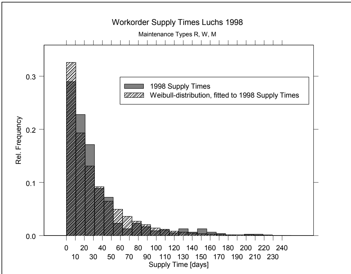
Figure 5.6 Workorder Supply Time Distribution vs. Weibull-model. The model shows a good fit to the 1998 workorder supply times.
