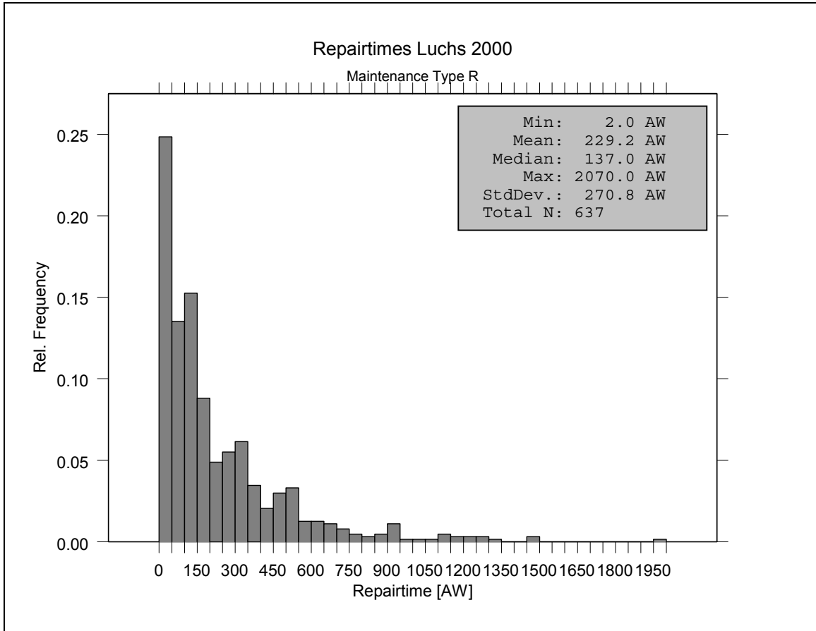
Figure 4.2 Histogram of Luchs Repairtimes (Vehicle) from 2000. The histogram does not look as smooth as in Figure 4.1 because the number of bars (40) is quite high for the total number of observations (637). However, using the same number of bars in both figures simplifies comparisons between the two histograms. Figure 4.2 is based on the reduced dataset (after removal of 30 collective workorders).
