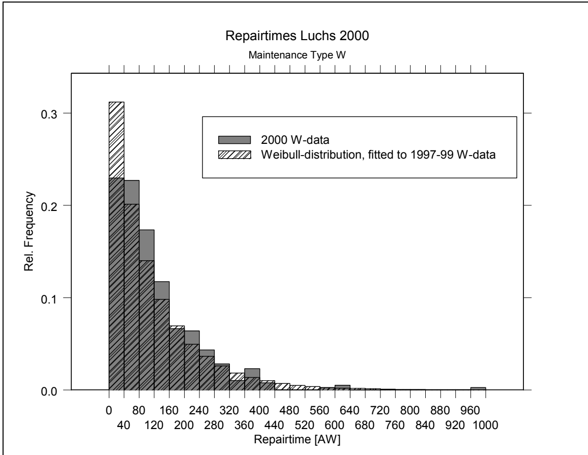
Figure 4.6 Comparison between Actual Data and Fitted Weibull Distribution.
