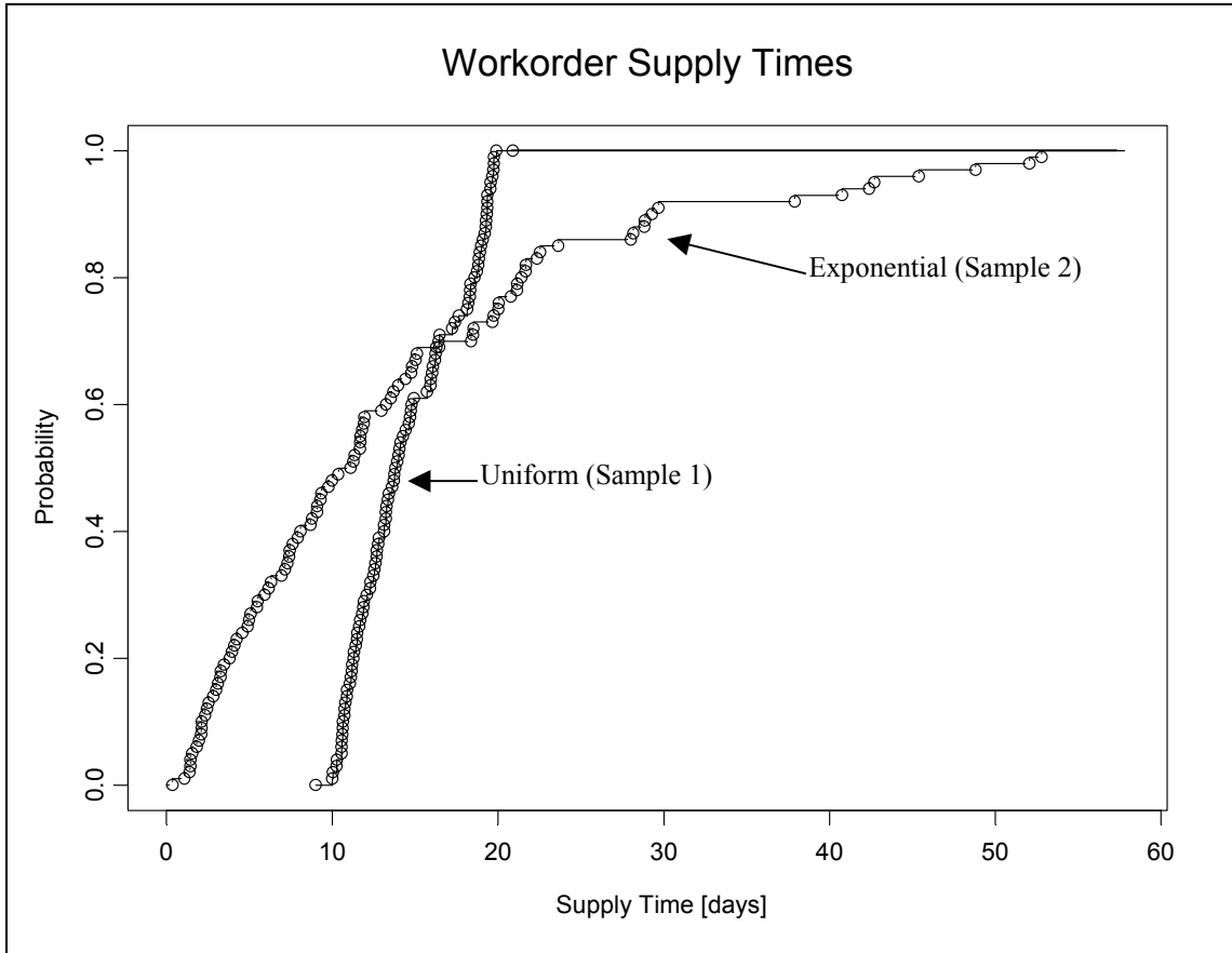
Figure 5.10 Comparison between Samples from Distributions with Different Variances. Both samples have a mean of 14 days. The sample from the uniform distribution has a standard deviation (SD) of 3.2 days, whereas the sample from the exponential distribution has a SD of 12.1 days. After 20 days all workorders from Sample 1 are supplied. At the same time, only about 70% of the workorders of Sample 2 are supplied.
