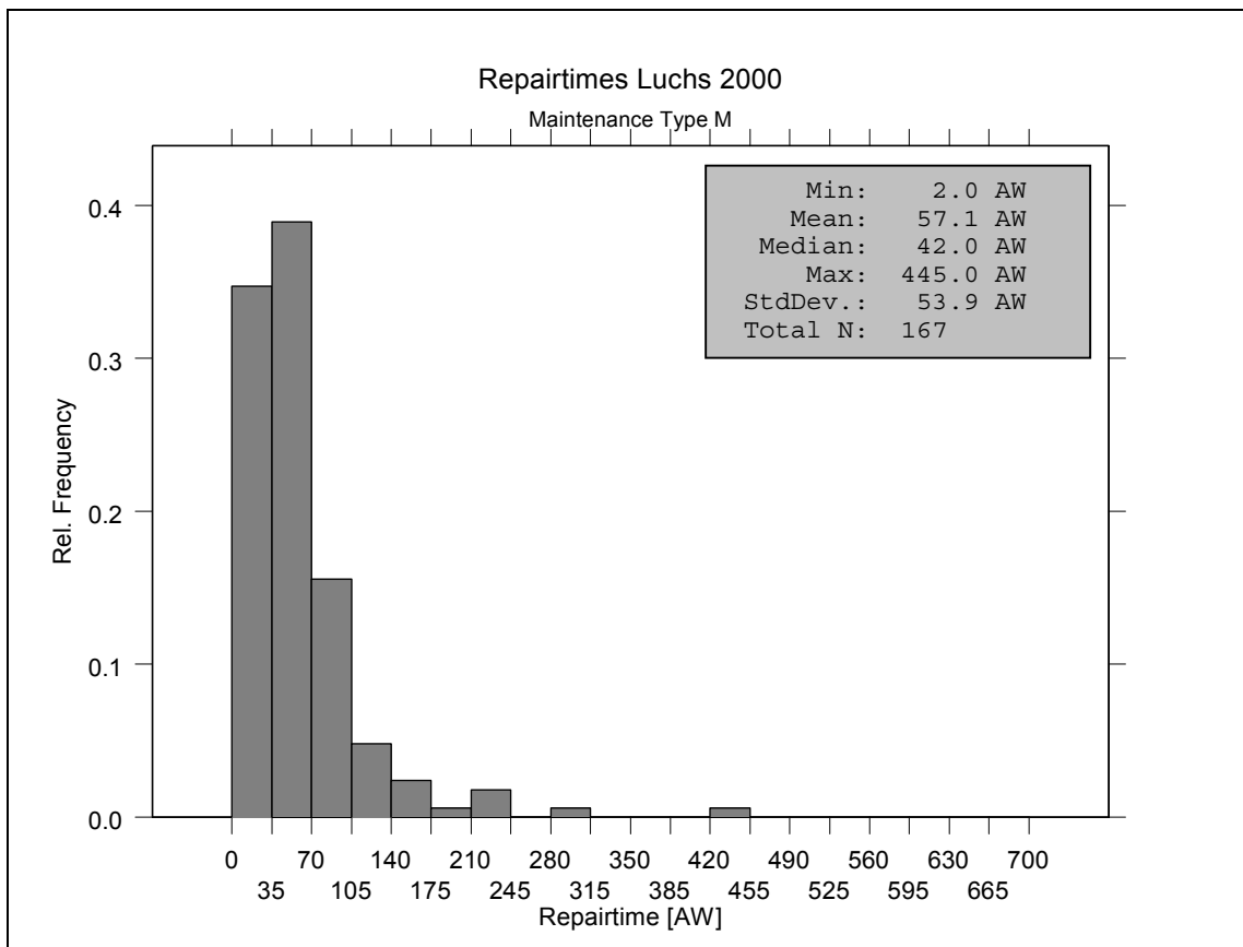
Figure 4.8 Histogram of Luchs Repairtimes (Radio Equipment).
