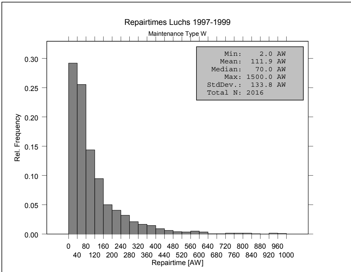
Figure 4.4 Histogram of Luchs Repairtimes (Weapon). The shape of the distribution is quite similar to the previous ones. Again, a Weibull distribution seems a reasonable approach to model the repairtimes.
