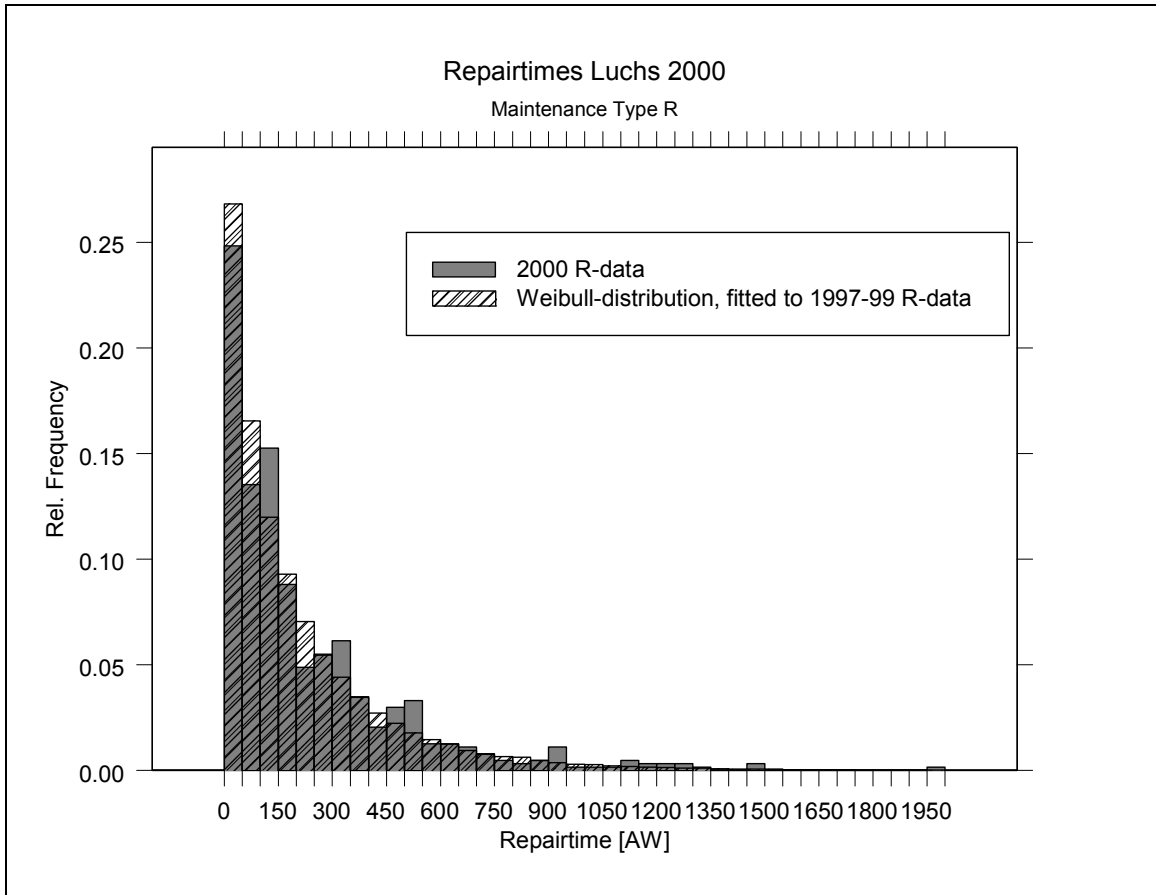
Figure 4.3 Comparison between Actual Data and Fitted Weibull Distribution. The histogram shown in Figure 4.2 was supplemented with the histogram bars obtained by generating 100,000 numbers from the Weibull distribution fitted to the 1997-99 data. The optical impression of a good fit supports the conclusion of the Kolmogorov-Smirnov goodness-of-fit test.
