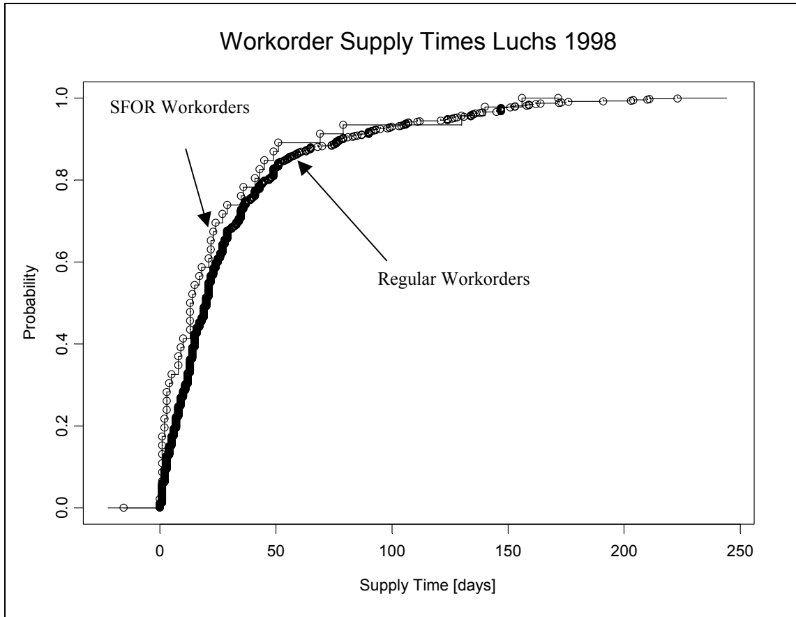
Figure 5.9 Comparison between Regular Workorder Supply Times and SFOR Workorder Supply Times. This plot supports the results from the permutation test in Section C. The empirical distribution function of the 1998 SFOR workorder supply times has a similar shape as the distribution function of the regular workorder supply times.
