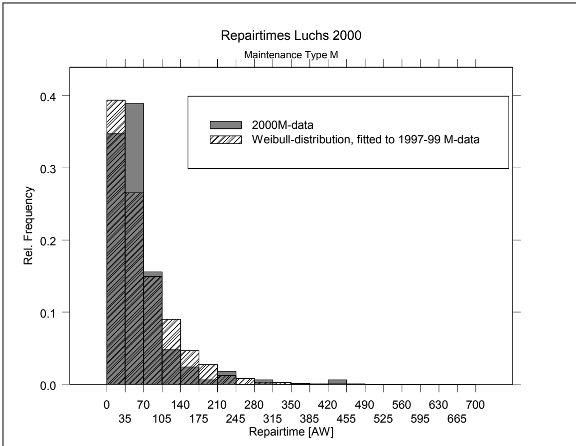
Figure 4.9 Comparison between Actual Data and Fitted Weibull Distribution.
