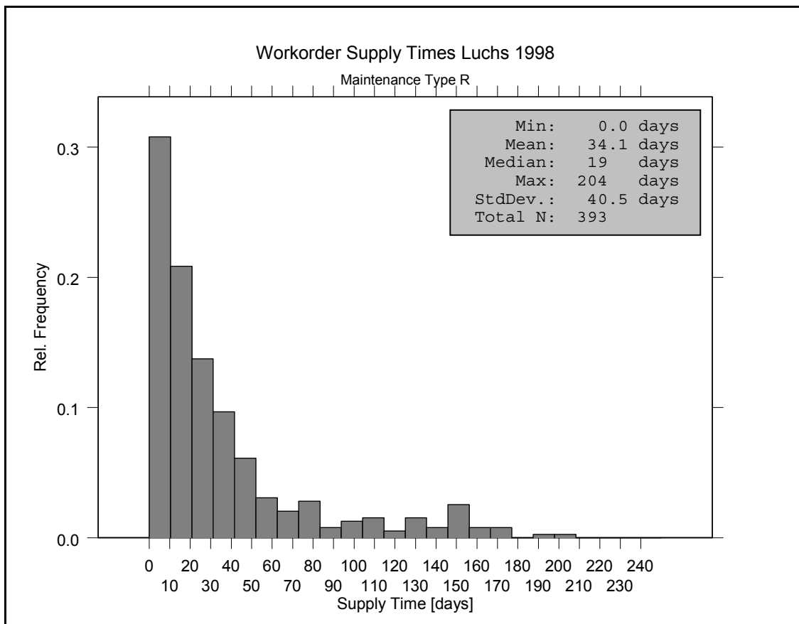
Figure 5.2 Workorder Supply Time Distribution (Vehicle).
