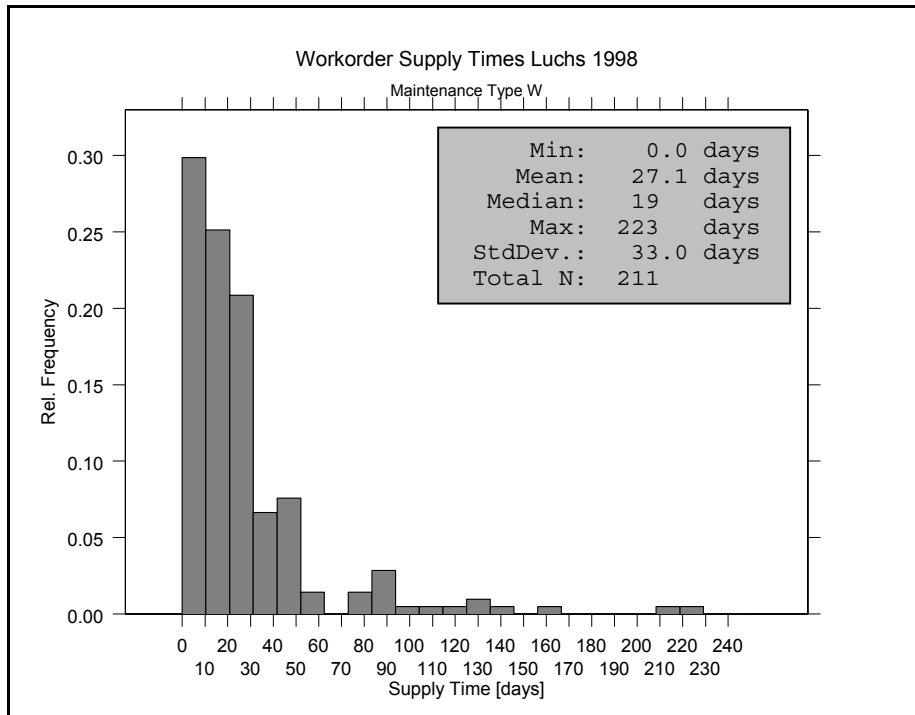
Figure 5.3 Workorder Supply Time Distribution (Weapon).
