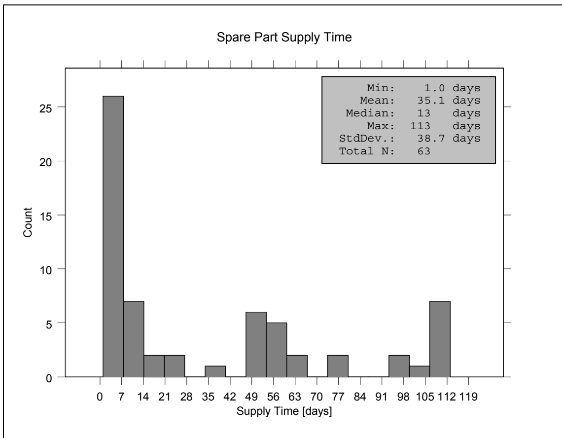
Figure 5.1 Distribution of Spare Part Supply Times for Stock Number 2530123005149. This histogram shows how misleading an average in a skewed distribution can be. Although the average supply time for this item is 35.1 days, 50 percent of orders arrived within the median supply time of 13 days.
