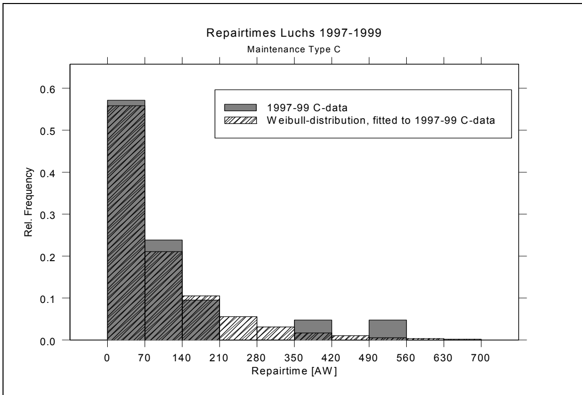
Figure 4.11 Comparison between Actual Data and Fitted Weibull Distribution.
