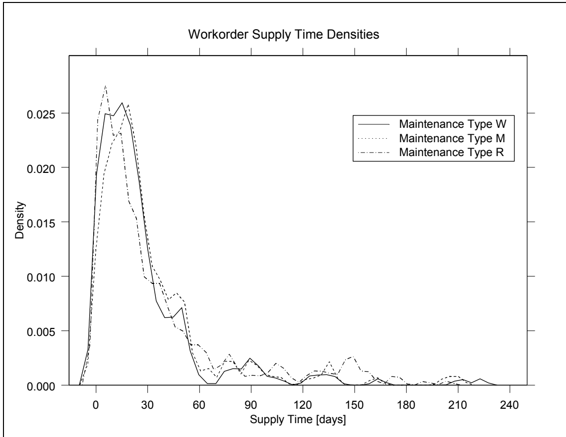
Figure 5.5 Comparison Between Density Lines.
