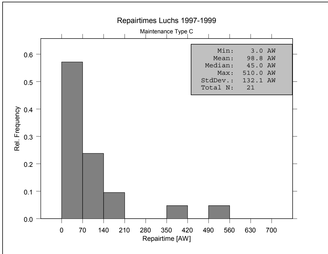
Figure 4.10 Histogram of Luchs Repair times (Optical Equipment).
