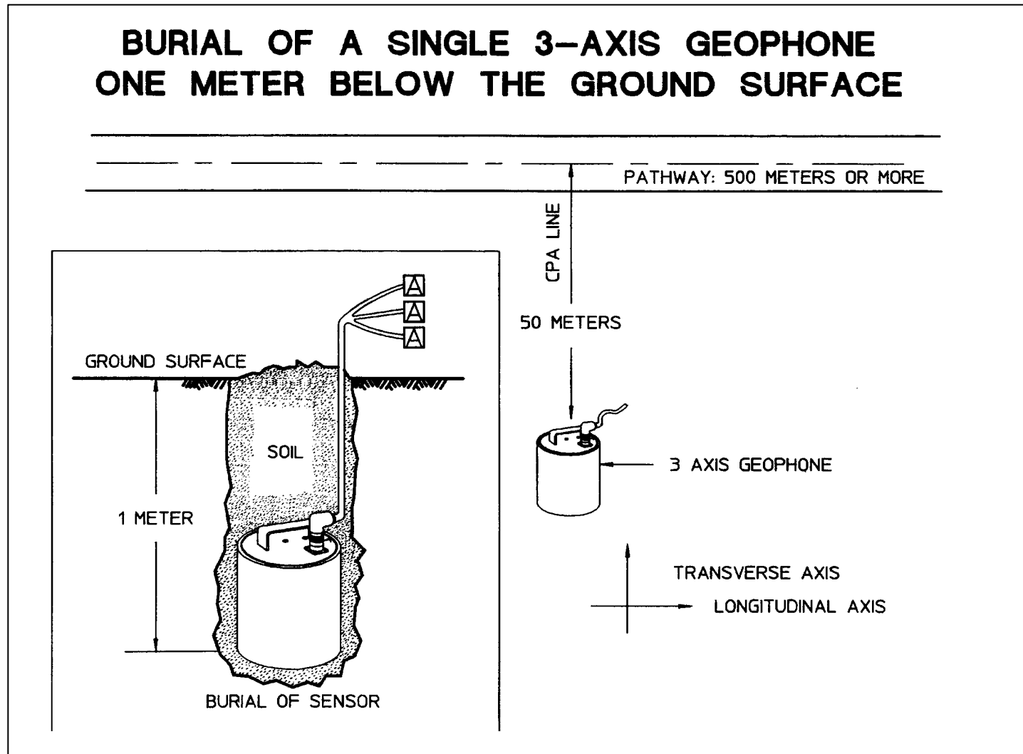
Figure A-3. Burial of a single 3-axis geophone one meter below the ground surface.
