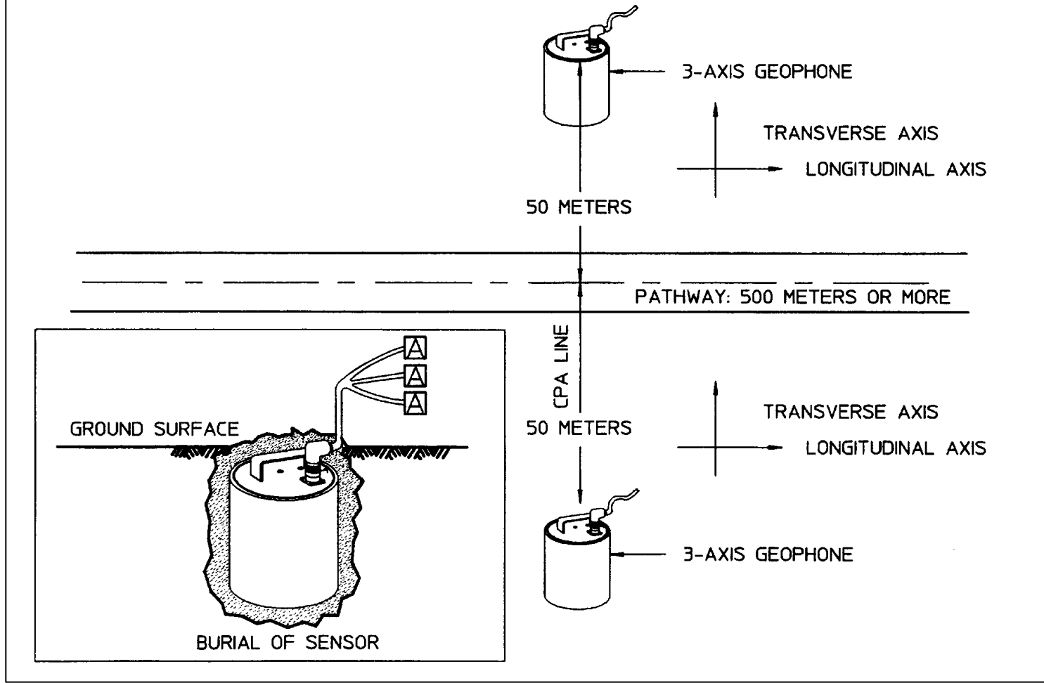
Figure A-4. Burial of 3-axis geophone on both sides of the pathway.
