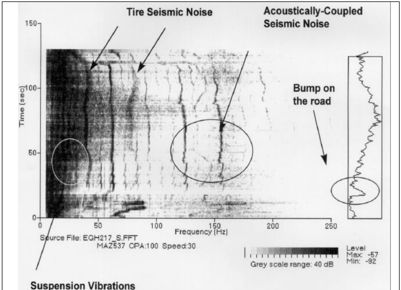
Figure 2-1. Seismic data sample shows acoustic coupling spectral lines. (Note: level is expressed in dB ref 1V/m/sec.)
