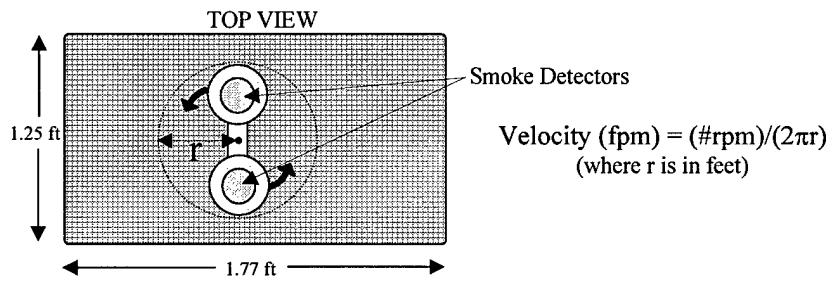
Figure 12. Top View of Air Velocity Testing Platform
