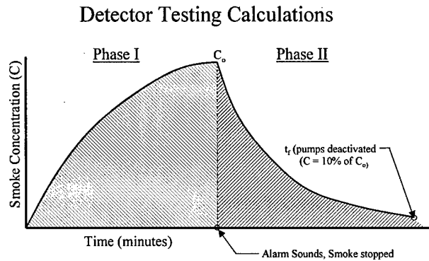
Figure 8. Test Chamber Smoke Concentration Plot
