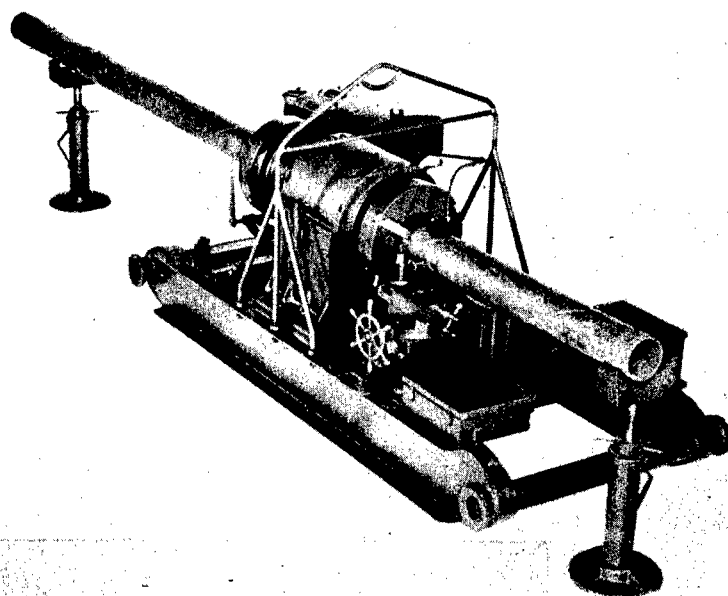
Pipe-Cutting & Grooving Machine.
