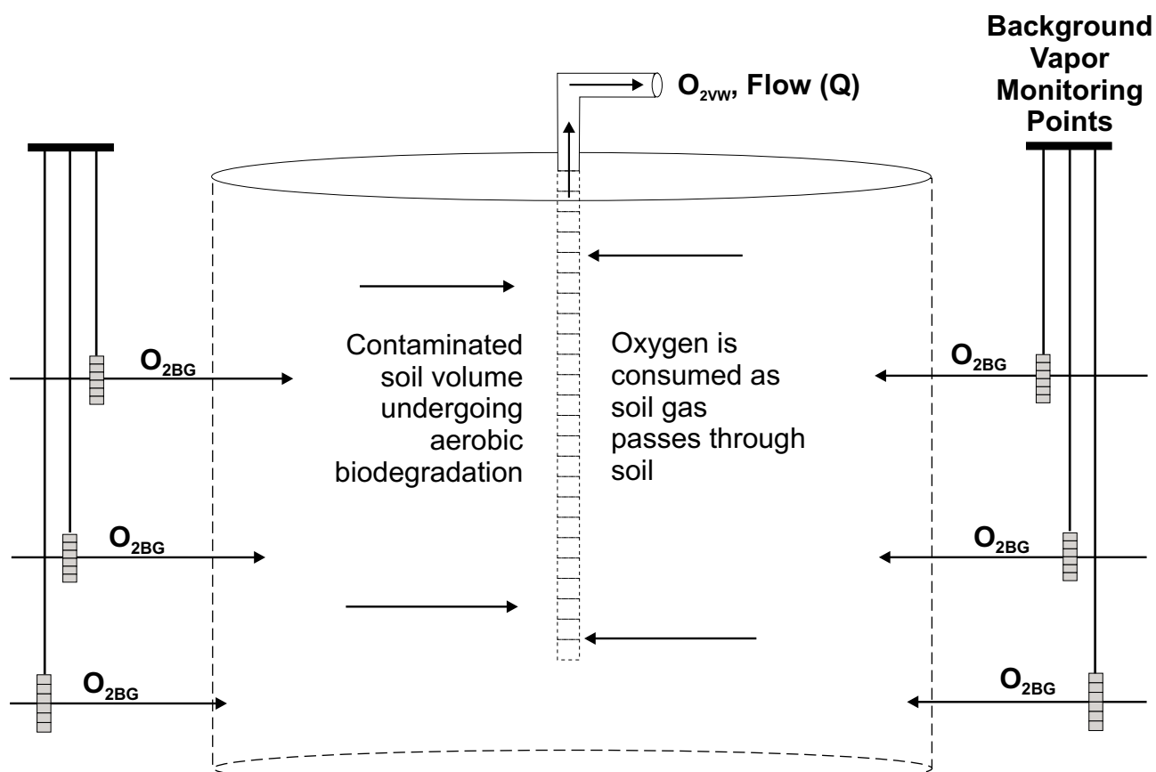
Figure 4.5 ESTIMATION OF BIODEGRADATION AT SVE SITES
