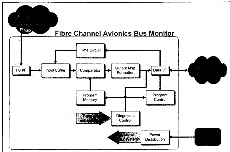
Figure 2 Block Diagram
