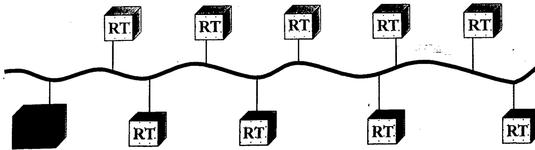
Figure 2, 1553 Bus Architecture
