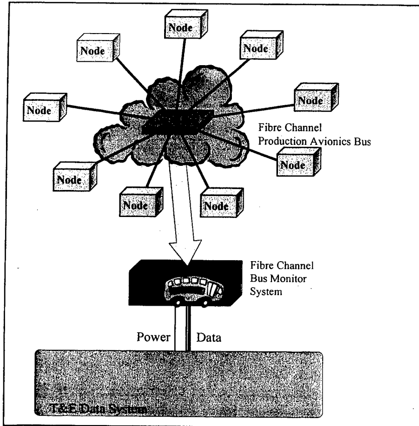
Figure 4 Fibre Channel Bus Monitor System Context
