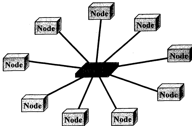
Figure 3, Fibre Channel Switched Fabric Architecture
