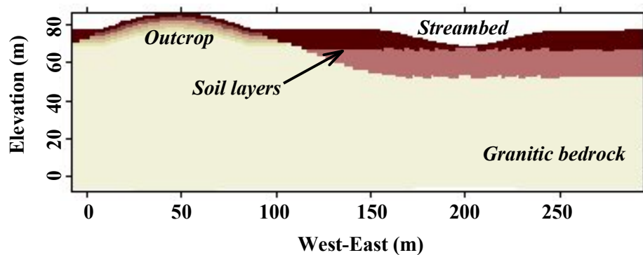
Figure 2. Slice through model at South-North coordinate = 128 m. Distinct shades in graph illustrate layering, with principal layers being granitic bedrock and soil below and above water table. Shading variations in bedrock outcrop are property variations to imposed “weathering.”
