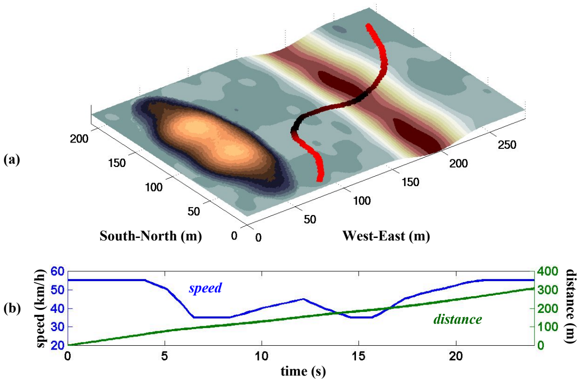
Figure 4. (a) Vehicle path over topographic surface and (b) vehicle speed and distance vs. time.
