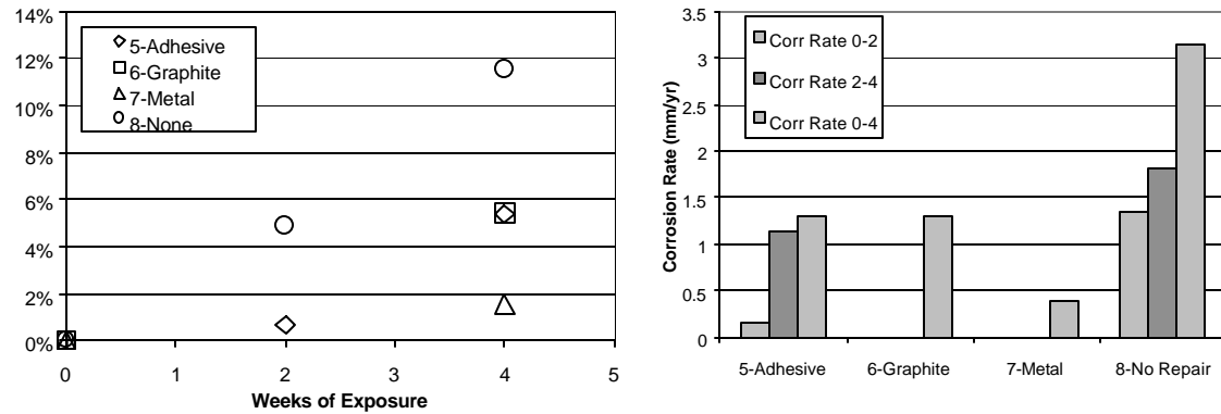
Figure 6: Repair Evaluation % Mass Loss and Corrosion Rate Graphs
