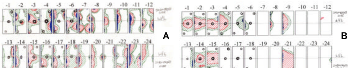
Figure 9: Damage Maps - A) graphite B) metal
