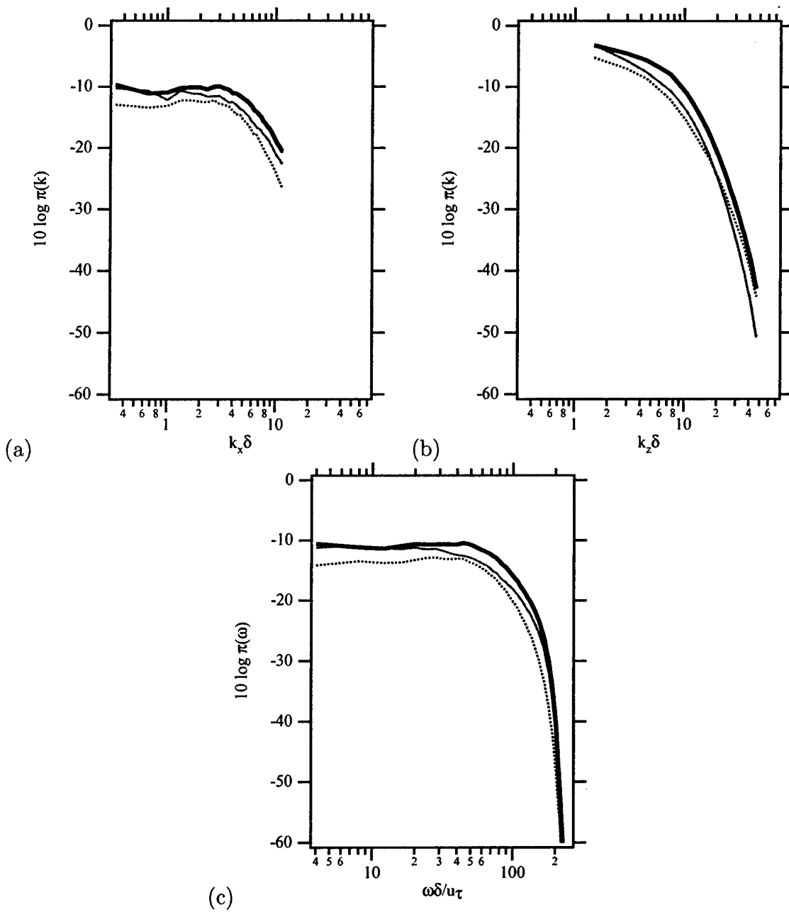
Figure 7. One-dimensional spectra of partial pressures for sources integrated over entire channel (R1234). — : \pi^{tot} ; - - : \pi^{MS} ; ..... : \pi^{TT} ; (a) streamwise wavenumber (b) spanwise wavenumber and (c) frequency.
