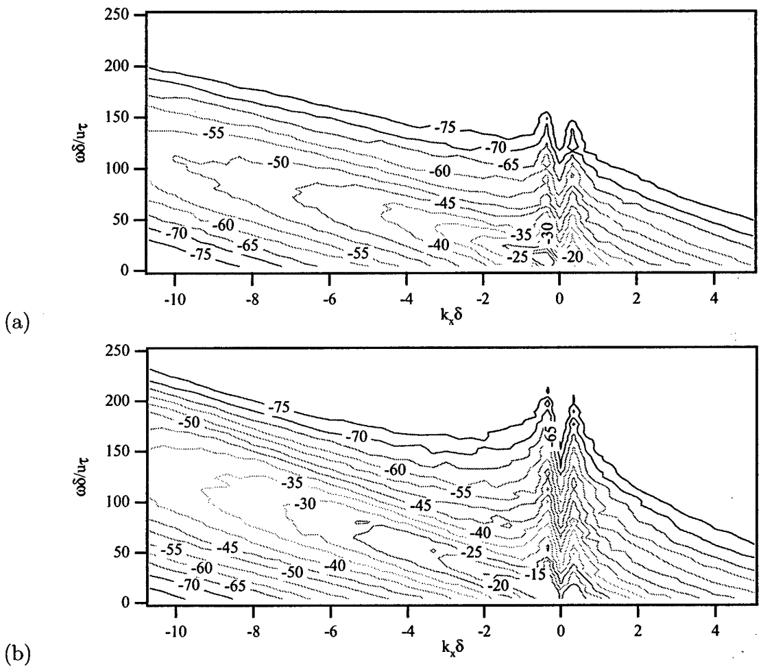
Figure 18. Two-dimensional contour plots of k_x - \omega spectra of \pi^{TT} from LES9; (a) viscous shear layer (R1) and (b) buffer layer (R2).
