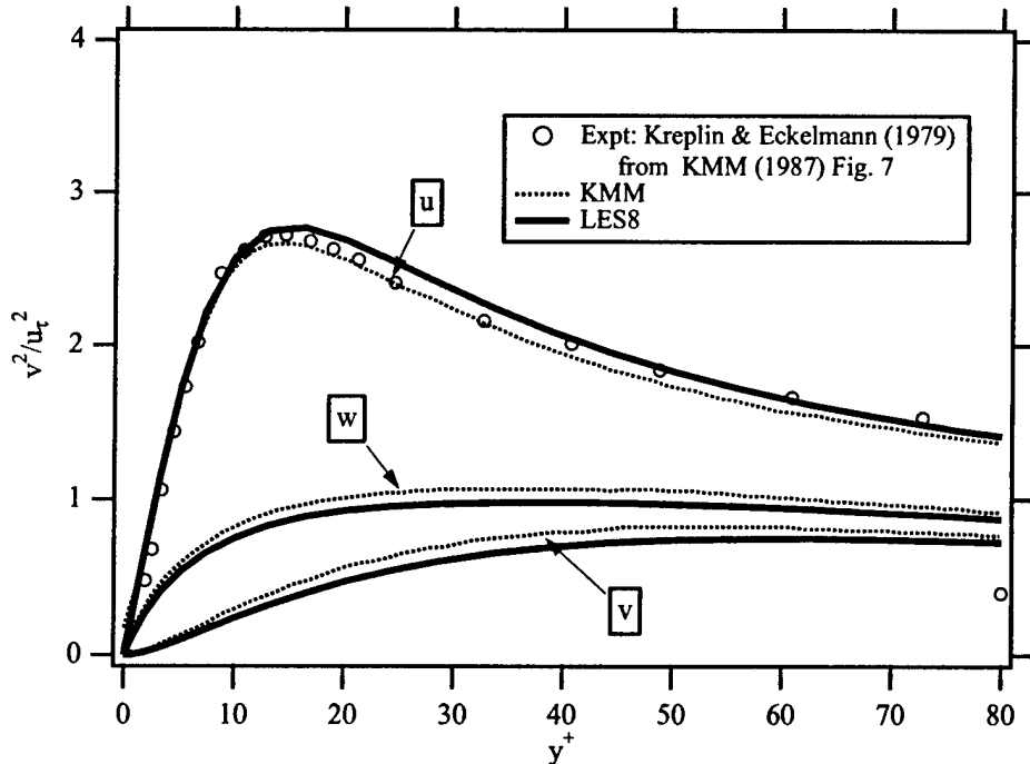
Figure 2. Turbulence intensity profiles; — : LES8; ..... : Kim et al. 4 ; o : Kreplin and Eckelmann 9
