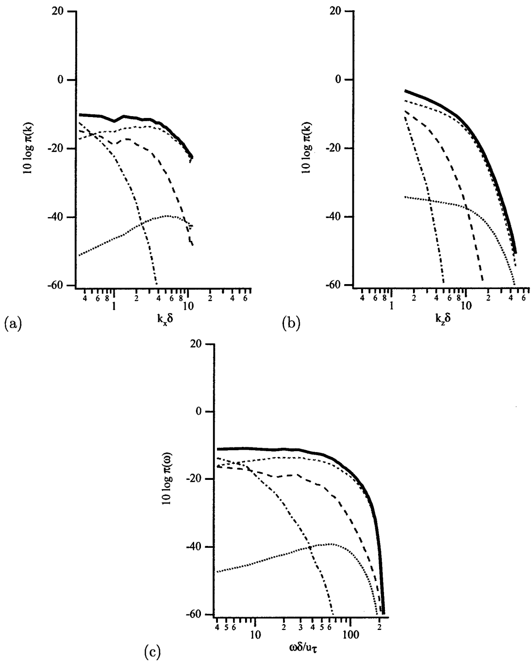
Figure 12. One-dimensional spectra of \pi^{MS} from LES8; (a) streamwise wavenumber and (b) spanwise wavenumber and (c) frequency; — : all regions (R1234), ..... : viscous shear layer(R1), -·-·- : buffer layer, - - - : logarithmic region, and - - - : upper channel.
