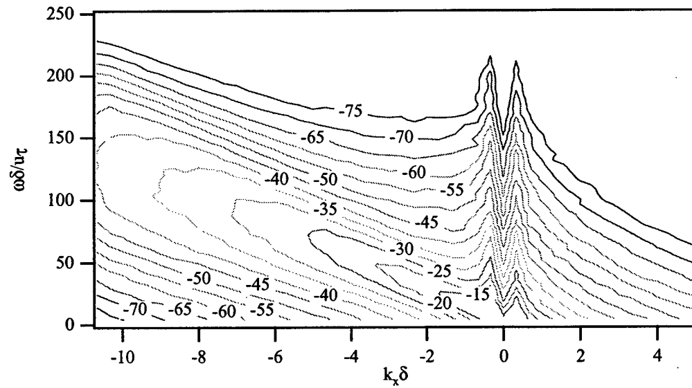
Figure 16. Two-dimensional contour plots of k_x - \omega spectra of \pi^{TT} from LES8; (a) viscous shear layer (R1) and (b) buffer layer (R2).
