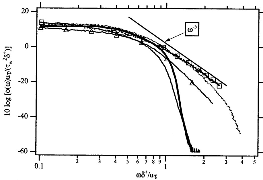
Figure 4. Comparison of (a) outer- and (b) inner-scaled ( \delta^+ \equiv \nu/u_\tau ) point frequency spectra; — : LES8, ..... : DNS5, — : Singer. 11 \Delta : Farabee and Casarella 12 , and \square : Gravante et al. 13 .
