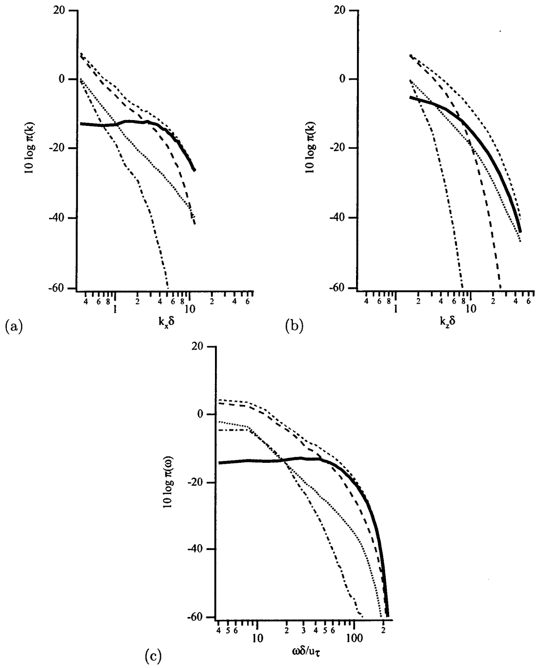
Figure 13. One-dimensional spectra of \pi^{TT} from LES8 (a) streamwise wavenumber and (b) spanwise wavenumber and (c) frequency. — : all regions (R1234), ..... : viscous shear layer(R1), -·-·-· : buffer layer(R2), - - - - : logarithmic region(R3), and - - - - : upper channel(R4).
