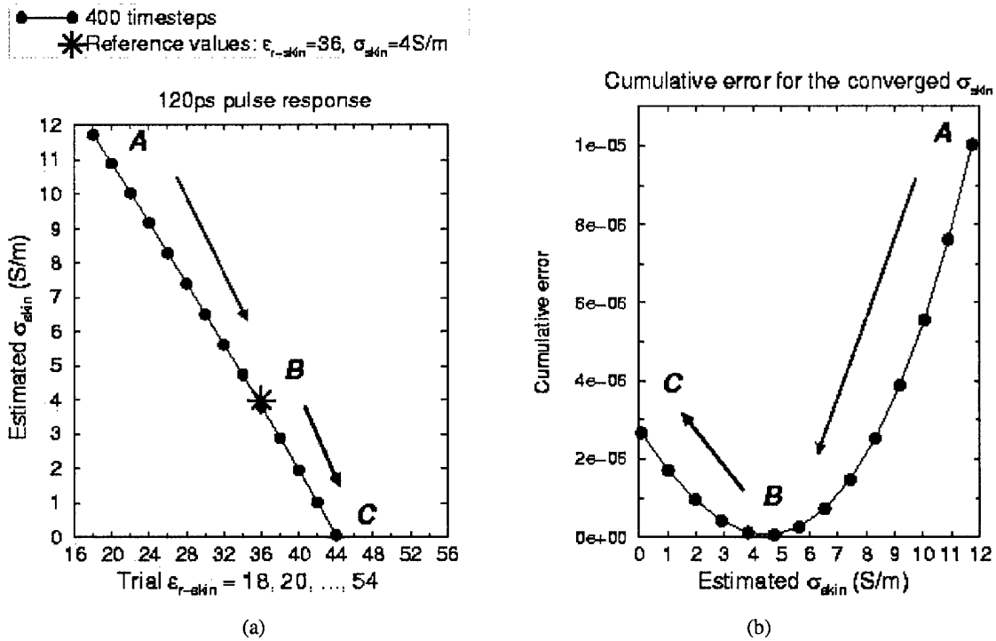
Figure 3. Results for the 120-ps differentiated Gaussian pulse excitation. (a) Search trajectory in (\epsilon_{r\text{-skin}}, \sigma_{\text{skin}}) space search. T_{\text{window}} = 400 time steps, where \Delta t = 0.3335 \text{ ps} . (b) The cumulative error vs. estimated \sigma_{\text{skin}} values, showing a broad null at the location of the assumed accurate values of the skin parameters.
