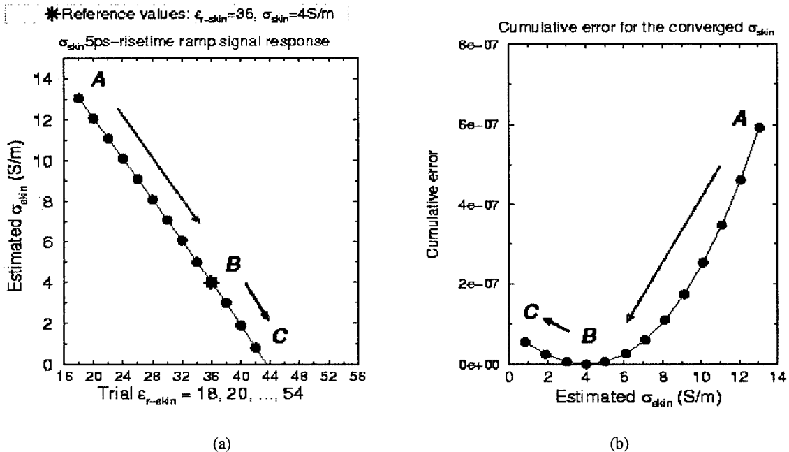
Figure 5. Results for the 5-ps risetime ramp signal excitation. The amplitude of the excitation is the same as the maximal value of the 5-ps risetime differentiated Gaussian with results in Fig. 4. (a) Search trajectory in (\epsilon_{r-skin}, \sigma_{skin}) space. T_{window} = 100 time steps, where \Delta t = 0.3335ps . (b) The cumulative error vs. estimated \sigma_{skin} value, showing a broad null at the location of the assumed accurate values of the skin parameters.
