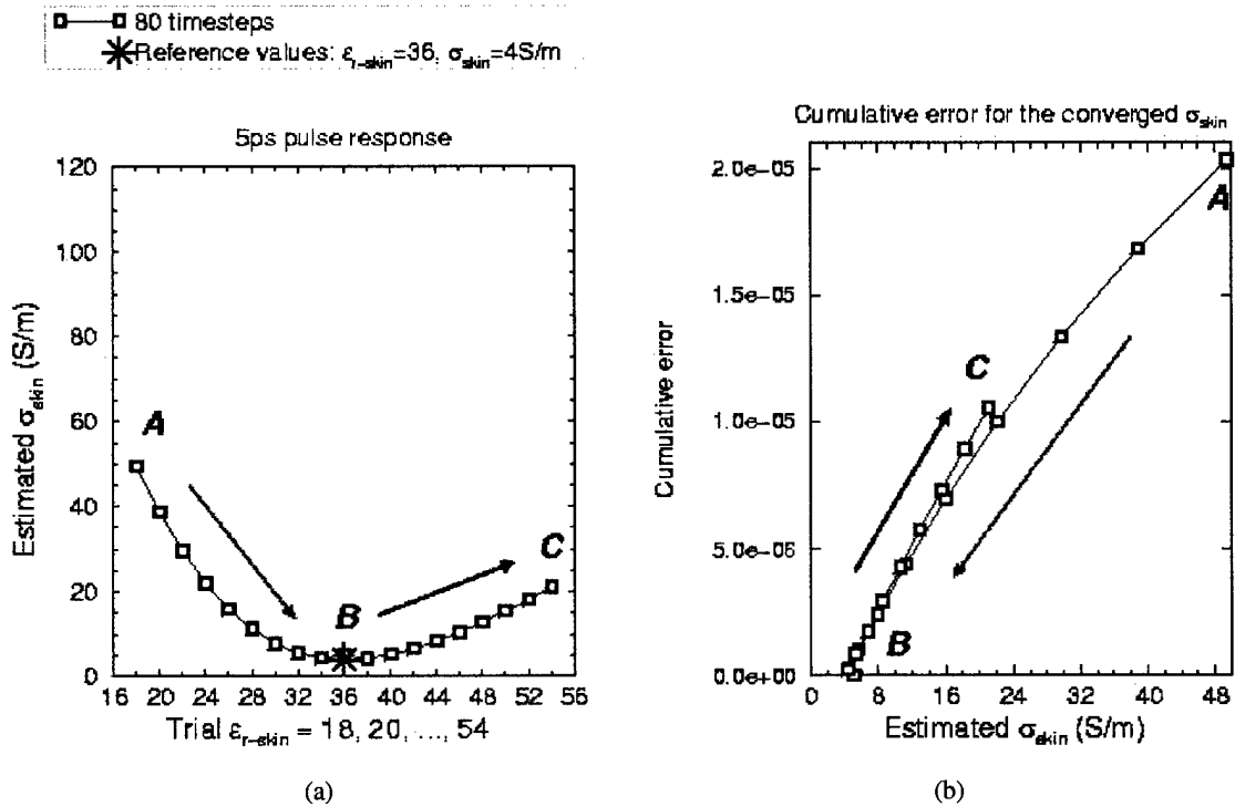
Figure 4. Results for the 5-ps differentiated Gaussian pulse excitation. (a) Search trajectory in (\epsilon_{r-skin}, \sigma_{skin}) space. T_{window} = 80 time steps, where \Delta t = 0.3335ps . (b) The cumulative error vs. estimated \sigma_{skin} values, showing a sharp null at the location of the assumed accurate values of the skin parameters.
