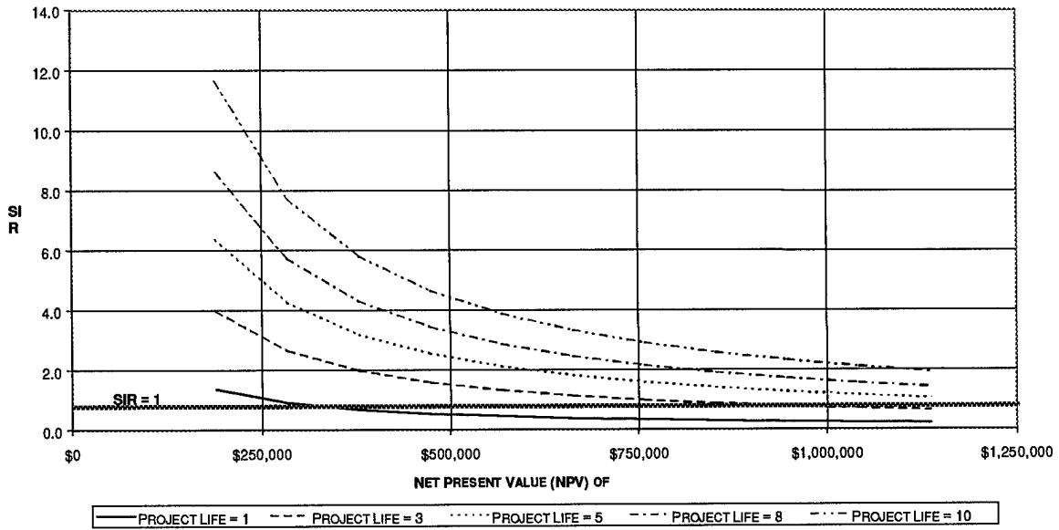
Figure 7. Four-Stroke Outboards for RIBs Cost Sensitivity Analysis (Net Present Value of Investment)
