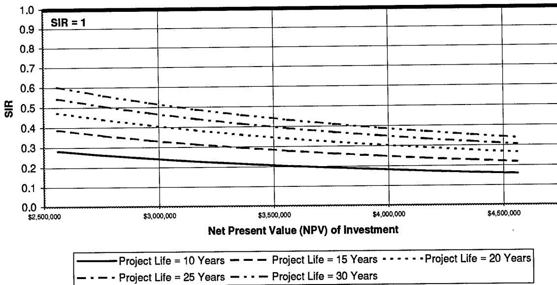
Figure 5. Advanced Propellers for 87' WPB Cost Sensitivity Analysis (Net Present Value of Investment)
