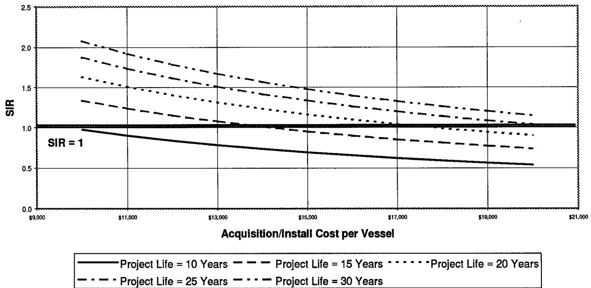
Figure 2. Stern Flaps for 87' WPB Cost Sensitivity Analysis (Acquisition/Install Cost per Vessel)
