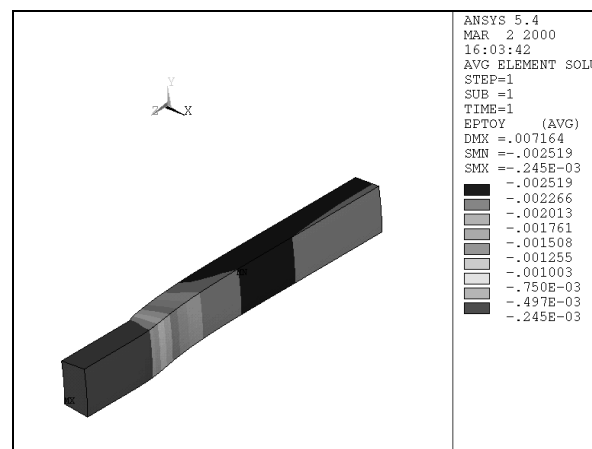
Figure MAF-49. Hoop Strain of the Scaled Pressure Vessel
