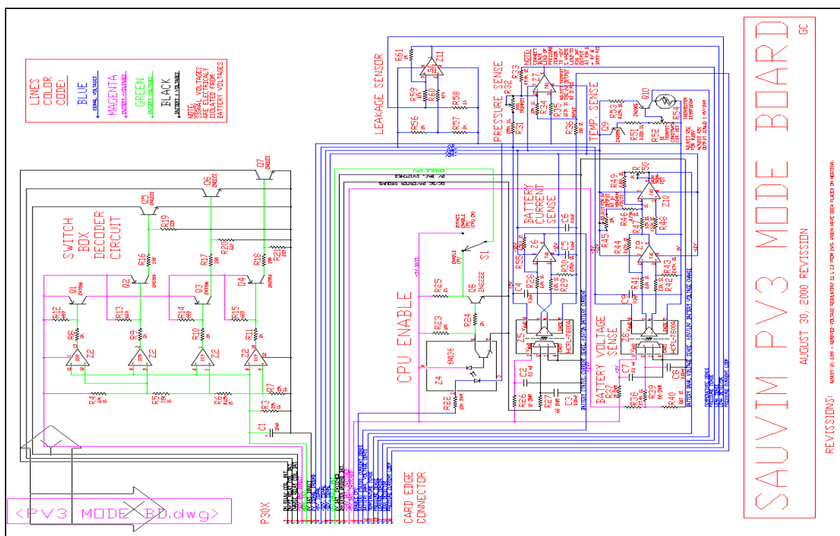
Figure MED-45: Pressure Vessel #3 Mode Board Circuit Schematic.
