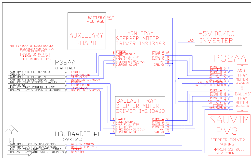
Figure MED-44: Pressure Vessel #3 Stepper Motor Control Circuit Schematic.
