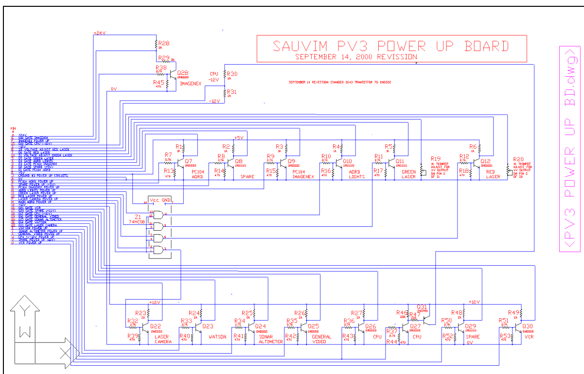
Figure MED-46: Pressure Vessel #3 Power-Up Board Circuit Schematic.
