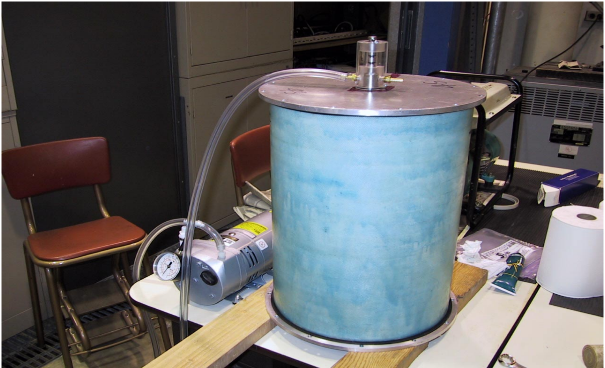
Photograph MED-13: Vacuum Bolt and Chuck in Use for Sealing Shallow Water Pressure Vessel.
