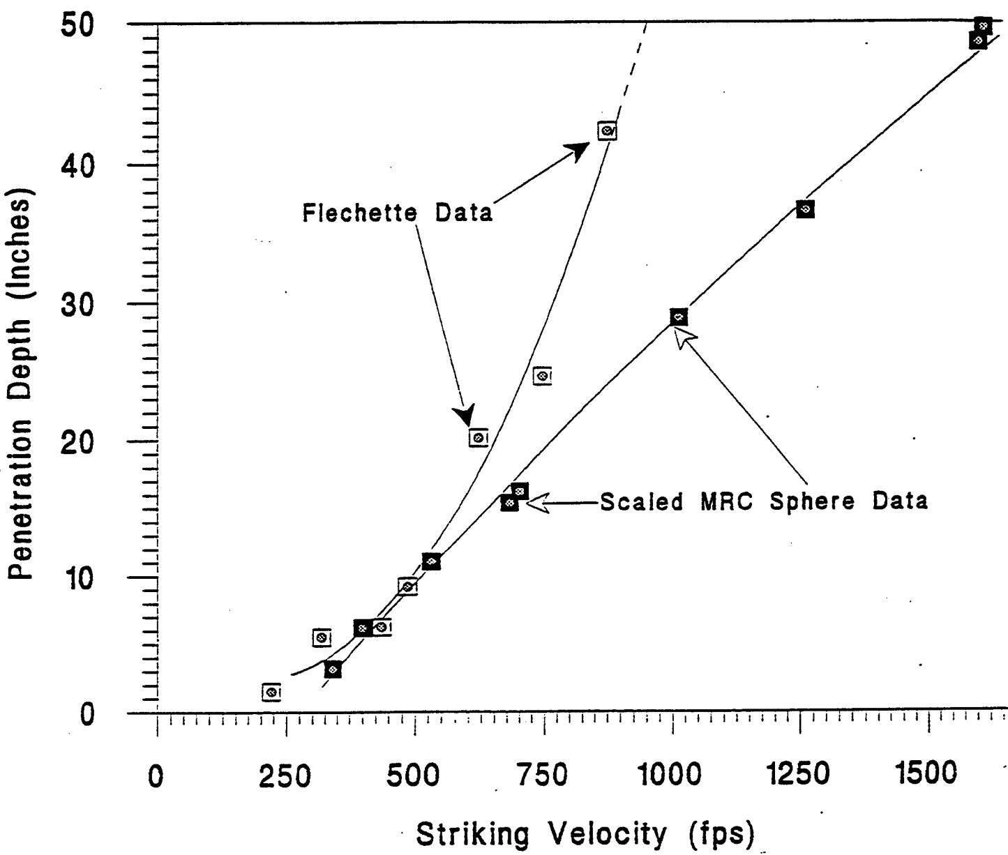
Figure 1. Comparison of an Equivalent Sphere and Flechette Depth of Penetration into 20% Ordnance Gelatin [Compiled from References 3 and 4].
