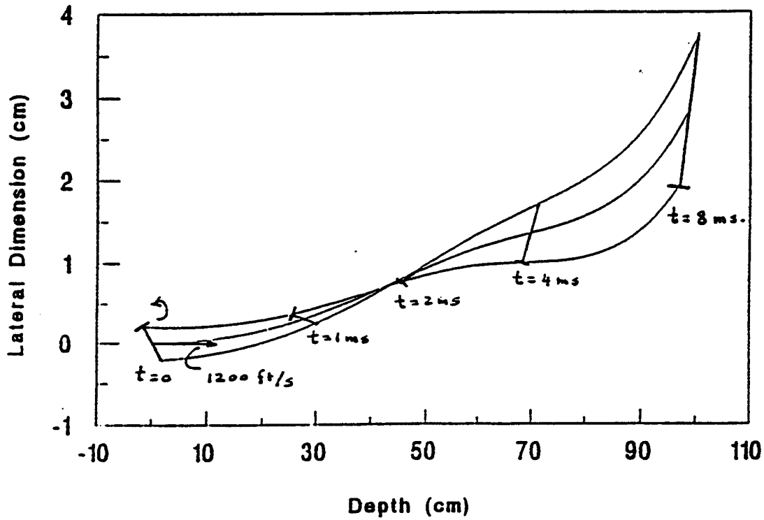
Figure 19. Flechette Motion for Different Angular Velocities at the Time of Target Entry
