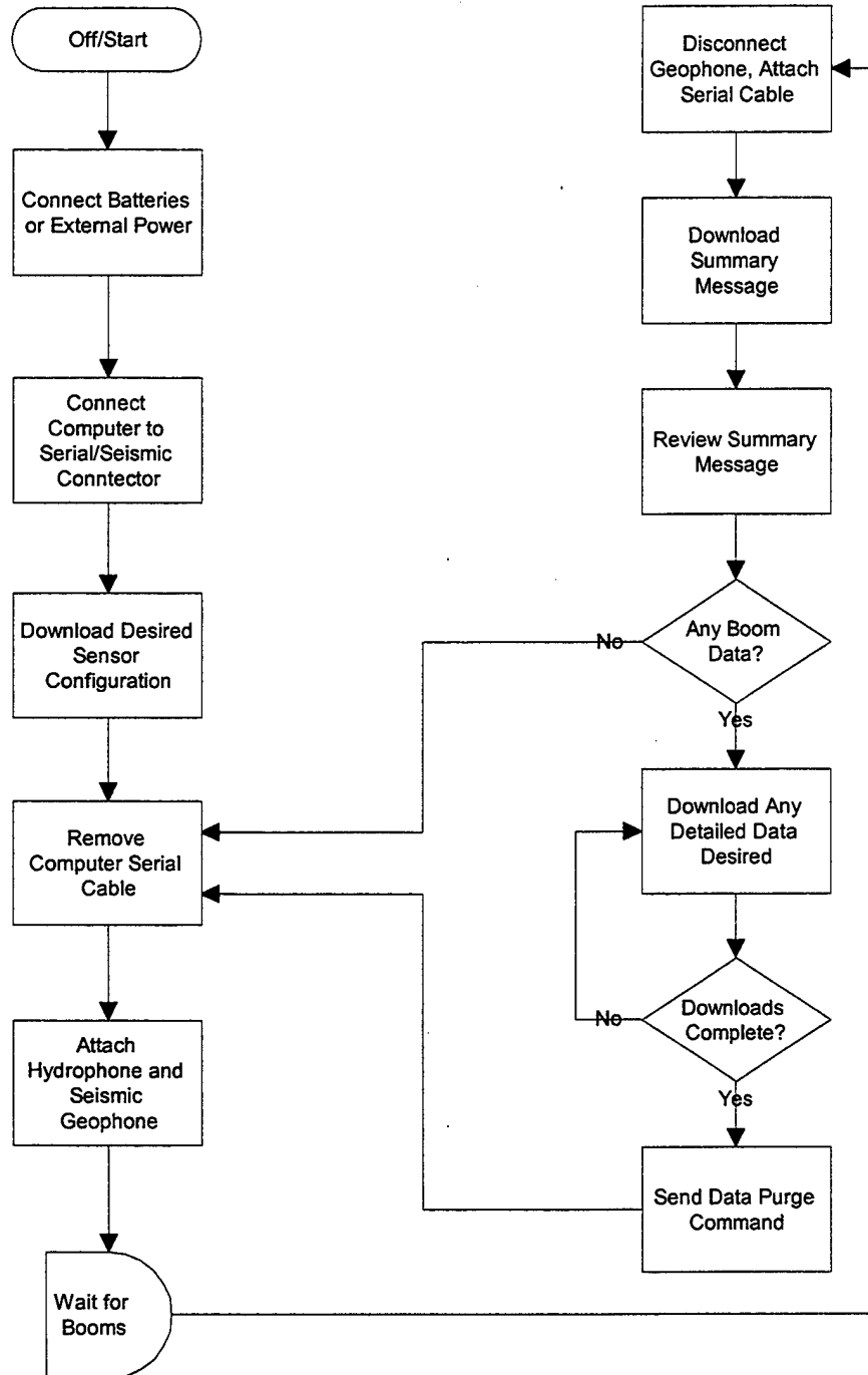
Figure 4 BAM Installation Flow Chart
