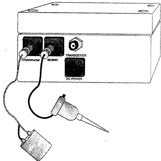
Figure 2 BAM Sensor and Transducer Connections
