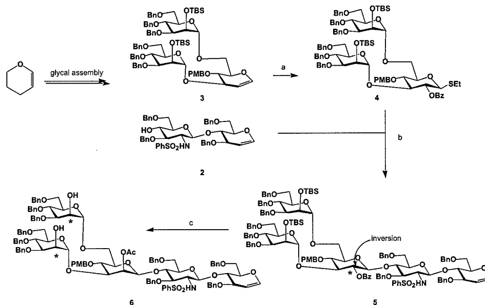
Figure 1. Core Pentasaccharide. a, 1. DMDO/CH 2 Cl 2 ; 2. EtSH/TFAA/CH 2 Cl 2 , 75% (two steps); 3. BzCl/Py/DMAP, 90% b, MeOTf/ CH 2 Cl 2 /DTBP, 75% ; c, 1. LiAlH 4 /THF/−20° C- 0° C; 2. Dess-Martin/ CH 2 Cl 2 /22° C; 3. L-selectride/THF/rt; 4. Ac 2 O/Py/DMAP/ CH 2 Cl 2 , 82% (four steps); 5. TBAF/THF, 77%
