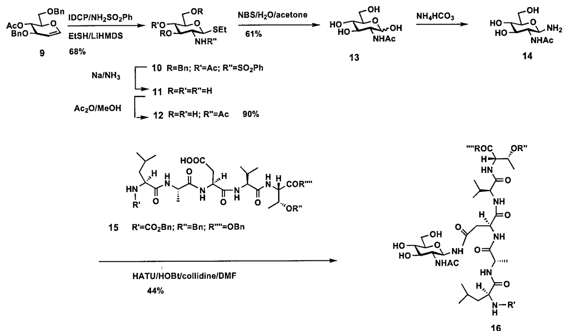
Scheme 2. Bn: benzyl; IDCP: bisdicollidine iodonium perchloride; LiHMDS = lithium hexamethyldisilazide; HATU: N -[(dimethylamino)-1 H -1,2,3-triazole[4,5- b ]-pyridin-1-ylmethylene]- N -methylmethanaminium hexafluorophosphate; HOBT: 1-hydroxy-1 H -benzotriazole hydrate; collidine = 2,4,6-trimethylpyridine.
