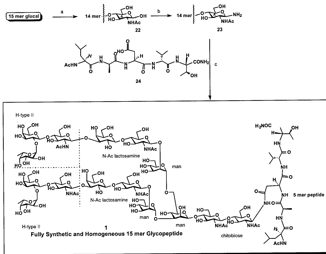
Figure 5. a.1. NH 2 CH 2 CH 2 NH 2 /EtOH; 2. Ac 2 O/Py/DMAP, 85% (two steps); 3. IDCP/NH 2 SO 2 Ph, 74%; 4. LiHMDS/AgOTf/THF/H 2 O, 63%; 5. Na/NH 3 /THF; 6. Ac 2 O/MeOH, 46% (two steps); b. NH 4 HCO 3 /H 2 O, 90%; c. Peptide 24 /HOBT/HBTU/DIEPA/DMSO, 20%
