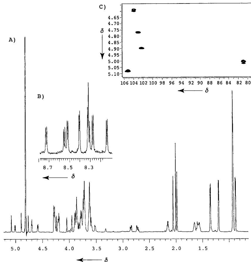
Figure 1. A) ^1H NMR (800 MHz) spectrum of 1 in D_2O at 20^\circ C and pH 3.7 (phosphate buffer). B) Section of the ^1H NMR spectrum of 1 in H_2O at 5^\circ C and pH 3.5 (phosphate buffer) showing the secondary NH signals of amides from the peptide backbone, side chain, and GlcNAc sites. The protons of the terminal carboxamide (not shown) are observed slightly upfield of this region. C) The anomeric region of the ^1H - ^{13}C HMQC spectrum at 800 MHz of 1 in D_2O at 20^\circ C and pH 3.7 (phosphate buffer). The GlcNAc anomeric sites at \delta = 4.58 and 5.01 ( ^1H ) are clearly distinguished by their larger ^1H couplings.
