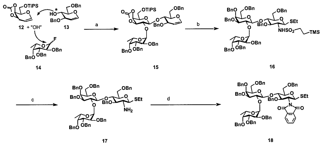
Figure 3. Synthesis of Wing trisaccharide: a, 1. DMDO/ \text{CH}_2\text{Cl}_2 ; 2. \text{ZnCl}_2 ; 3. \text{SnCl}_2/\text{AgOTf}/\text{DTBP}/\text{CH}_2\text{Cl}_2 , 50%; b, 1. TBAF/THF; 2. \text{BnBr}/\text{NaH}/\text{DMF} , 81%; 3. IDCP/ \text{PhSO}_2\text{NH}_2 ; 4. \text{EtSLi}/\text{DMF}/-40^\circ\text{C} - 0^\circ\text{C} 75%; c, \text{CsF}/\text{DMF}/100^\circ\text{C} , 5 days 65%; d, 1. Phthalic anhydride/ \text{Py}/22^\circ\text{C} ; 2. \text{Ac}_2\text{O} , 97%
