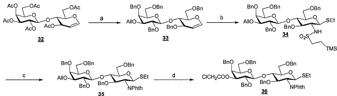
Figure 7. Lactosamine Building Block. a, 1. \text{NH}_3/\text{MeOH} ; 2. \text{Bu}_2\text{SnO}/\text{benzene} ; 3. Allyl bromide/ \text{Bu}_4\text{NBr} ; 4. \text{BnBr}/\text{NaH}/\text{DMF} , 50%; b, 1. IDCP/ \text{TMSCH}_2\text{CH}_2\text{SO}_2\text{NH}_2 , 83%; 2. \text{EtSH}/\text{LiHMDS}/\text{DMF} , 85%; c, 1. \text{CsF}/\text{DMF} , 90^\circ\text{C} , 94%; 2. Phthalic anhydride/ \text{Py}/\text{rt} , 3. \text{Piv}_2\text{O} or \text{Ac}_2\text{O} , 100%; d, 1. \text{Ph}_3\text{RuCl}/\text{DABCO}/\text{THF} ; 1N \text{HCl} , 74%; 2. (\text{ClCH}_2\text{CO})_2\text{O}/\text{DTBP}/\text{Cat} . DMAP/ \text{DCM} , 97.3%
