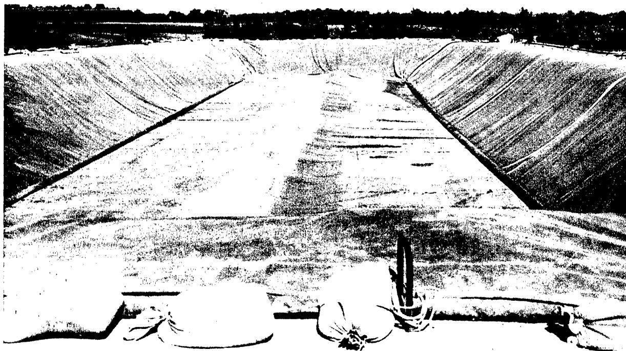
Figure 4. 10,000-barrel fuel storage reservoir. The reservoir contained 4500-bbls of fuel when the photograph was made.
