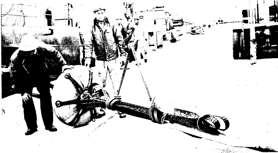
Figure 1. 50K experimental explosive emplaced anchor assembly of early design readied for loading on Navy vessel for test firing.
