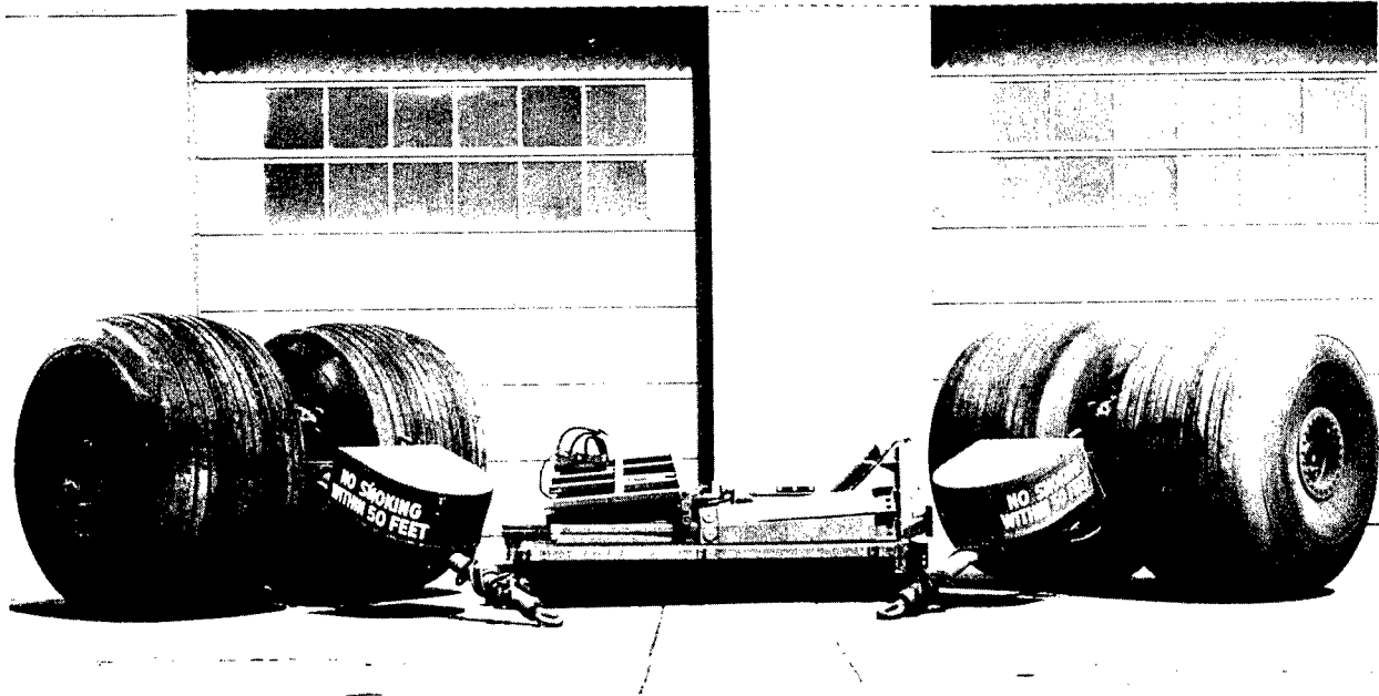
Figure 23. Rolling Liquid Transportation Trailer Kit and Two (2) (ea) 1000-gallon T-3 Rolling Liquid Transporters.
