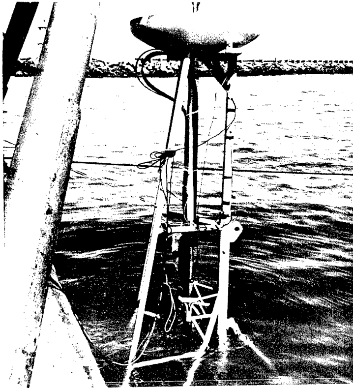
Figure 2. Refined 50K explosive emplaced anchor assembly in test fixture ready for lowering and emplacement at USNCEL, Port Hueneme, California.
