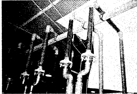
Figure 3. 1998 photograph of fiberglass pipe discoloration for 13V1001 (starboard side).
