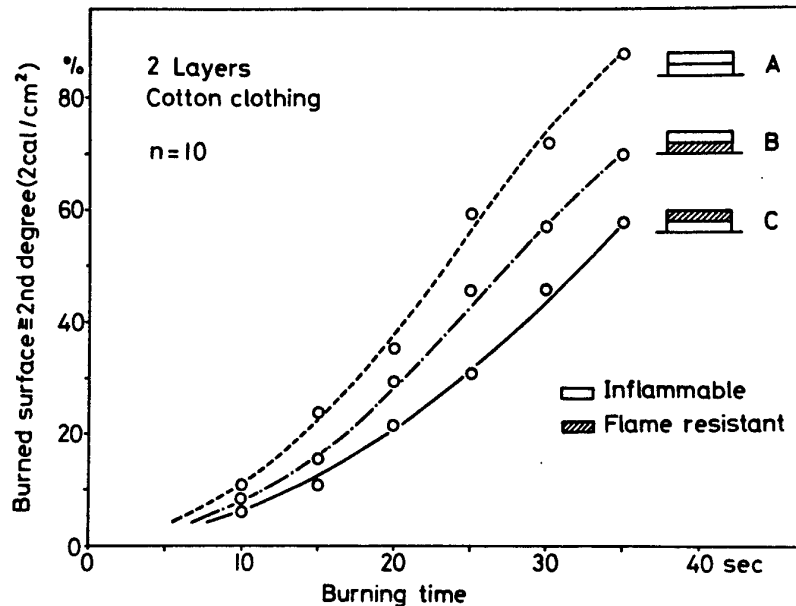
Fig. 2: Percentage of burned surface \leq 2 nd degree as a function of burning time (4). Model experiments with a two-layer work clothing of cotton; outside a 280 \text{ g/m}^2 twill, inside a 230 \text{ g/m}^2 tricot.
