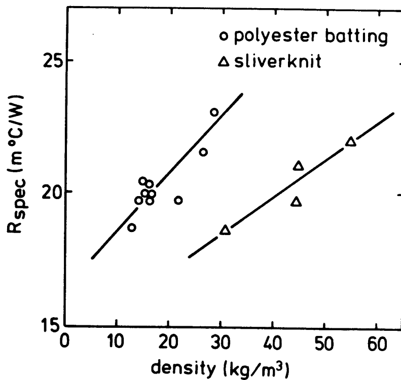
Fig. 2. Dependency of specific insulation on density for two types of insulative material (Adopted from Van Bruggen et al., 1984.)
