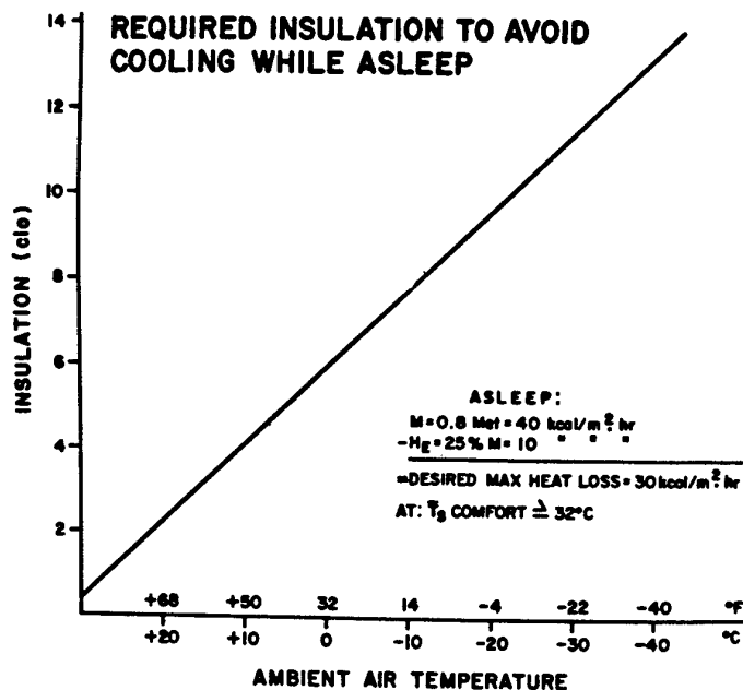
Fig 1. Required insulation to avoid cooling while asleep
