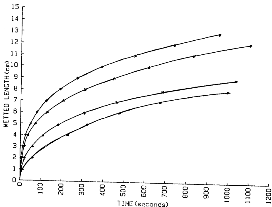
Fig. 1: Wetted length vs. time from vertical wicking trial
