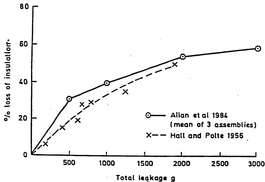
Fig. 3. Percent loss of insulation plotted against leakage.
