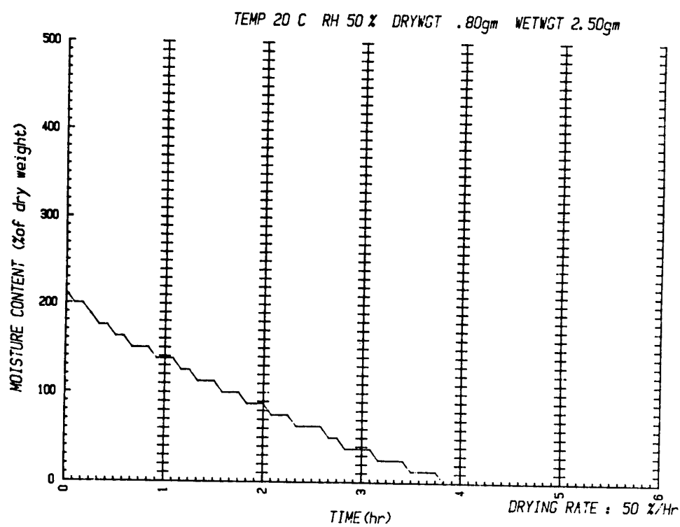
Fig. 2. Moisture content as a function of drying rate
