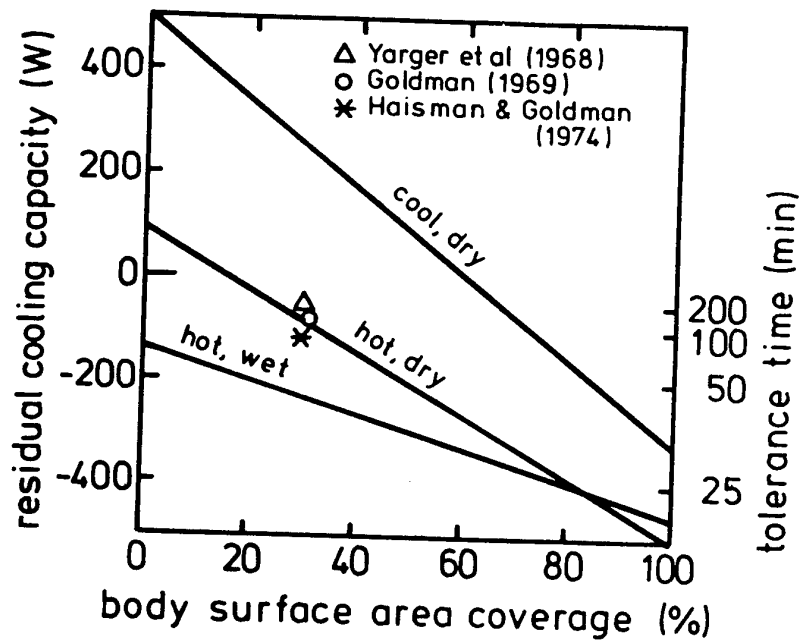
Fig. 5. Calculated residual cooling capacity and tolerance times for three hypothetical climates, in relation to % body surface area covered by body armour (for additional conditions see text). Data of 3 authors for the hot, dry climate are also known.
