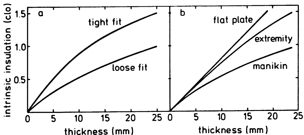
Fig.2 a. Calculated intrinsic insulation as a function of assembly thickness. b. Calculated insulation of the same material on a flat plate, as a sleeve and on a manikin (for loose fit).
