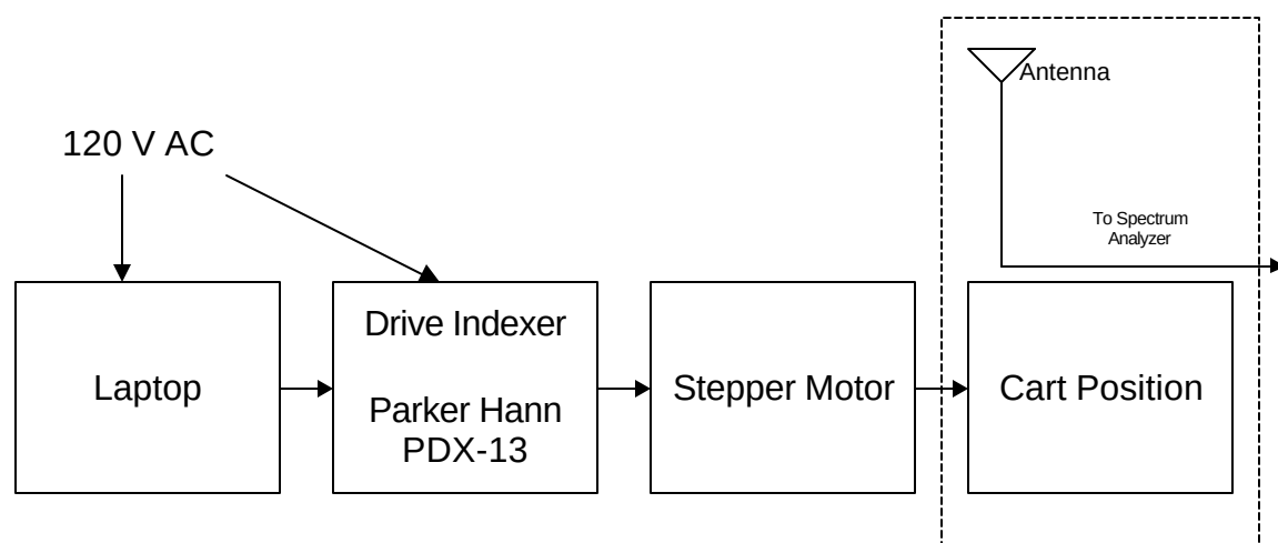
Figure 6 Antenna Positioning System Block Diagram.
