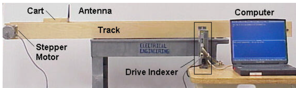
Figure 7 Antenna Positioning System.
