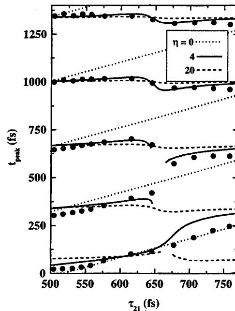
FIG. 8. Comparison between the measured (solid dots) and the simulated time t_p at which each peak in the lh-hh oscillations occurs as a function of \tau_{21} for three values of the EID parameter: \eta=0 (dotted line), 4 (solid line), and 20 meV (dashed line).
