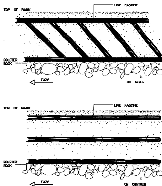
Figure 7. LF configuration showing fascine angle along bank face
