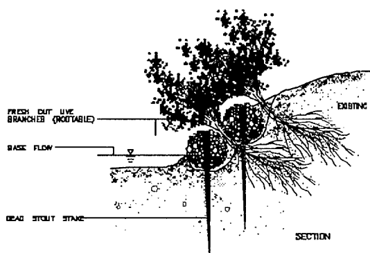
Figure 8. Live siltation construction with stacked LFs
