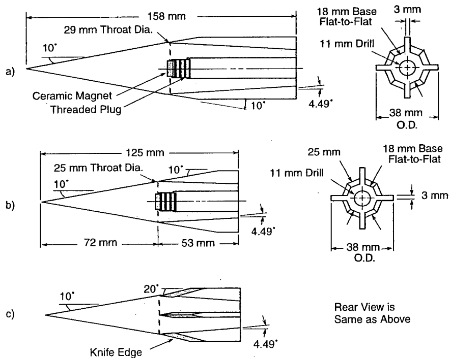
Fig. 8 Solid Mg alloy projectiles: a) standard 29 mm throat. b) reduced 25 mm throat. c) reduced 25 mm throat with knife-edged fins and 20° fin rake angle.
