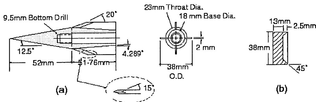
Fig. 3. a) Generalized Ti alloy projectile design. b) Obturator design.
