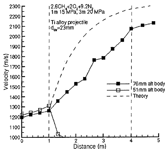
Fig. 6. Results from two-stage 15/20 MPa experiments.
