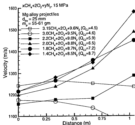
Fig. 8 Results of propellant composition variation using 25 mm throat Mg projectiles.
