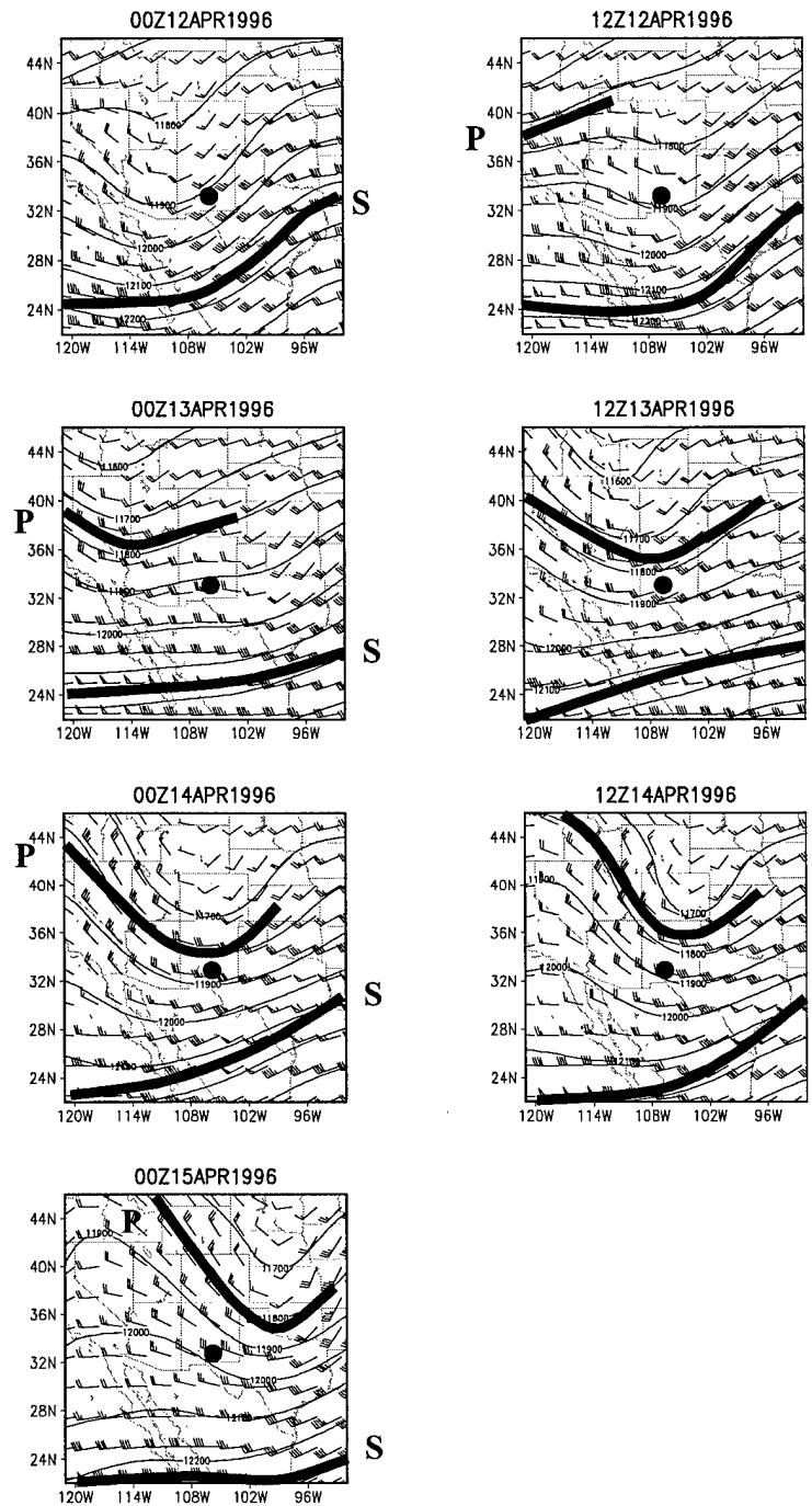
Figure 19 Case study 2 NCEP/NCAR 200 hPa analysis. The polar (P) and subtropical (S) jet cores are denoted by solid line and the WSMR radar by dot. Geopotential height is in meters MSL and wind barbs are in meters per second.
