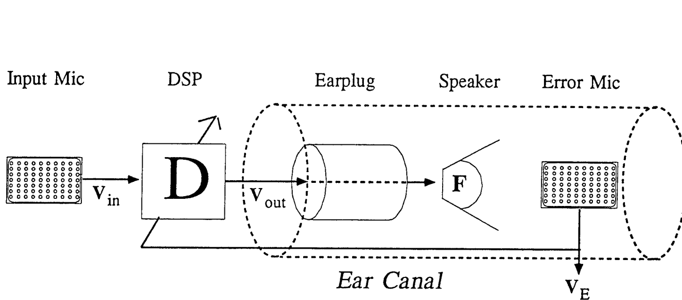
Figure 1. Schematic Depiction of ANR Earplug For Feed Forward Approach
