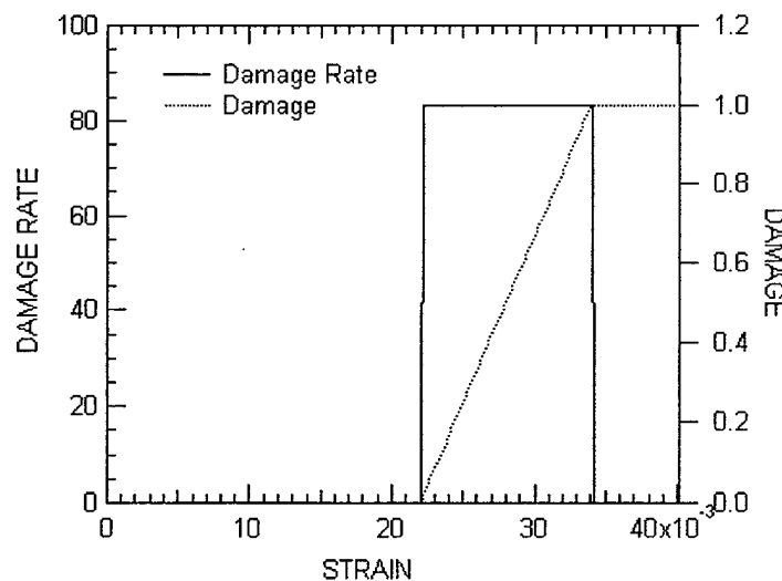
FIGURE 63. FIBER DAMAGE AS A FUNCTION OF STRAIN
