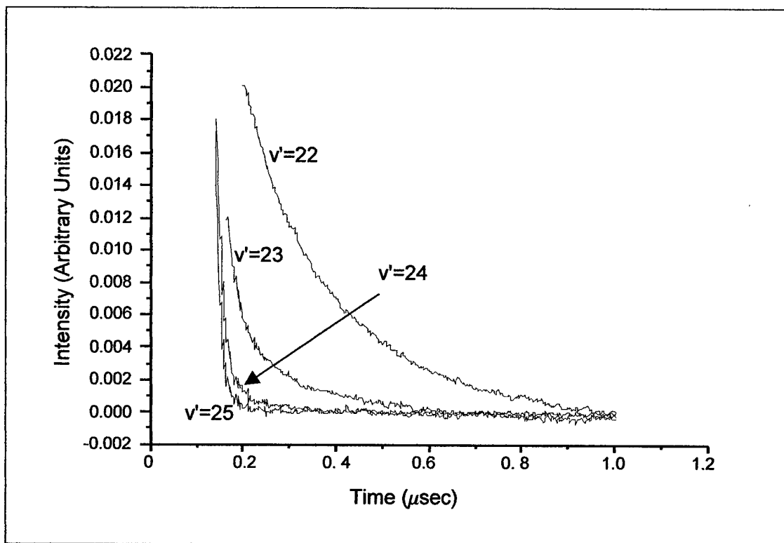
Figure 3.10. Fluorescence Decay Curves for Helium Buffer Gas, ~3000mTorr, v'=22 through v'=25 .
