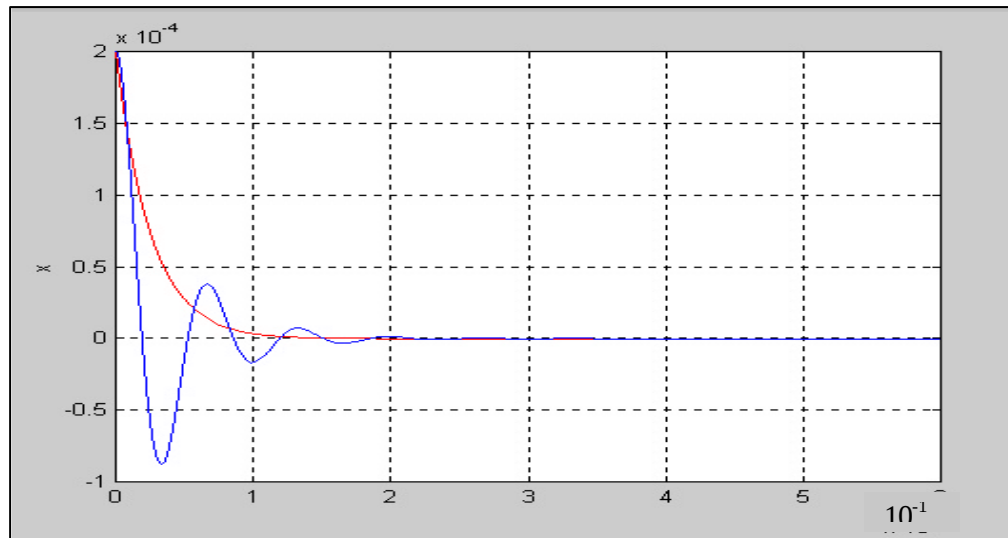
Fig. 11: Desired input x(t) (red line) and output response (blue line) without NN controller
