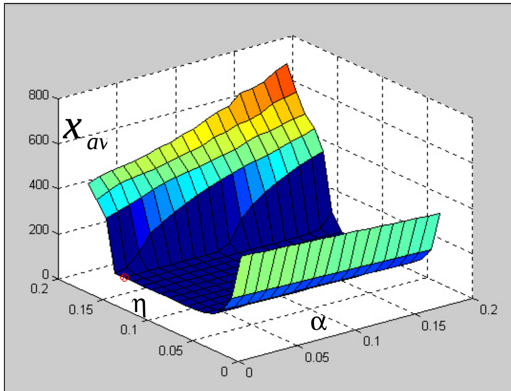
Fig. 9: Average error x_{av} function of the parameters \alpha and \eta
