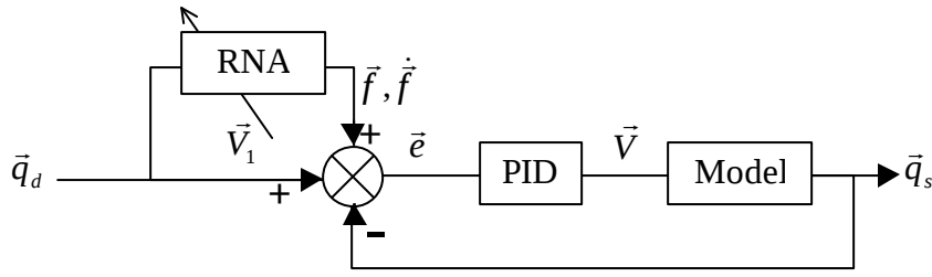
Fig. 8: Condensed neural network control loop
