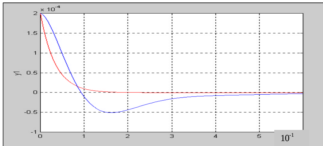
Fig. 12: Desired input y_1(t) (red line) and output response (blue line) without NN controller
