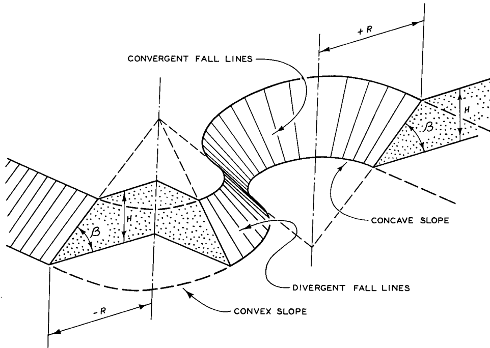
Fig. 15. Dimensions of slope curved in plan
