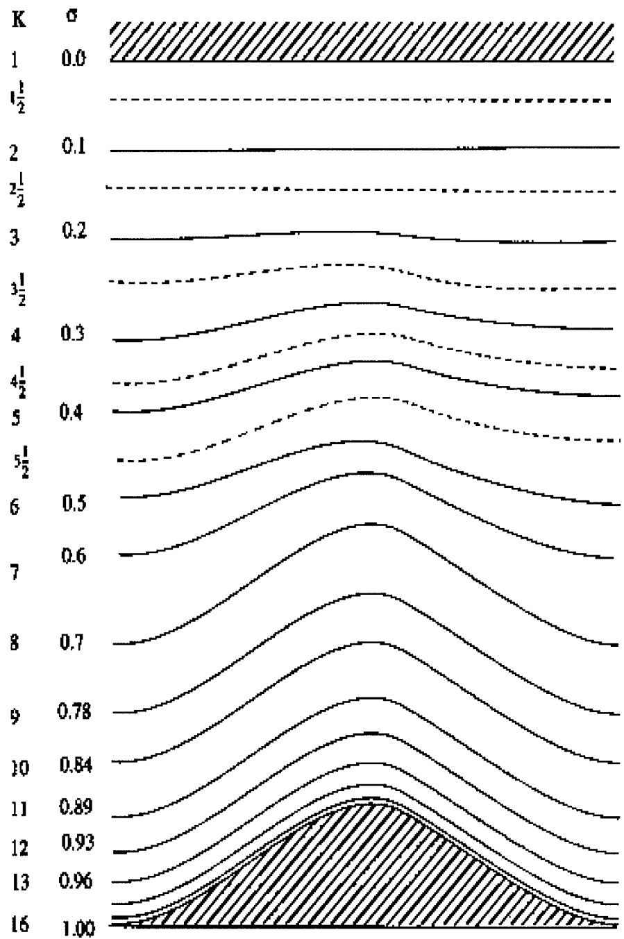
Figure 2-4. Schematic representation of the vertical structure of the MM5 model. Adapted from MMMD/NCAR (MMMD/NCAR 2000).
