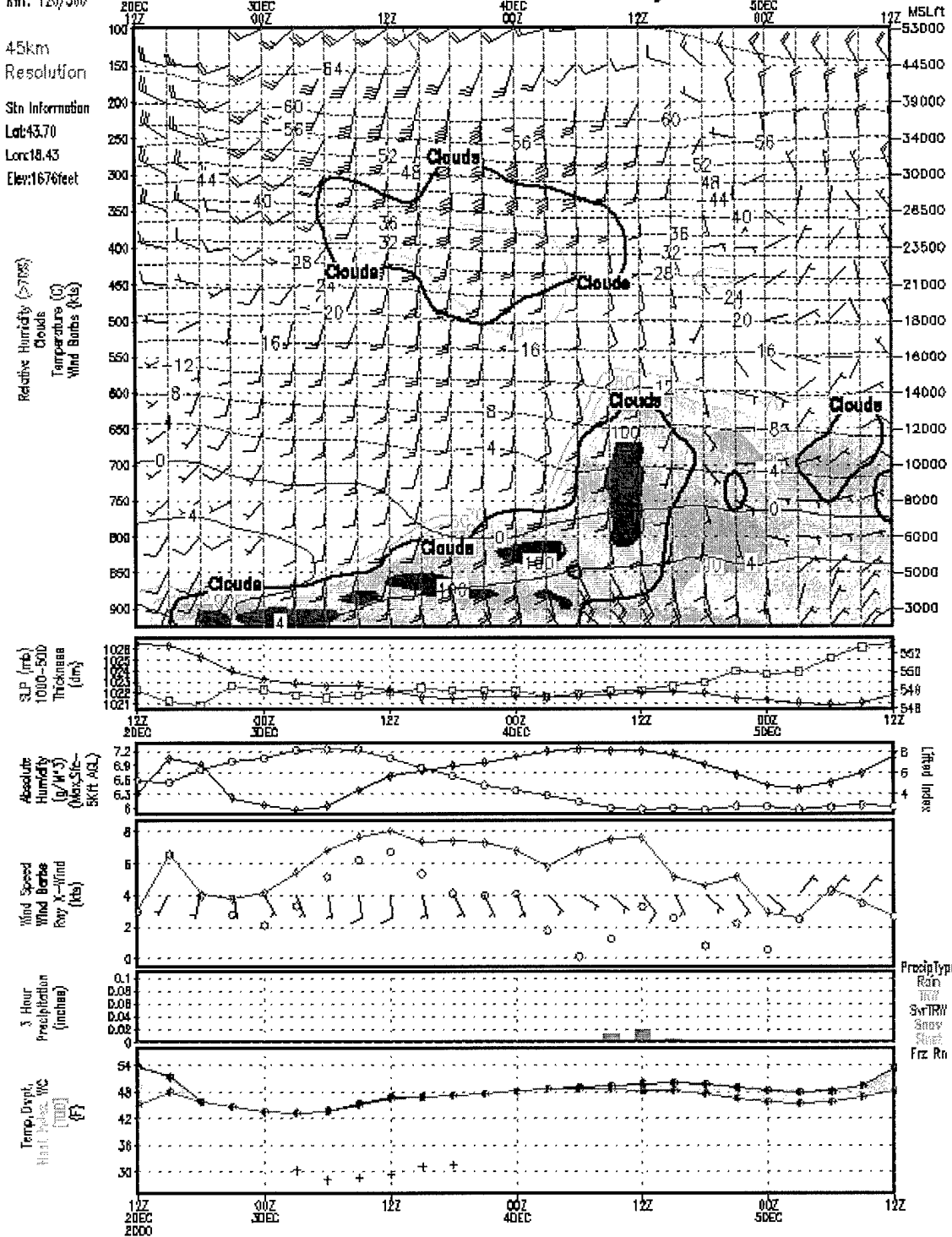
Figure 3-1. Meteogram for Sarajevo, Bosnia.
