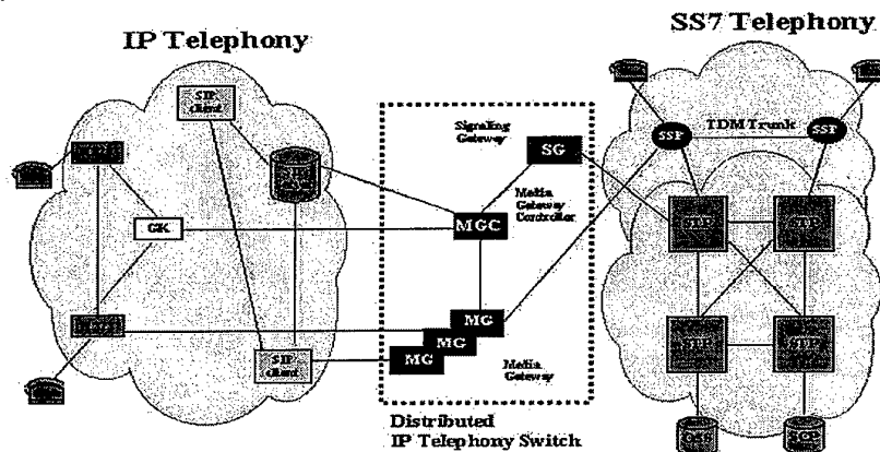
Figure 9 Gateway Approach
