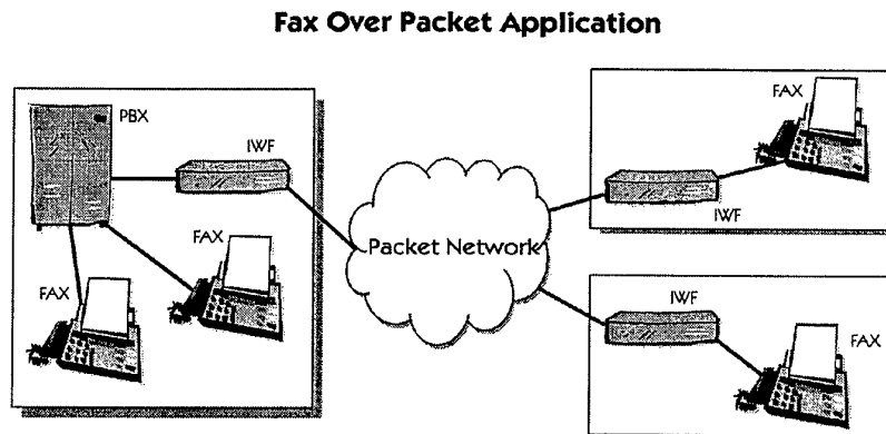
Figure 10 Fax over IP
