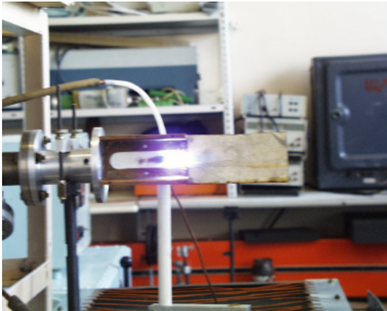
Fig.5. External PAC. Streamer HF discharge in metal section (lateral wall is absent). Propane injection through pylon. M=0,8-1,2; P_{st} \sim 1 Bar, T_o \sim 300\text{K}
