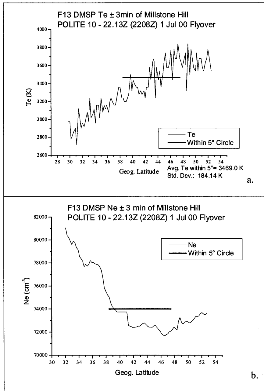
Figure 32. Case M10-3, DMSP Plots of (a) T_e and (b) n_e Showing Support for a Mid-Latitude Trough around 46°N Geographical Latitude.
