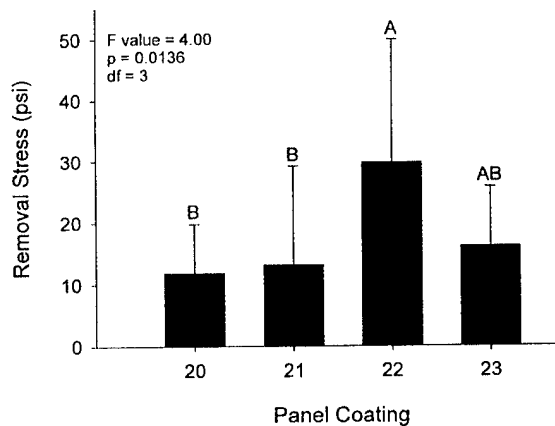
Figure 2. Forces to remove Hydroïdes elegans from select panels immersed at the Pacific Test Site.
