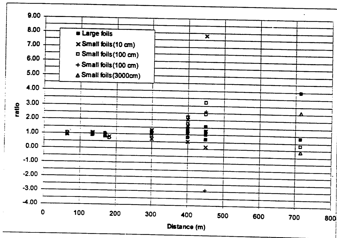
Figure 2-9. Sulfur activation calculation to measurement ratio.
