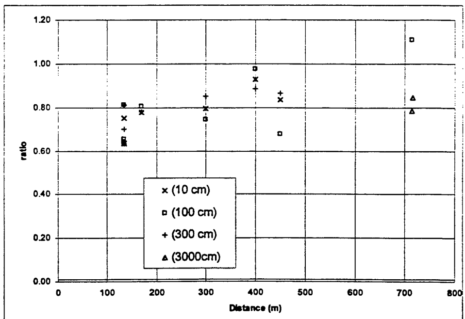
Figure 2-18. Al 2 O 3 TLD gamma ray dose calculation to measurement ratio.
