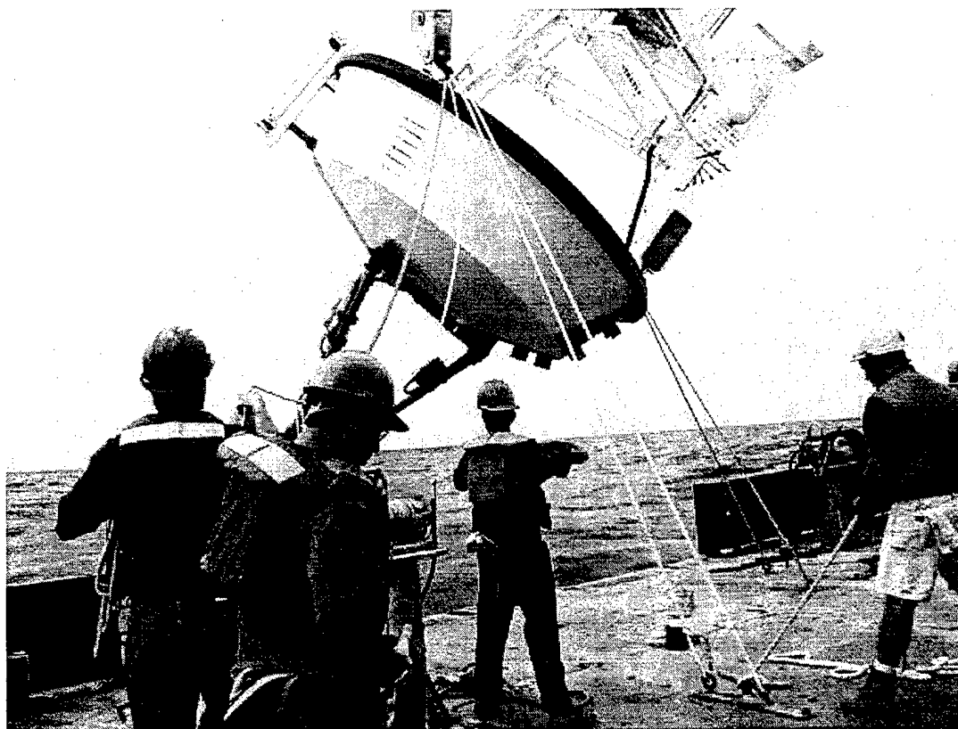
Figure 38: Three slip lines rigged on the discus to maintain constant swing control during the lift.
