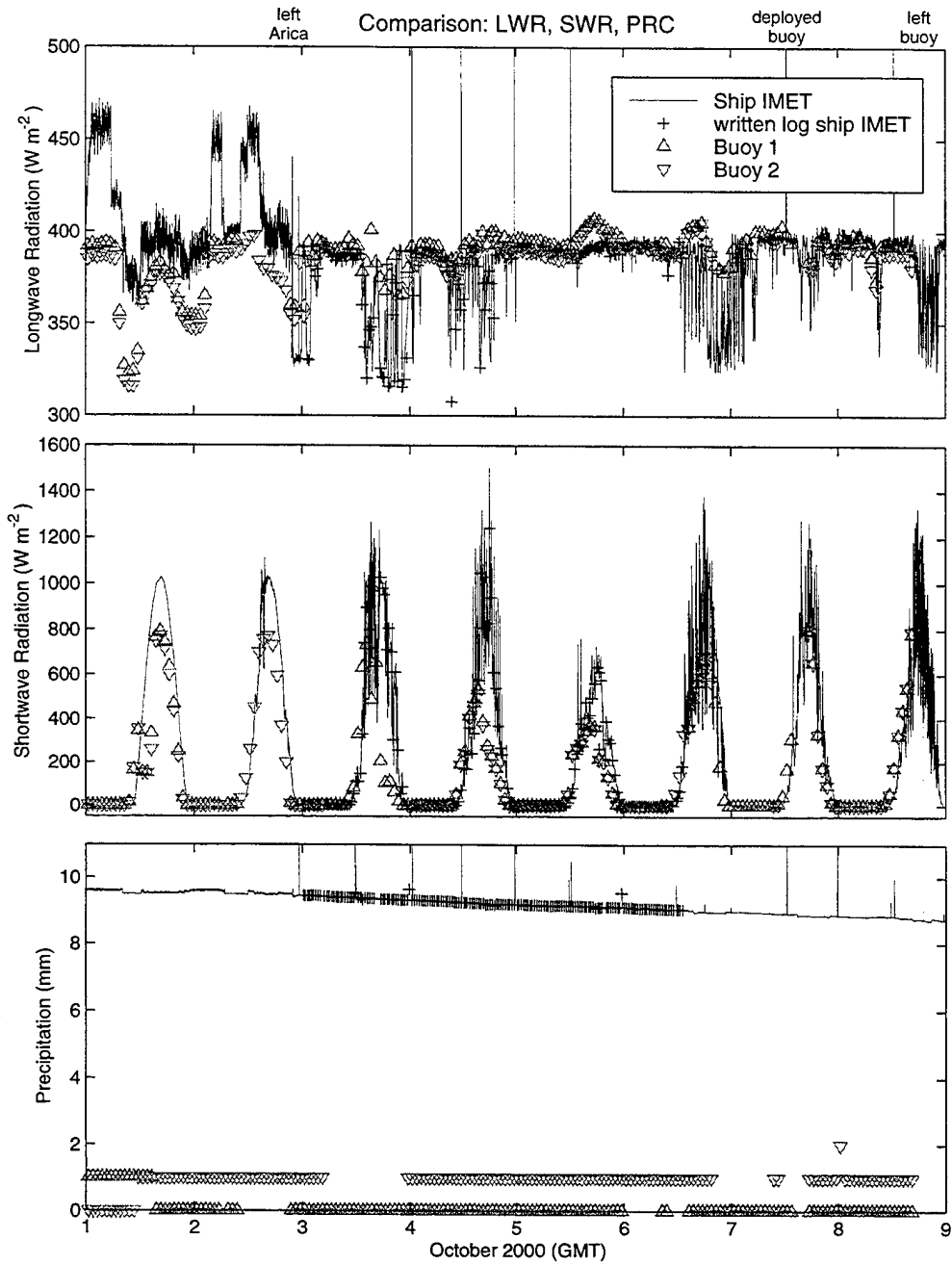
Figure 16: Overplots of Ship IMET, Buoy IMET, handheld, and written ship logs longwave and shortwave radiation, and precipitation.
