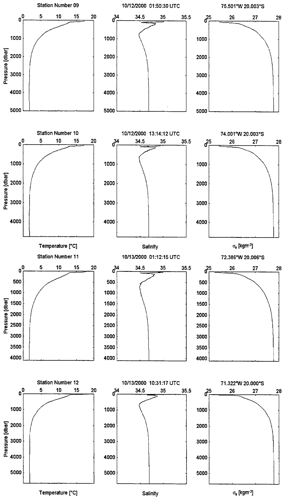
Figure 21: CTD stations nine, ten, eleven and twelve.
