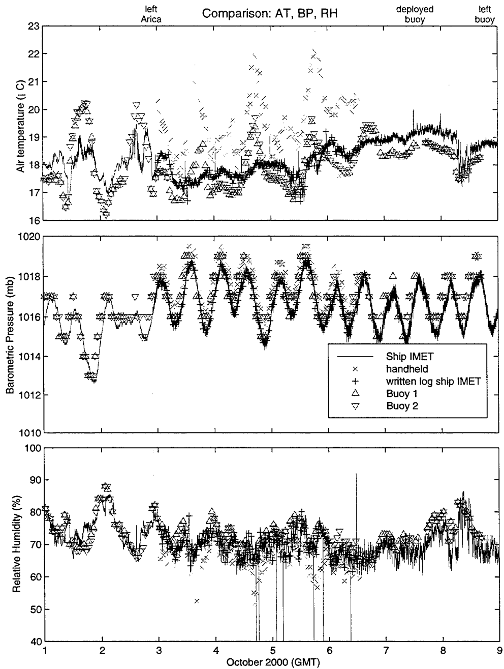
Figure 14: Overplots of Ship IMET, Buoy IMET, handheld, and written ship logs of air temperature, barometric pressure, and relative humidity.
