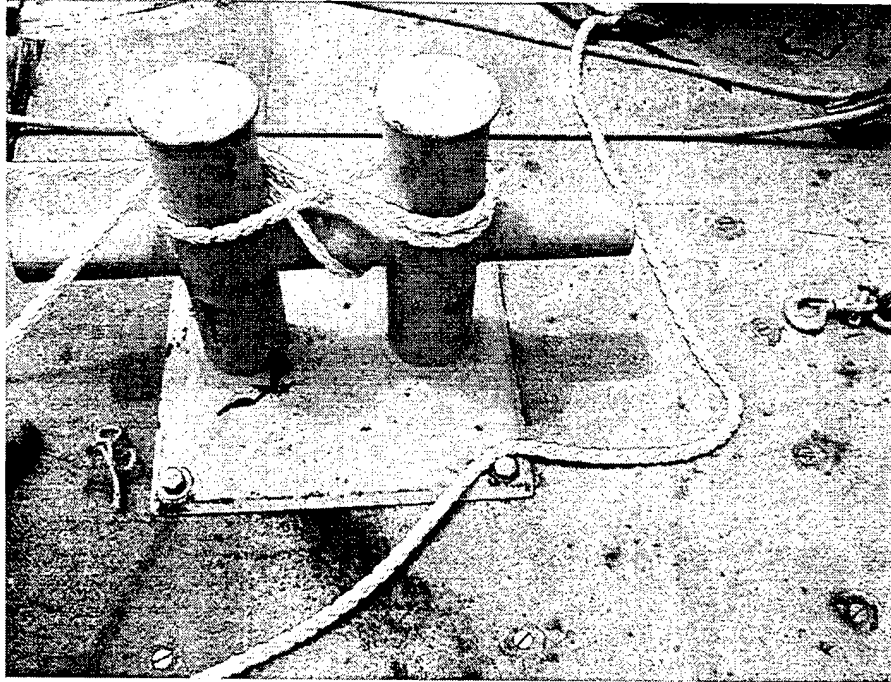
Figure 40: Details how this line was reeved around the H-bit
