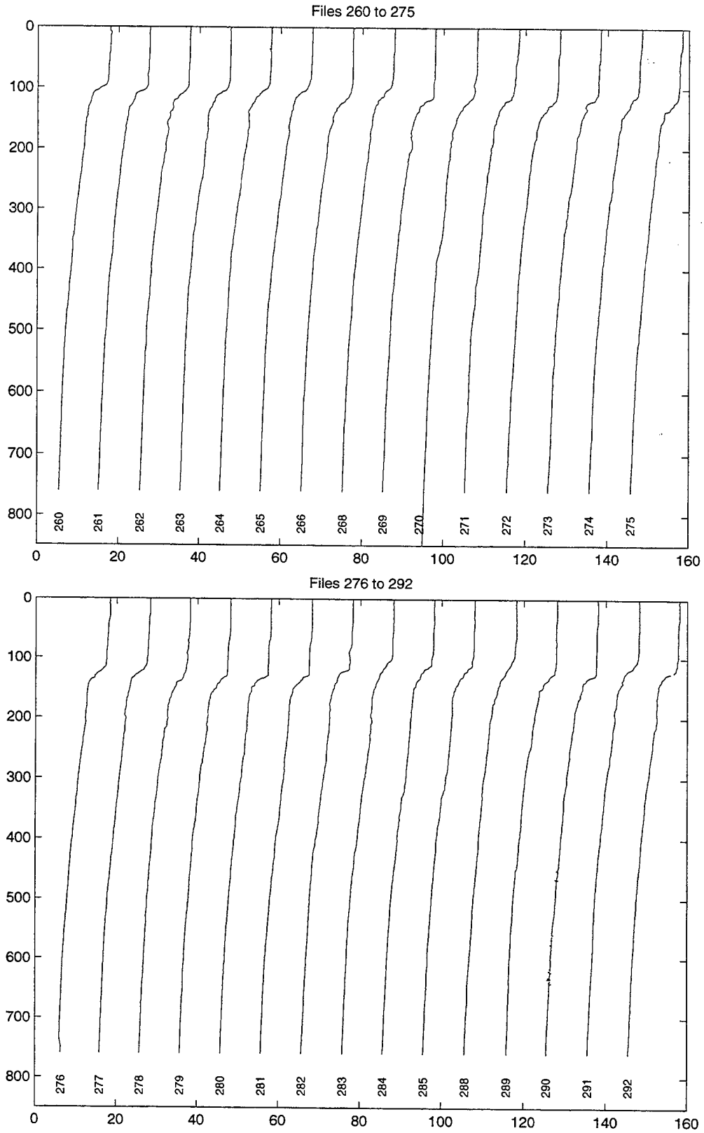
Figure 30: Profile plots of the XBT station data, separated by 10°C.
