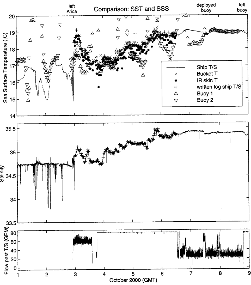
Figure 15: Overplots of Ship IMET, Buoy IMET, handheld, and written ship logs of sea surface temperature and salinity from the ship's thermosalinograph. The last plot is of the flow past the thermosalinograph, verifying that the pump was on while on station.
