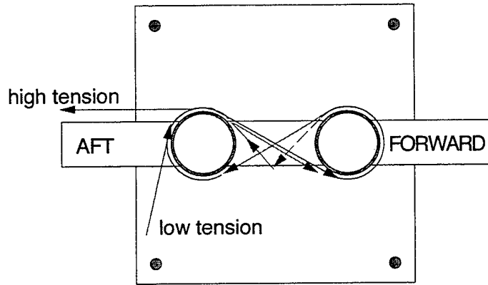
H-Bit line fair lead detail
