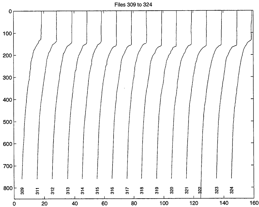
Figure 31: Profile plots of the XBT station data, separated by 10°C.
