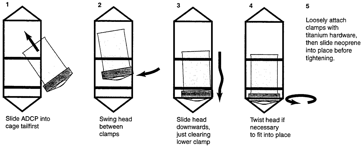
Figure 36: Diagram describing insertion of RDI ADCP into cage.
