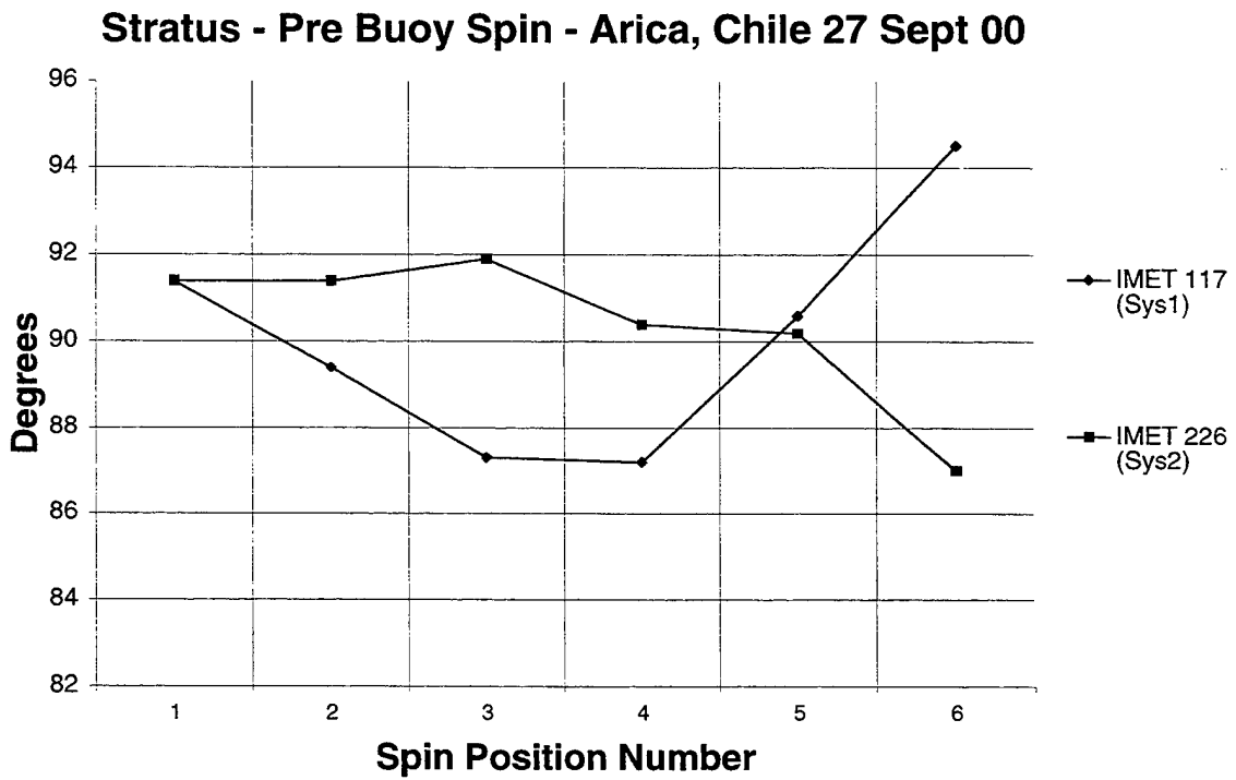
Figure 8: Spin data plot for Arica, Chile.
