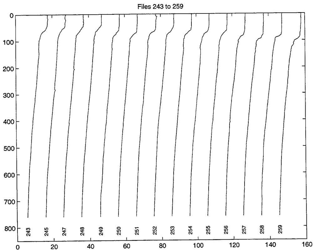
Figure 29: Profile plots of the XBT station data, separated by 10°C.
