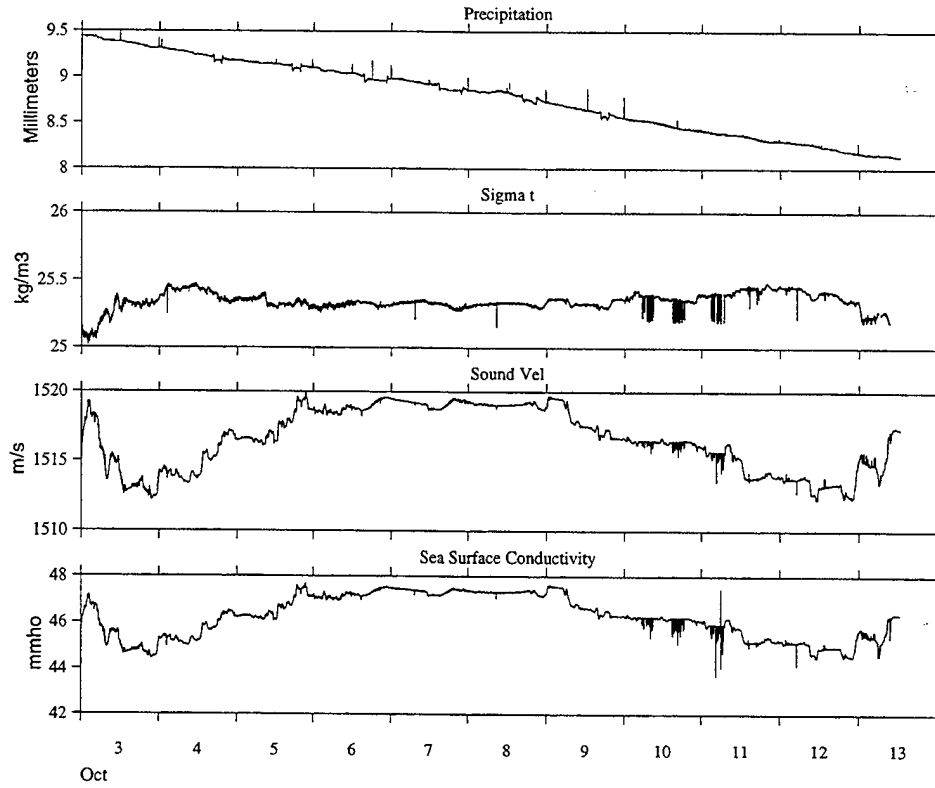
Figure 50: Precipitation, Sigma t, Sound velocity, and Sea surface conductivity.
