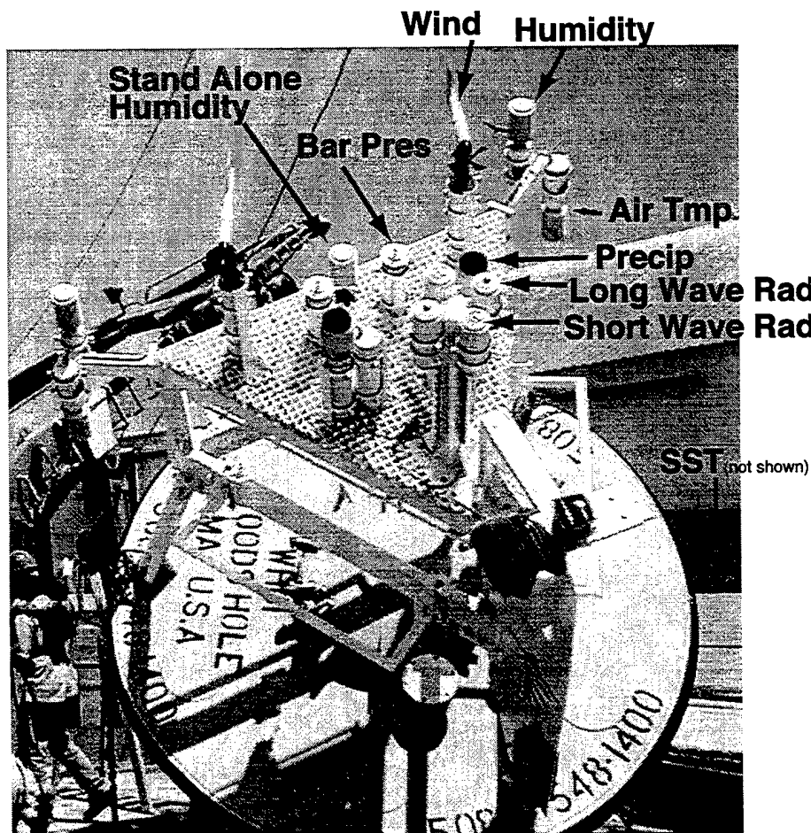
Figure 4: STRATUS 1 Buoy IMET Towertop.
