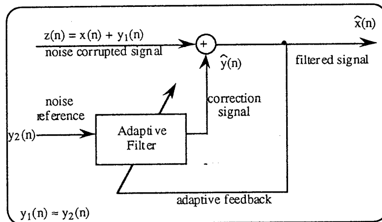
Fig. 4.1 Noise cancelling approach (after [Juan91]).
