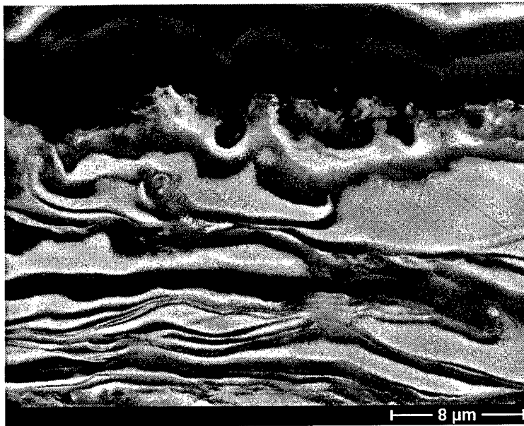
Figure 28: SEM-secondary electron image of cold-rolled Al 66 Pd 34 at a strain of \epsilon = -8.9
