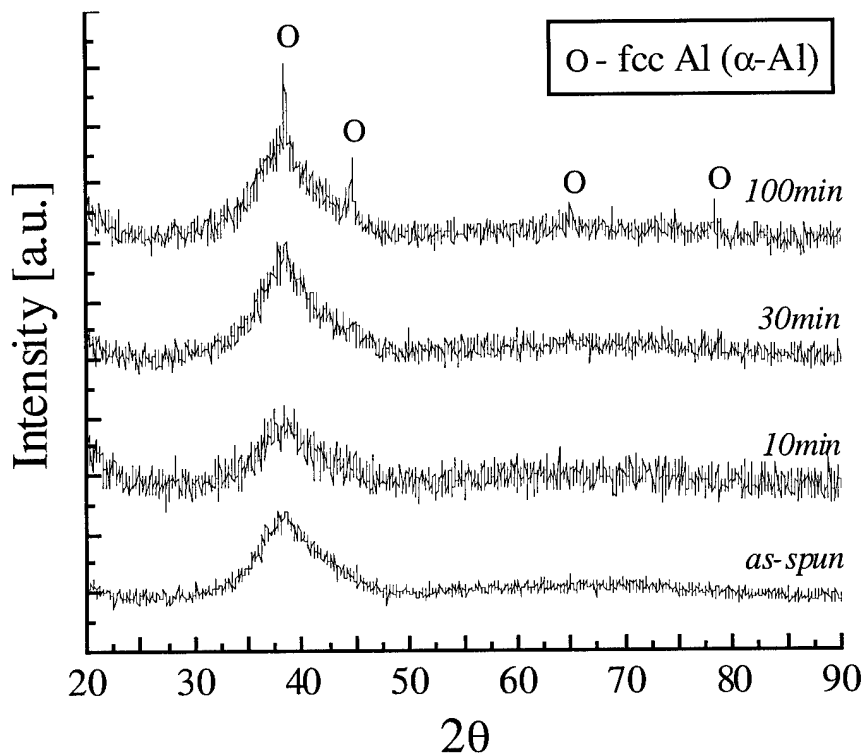
Figure 7. X-ray diffraction (XRD) traces of the as-spun Al_{88}Y_7Fe_5 ; and ribbon samples that were previously isothermally annealed at 245^\circ C for 10; 30 and 100minutes.
