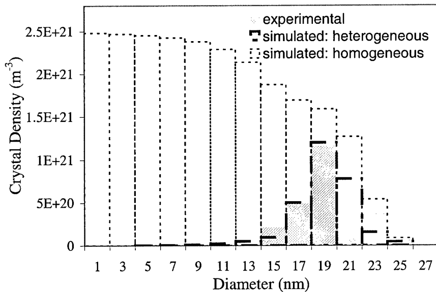
Figure 10. The size distribution of Al nanocrystals for the \text{Al}_{88}\text{Y}_7\text{Fe}_5 melt-spun sample isothermally annealed at 245°C for 10 minutes plotted with the simulated distribution for homogeneous and heterogeneous nucleation.
