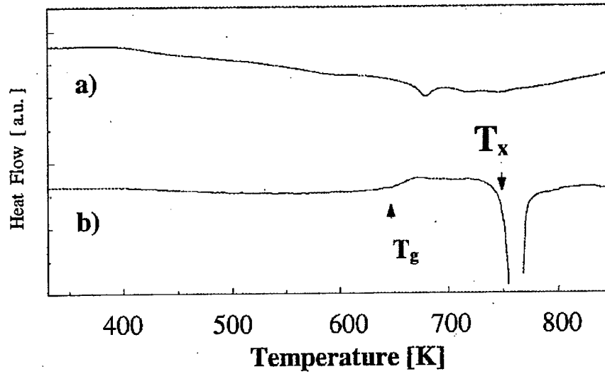
Figure 15. DSC continuous heating traces of Zr_{68}Ni_9Al_6Cu_{18} at 40K/min after (a) 40 and (b) 120 rolling passes. A glass transition at 647K is present in curve (b) and this T_g is close to that measured on the cast bulk metallic glass with the same composition.
