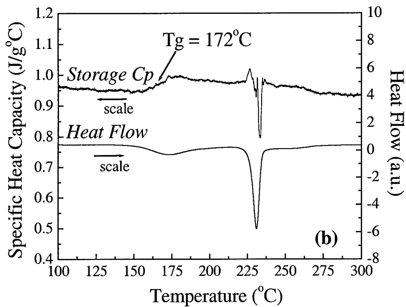
Figure 5. Results of the modulated-temperature DSC on the as-spun sample of (a) \text{Al}_{88}\text{Y}_7\text{Fe}_5 and (b) \text{Al}_{92}\text{Sm}_8 . The glass transition temperatures ( T_g ) were obtained as 258^{\circ}\text{C} in (a) and 172^{\circ}\text{C} in (b), respectively.
