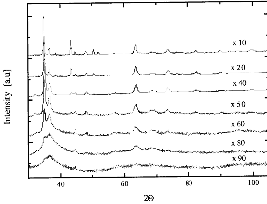
Figure 14. XRD of Zr_{68}Al_6Ni_9Cu_{18} after different number of rolling passes
