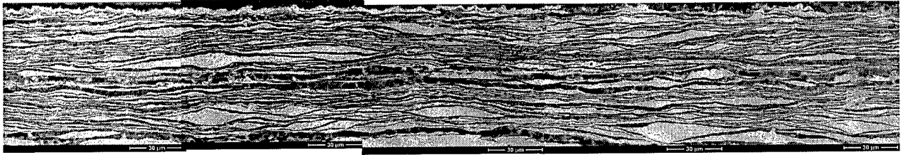
Figure 27: SEM-secondary electron images of cold-rolled Al 66 Pd 34 at a strain of \epsilon = -8.9
