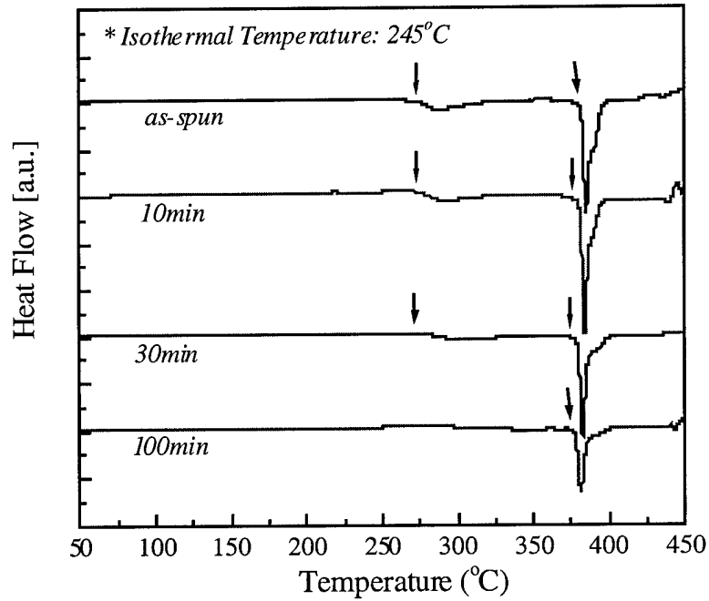
Figure 9. The continuous heating DSC traces on the \text{Al}_{88}\text{Y}_7\text{Fe}_5 melt-spun samples that were isothermally annealed at 245°C for 10, 30, and 100 minutes.
