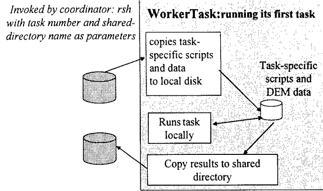
Figure 5 : Worker processing to run a task
