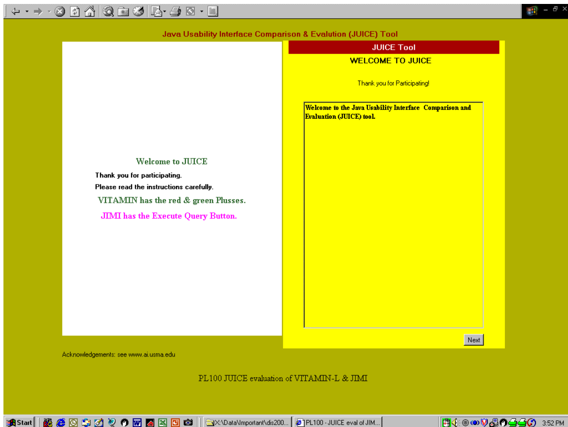
Figure 29 JUICE Welcome
