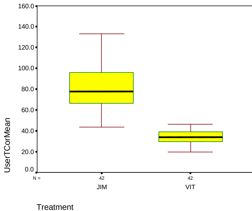
Figure 47 Time to Correctly Answer Tasks Box-plot
