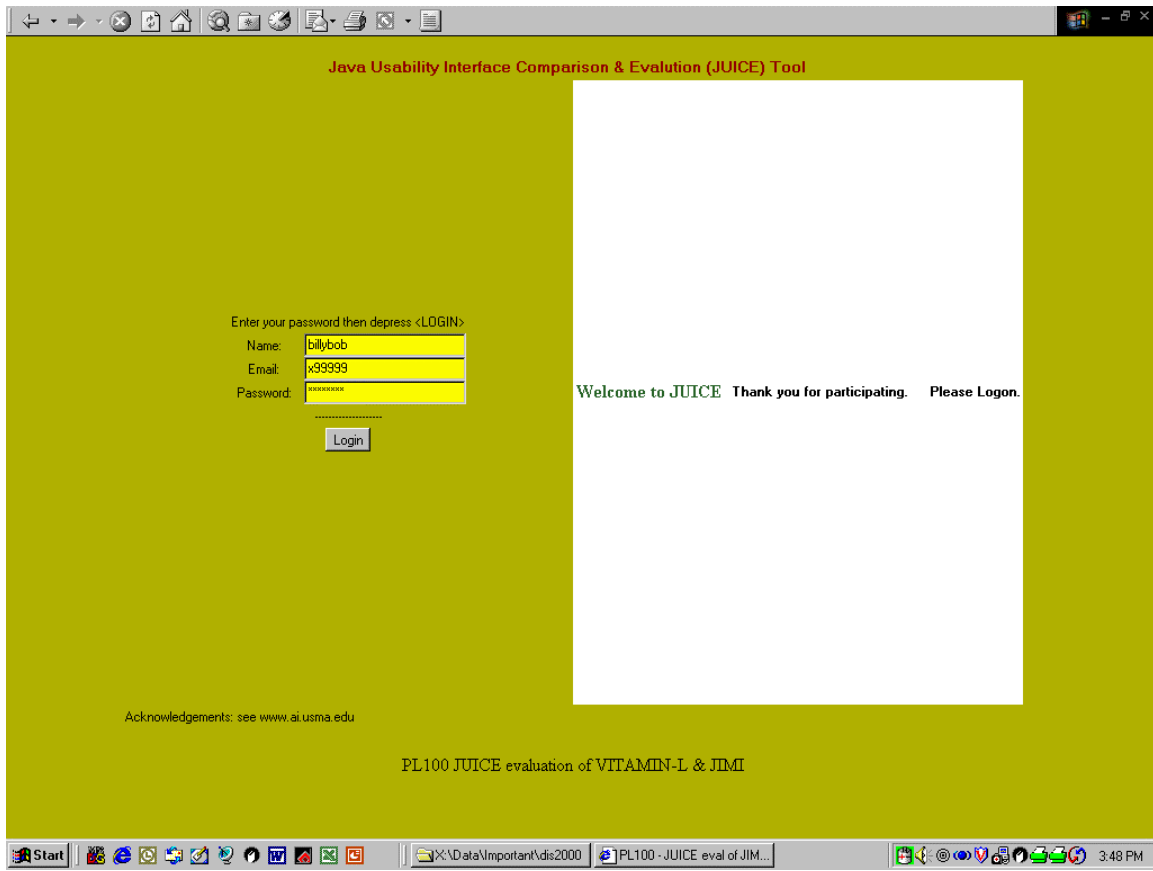
Figure 25 JUICE logon
