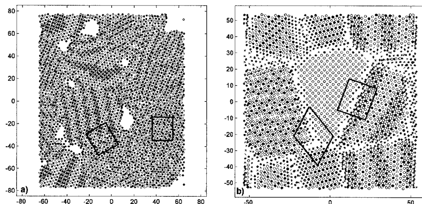
Figure 3: Slabs in NiAl CA (a) and Ni 3 Al SF (b) model samples after MD relaxation and MC sampling at 300K in order to account for Al segregation. Open circles represent Ni atoms and black circles represent Al atoms (in (b) 'o' and 'x' represent Ni and Al atoms, respectively, with the coordination number not equal to 12). The Al segregation at grain boundaries and at internal void surfaces is visible. The numbers on axes are in units of Å.
