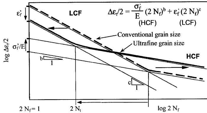
Figure 5. Schematic illustration of enhanced high-cycle fatigue (HCF) life and reduced low-cycle fatigue (LCF) life of UFG-materials due to increased fatigue strength coefficient \sigma_f' and reduced fatigue ductility coefficient \epsilon_f' , respectively. Note also the reduced transition fatigue life N_t . E : Young's modulus.
