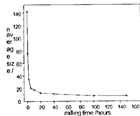
Figure 6. Grain size of WC versus milling time
