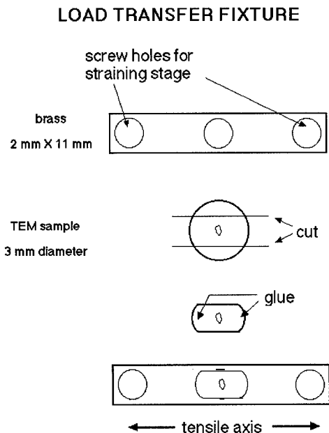
Figure 2. Fixture for supporting TEM samples during in situ deformation.
