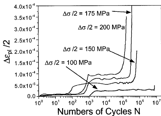
Figure 6: Cyclic deformation curves ( \Delta\epsilon_p/2 versus N ) of UFG-copper fatigued after slow stress build-up at constant stress amplitude \Delta\sigma/2 at 293 K. From [10].
