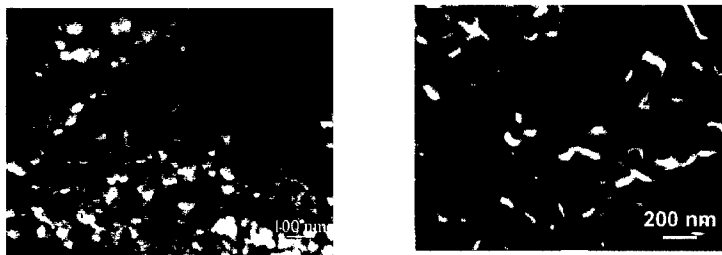
Fig. 5 Microstructure of (a) alumina-diamond and (b) alumina-niobium nanocomposites synthesized by high pressure sintering.
