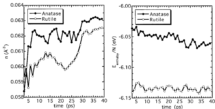
Figure 1. Time evolution of density and normalized enthalpy in the present simulations for rutile and anatase nanoparticles.
