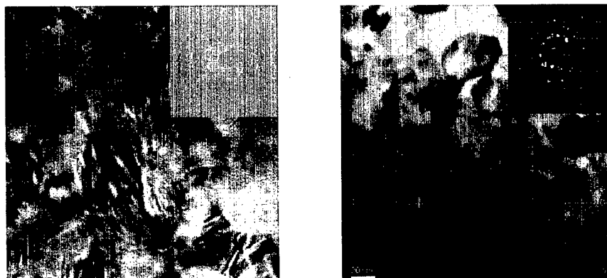
Figure 1.(a) and (b). Bright field images with its SAD patterns of the as received samples for ED Nickel (a) and IGC Nickel (b). The sizes of the SAD patterns are approximately 150 to 200 nm. In ED high strain is visible by the bowed Moiré fringes. IGC Ni shows much less strain with mostly distinct high angle grain boundaries.
