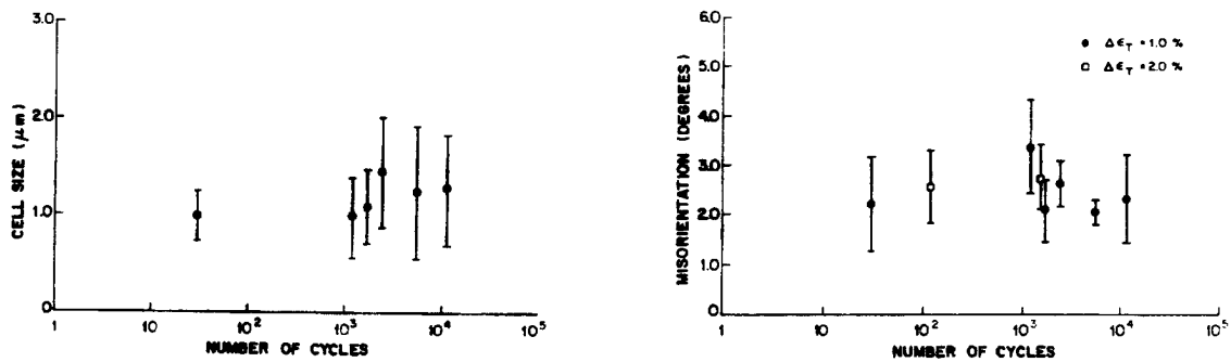
(a) Variation of cell size with cycles for \Delta\epsilon_T=1.0\% ; (b) Misorientation between cells for \Delta\epsilon_T=1.0\% , and 2.0\% .
