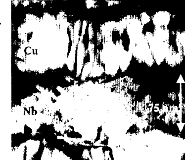
Fig. 3 TEM micrograph of a Cu-Nb multilayer annealed at 600 °C. Thermal strains ( \sim 0.5\% ) result in an array of dislocation loops in the Cu layer, while no significant plasticity is observed in Nb.
