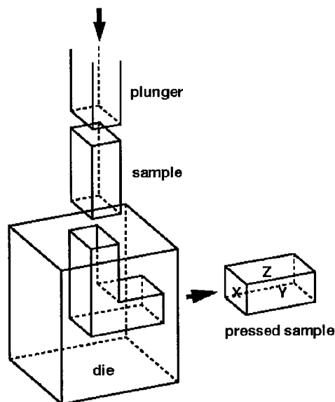
Figure 1. Schematic illustration of the principle of ECAP.
