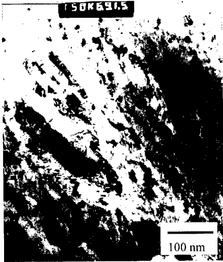
Fig. 6 Elongated grains, with smaller dimension, in Inconel 625 powder following cryomilling of 6 hours.
