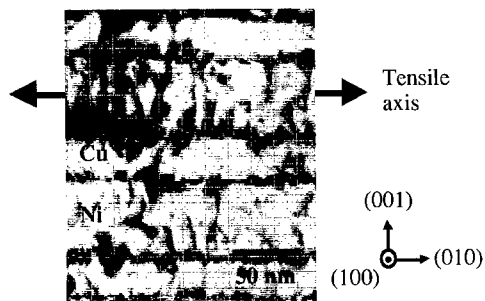
Figure 1. Cross-section TEM micrograph of a 35 nm Cu/55 nm Ni single crystal nanolaminate. Threading and Orowan type dislocation span both layer types.
