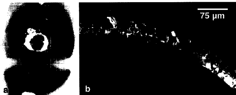
Figure 3. The optical microscope images of the (a) 1\ \text{mm} dia. \text{Be}_{1-x}\text{Cu}_x coated capsule tested to failure and (b) fracture cross-section at higher magnification.
