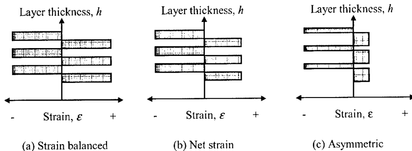
Figure 1. Types of multilayered structures grown. Range of layer parameters used ( 0\% < \epsilon < \pm 1.5\% , 17\text{nm} < \text{layer thickness} < 125\text{nm} ).
