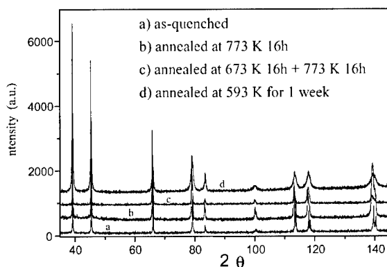
Fig.1 - X-ray diffraction patterns of selected Au 80 Fe 20 ribbons.
