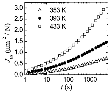
Figure 5. Temperature dependence of the anelastic creep compliance in Ni-MA. \sigma = 112 MPa
