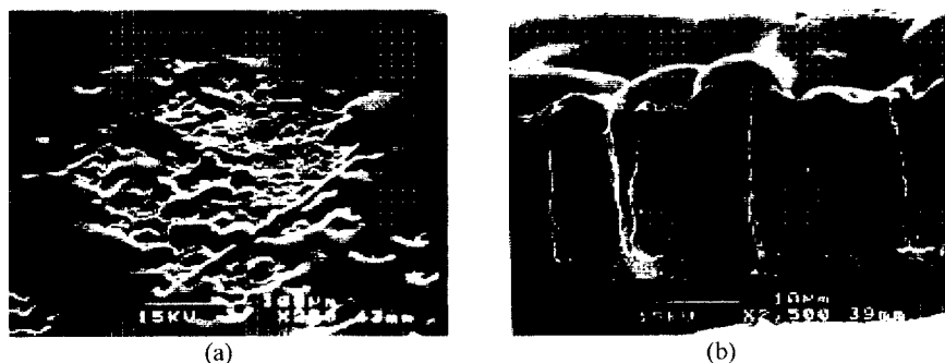
Figure 6. SEM micrographs showing (a) the nodular growth in an isolated area and (b) the brittle fracture associated with nodular growth in sample 3.
