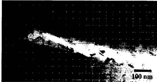
Figure 3. A crack formed during in situ straining as a result of localized plastic deformation in an epitaxial single crystal Cu/Ni nanolaminate. The crack is growing from right to left and was formed during two discrete events.
