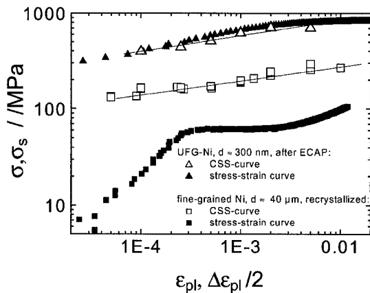
Figure 8. Cyclic and monotonic stress-strain curves of UFG-nickel (ca. 300 nm) at 293 K, comparison with data of recrystallized nickel of conventional grain size (40 μm). Courtesy of E. Thiele.
