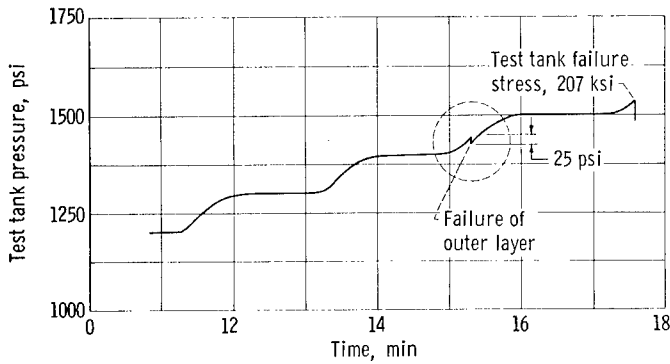
Figure 14. - Pressure as function of time plot for multilayer tank at -423^{\circ} F.
