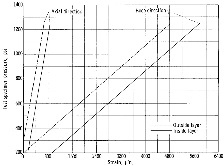
Figure 13. - Typical strain as function of pressure plot for multilayer tanks.
