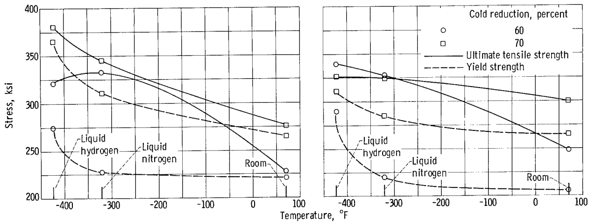
(a) Longitudinal direction. (b) Transverse direction. Figure 6. - Strength properties of 0.0055-inch-thick AISI 301 stainless steel as function of temperature.
