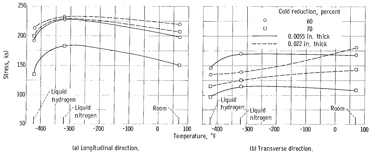
(a) Longitudinal direction. (b) Transverse direction. Figure 9. - Edge-notch strength properties of AISI 301 stainless steel as function of temperature.
