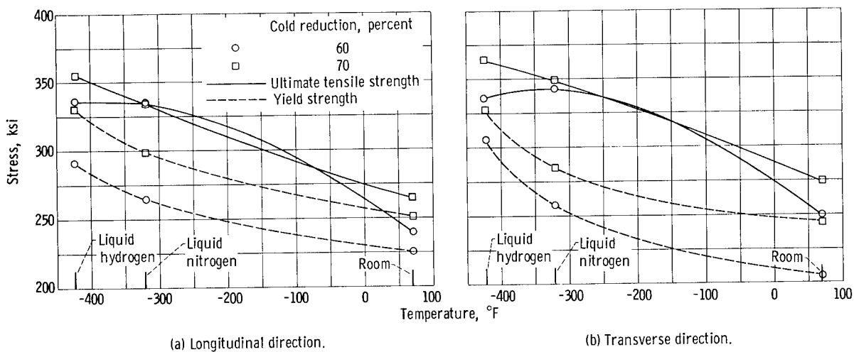
(a) Longitudinal direction. (b) Transverse direction. Figure 7. - Strength properties of 0.022-inch-thick AISI 301 stainless steel as function of temperature.
