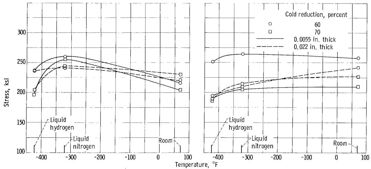
(a) Longitudinal direction. (b) Transverse direction. Figure 8. - Center-notch strength properties of AISI 301 stainless steel as function of temperature.
