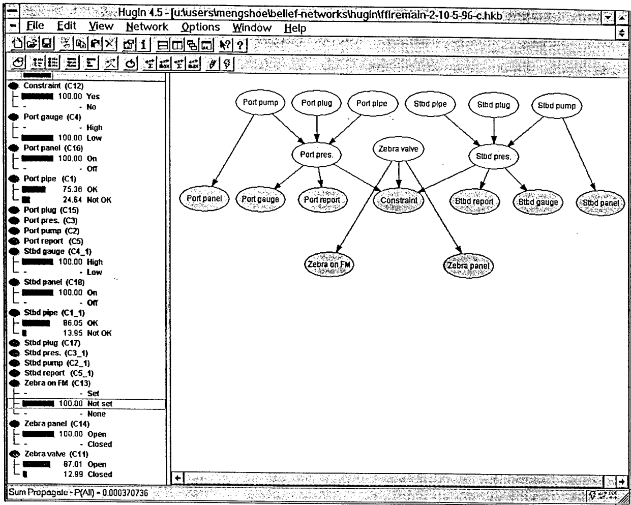
Figure 48. Belief network representing larger part of fire main system
