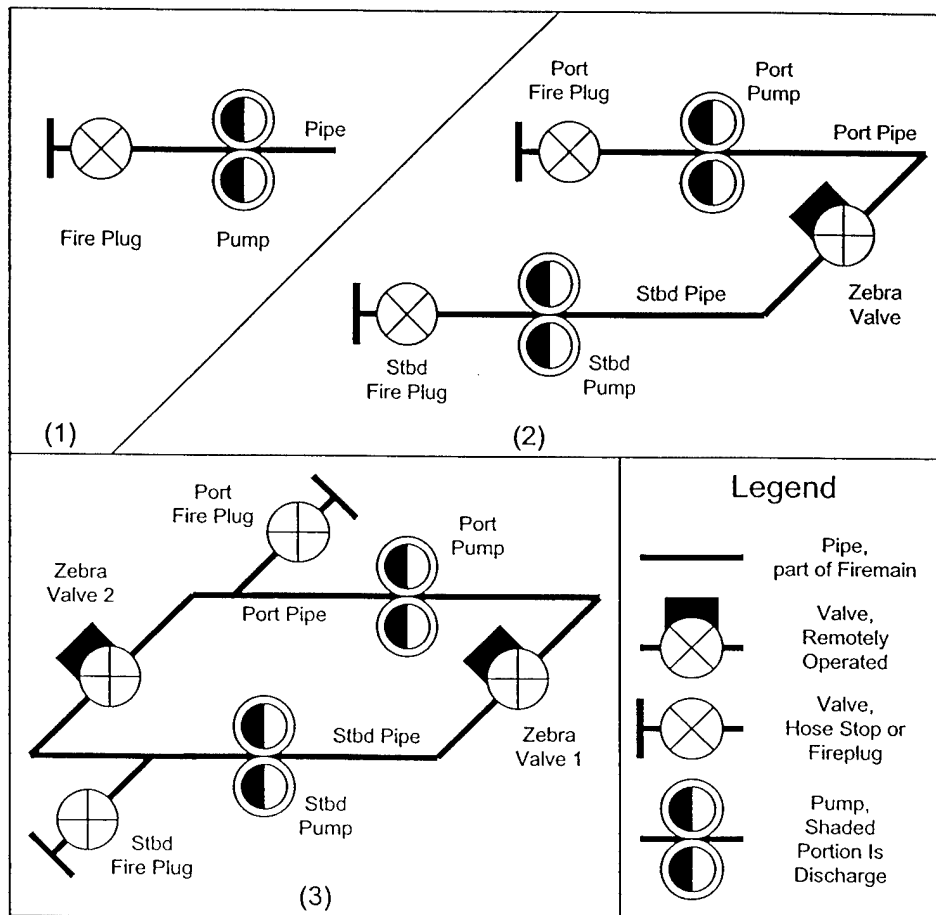
Figure 46. Parts of the fire main system
