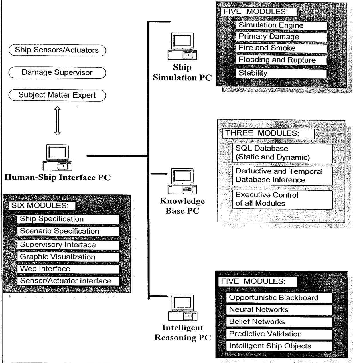
Figure 3. Module-Level View: Decomposition of the Automated Supervisory Control System into 19 independent modules
