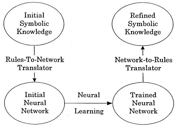
Figure 38. Rule refinement using Neural Networks
