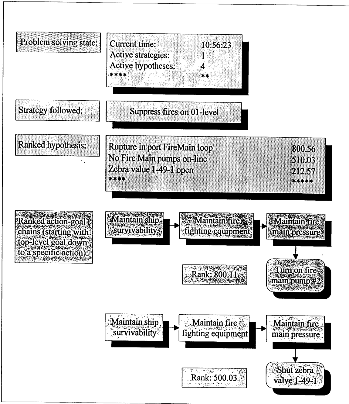
Figure 35. Blackboard items
