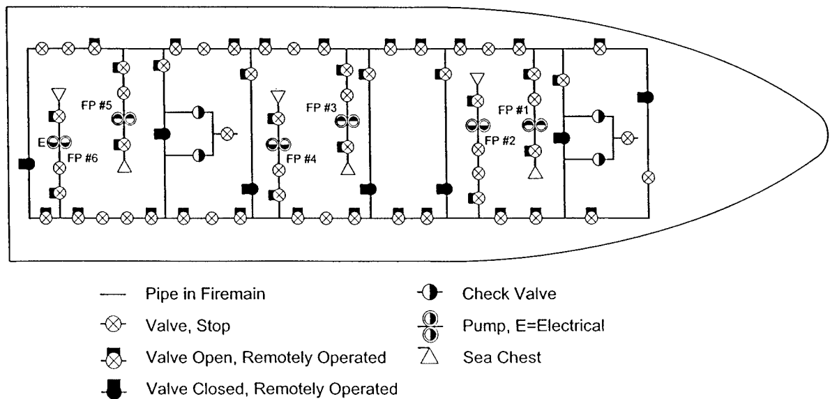
Figure 45. Fire main segregation
