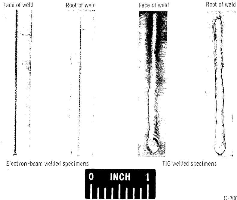
Figure 6. - Typical appearance of all electron-beam and gas tungsten-arc welded specimens.
