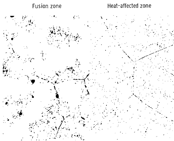
(a) As-welded and heat-treated 1 hour at 2500° F.
