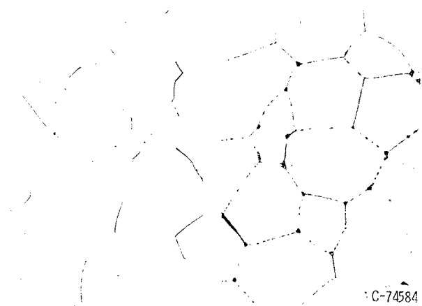
(e) Solution-treated and then aged 10 hours at 2000° F.
