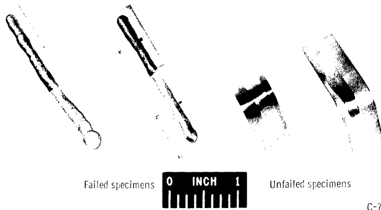
Figure 7. - Bend-tested specimens.
