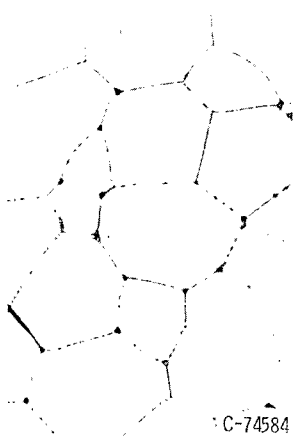
(f) Solution-treated, heat-treated, and then aged 10 hours at 2000° F.
