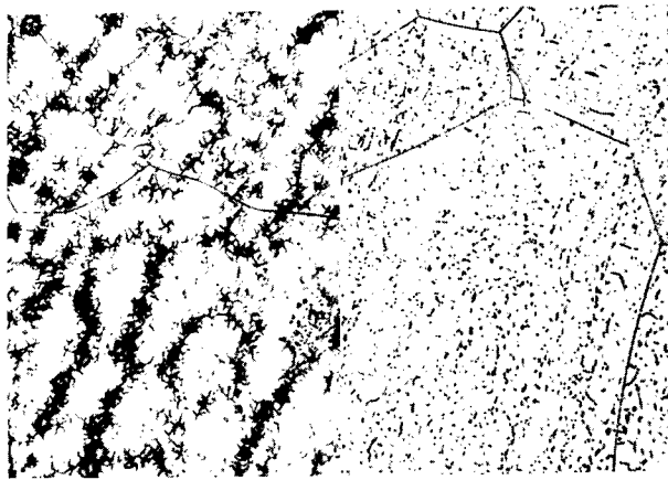
(a) Heat-treated 1 hour at 2500° F.
