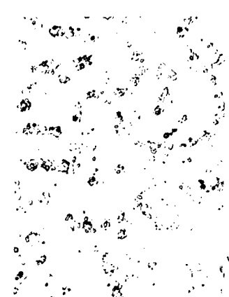
(c) As-welded and then aged 10 hours at 2000° F.
