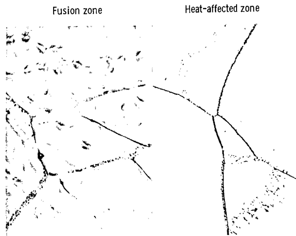
(a) Heat treated 1 hour at 2500° F.
