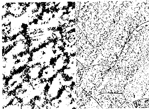
(c) Heat-treated and then aged 10 hours at 2000° F.
