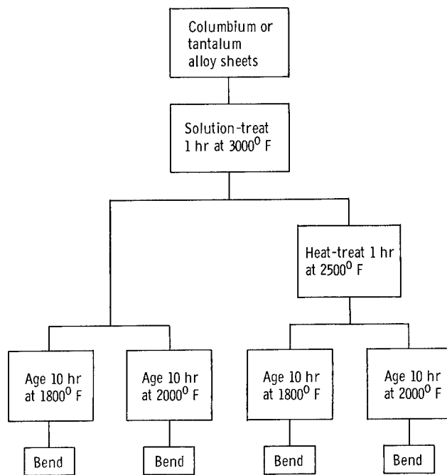
Figure 5. - Operations performed on nonwelded control specimens of FS-85, D-43, T-111, and T-222 alloys.
