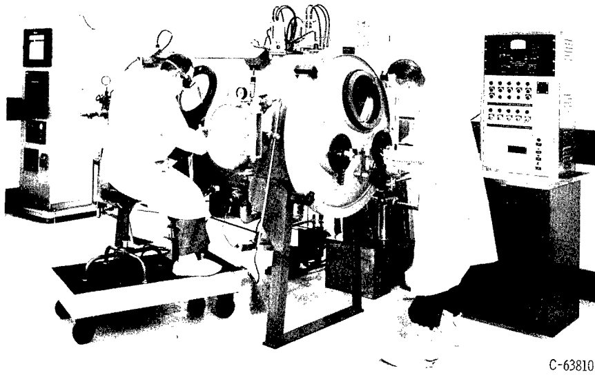
Figure 1. - Equipment used for gas tungsten-arc welding with clean laboratory conditions.
