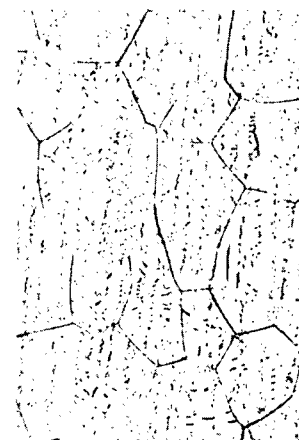
(c) Solution-treated and then aged 10 hours at 1800° F.
