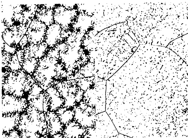
(b) Heat-treated and then aged 10 hours at 1800° F.
